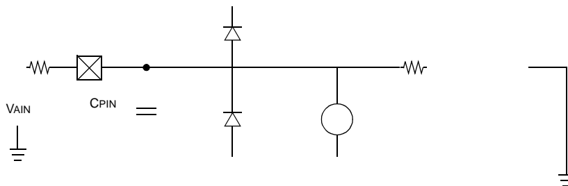
FIGURE 18-3: ANALOG INPUT MODEL
