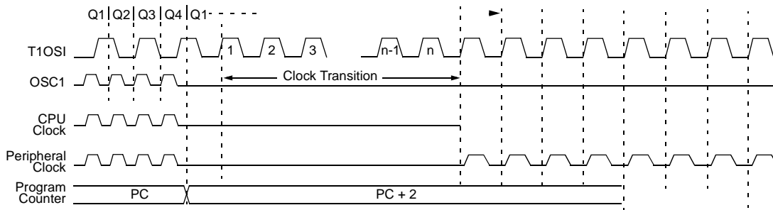
FIGURE 3-1: TRANSITION TIMING FOR ENTRY TO SEC_RUN MODE
