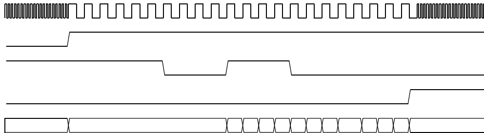
FIGURE 17-2: BRG OVERFLOW SEQUENCE
