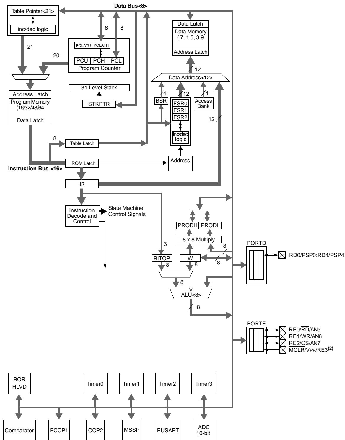
FIGURE 1-2: PIC18F4410/4510/4515/4610 (40/44-PIN) BLOCK DIAGRAM
