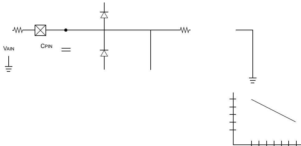
FIGURE 19-2: ANALOG INPUT MODEL
