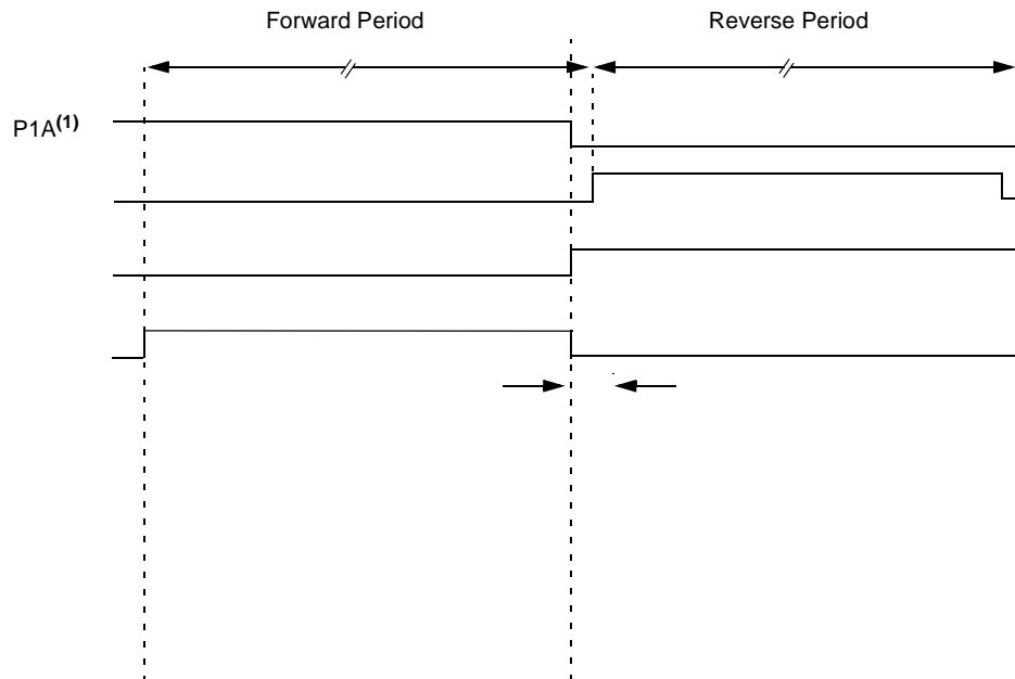
FIGURE 16-9: PWM DIRECTION CHANGE AT NEAR 100% DUTY CYCLE
