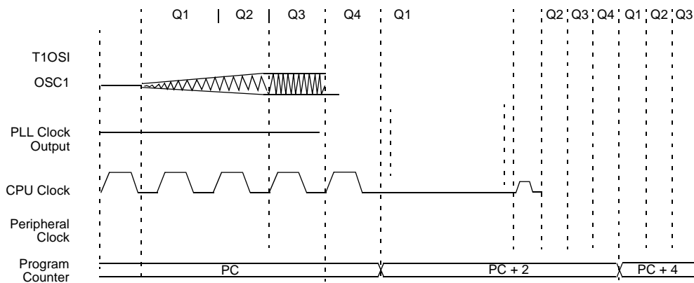
FIGURE 3-2: TRANSITION TIMING FROM SEC_RUN MODE TO PRI_RUN MODE (HSPLL)
