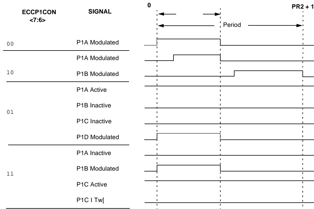
FIGURE 16-2: PWM OUTPUT RELATIONSHIPS (ACTIVE-HIGH STATE)
