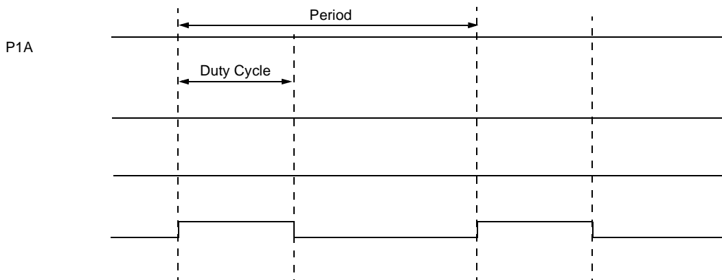
FIGURE 16-6: FULL-BRIDGE PWM OUTPUT
