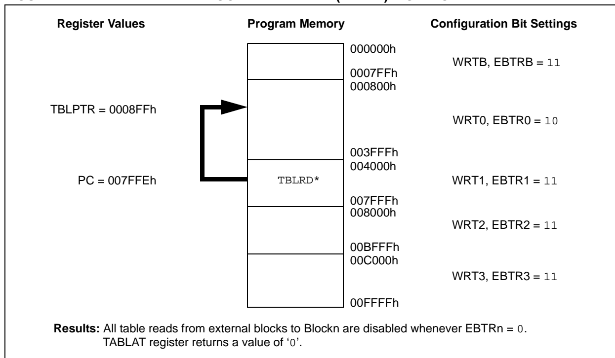
FIGURE 24-7: EXTERNAL BLOCK TABLE READ (EBTRn) DISALLOWED
