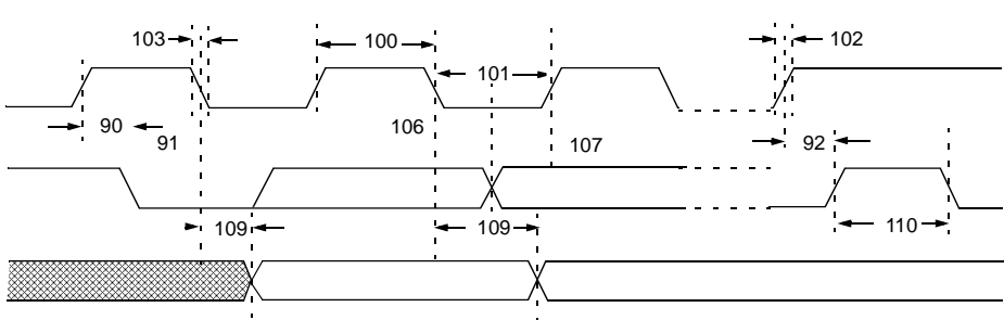
FIGURE 27-19: MASTER SSP I 2 C™ BUS DATA TIMING
