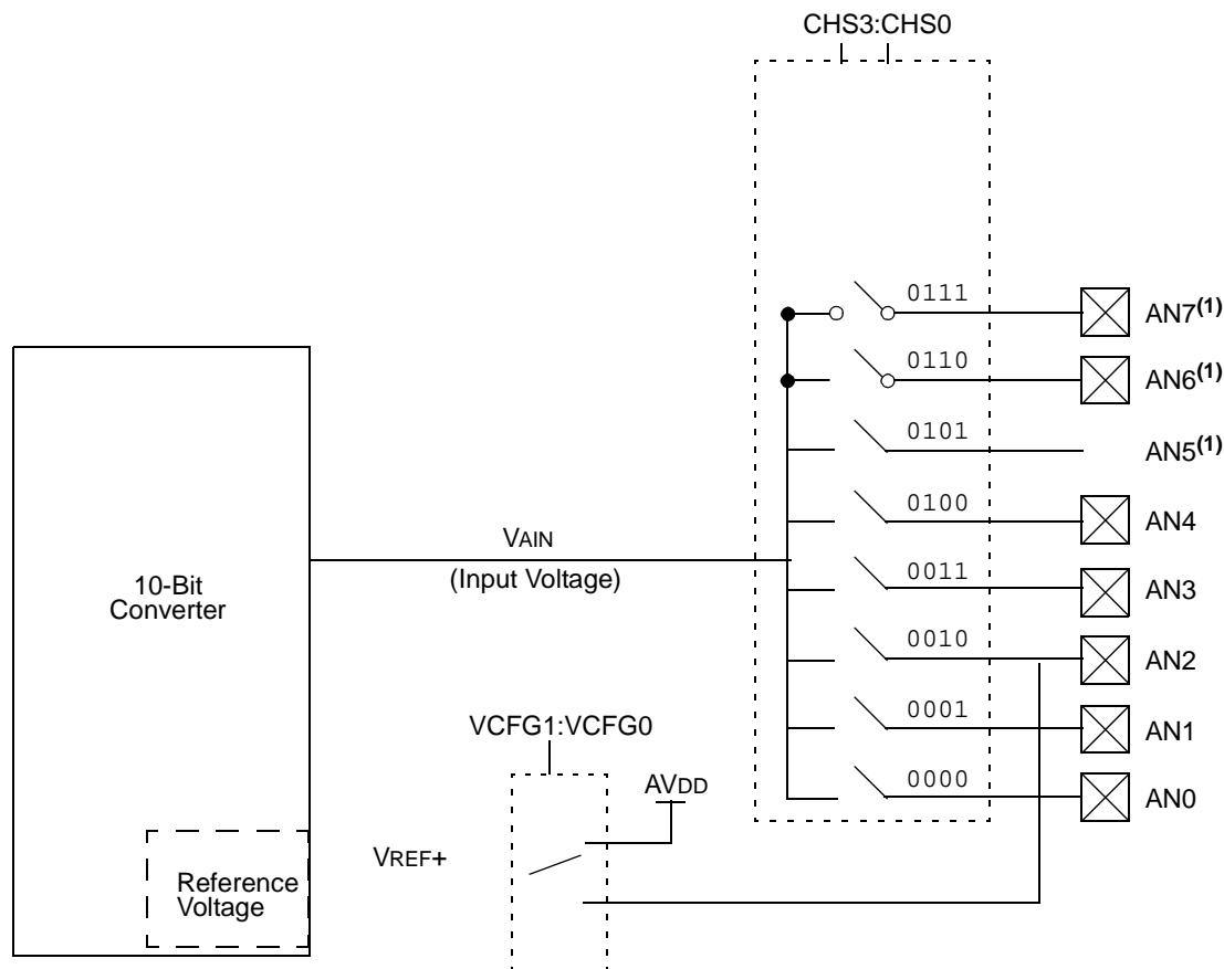
FIGURE 19-1: A/D BLOCK DIAGRAM
