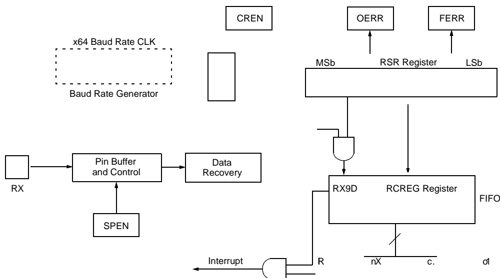
FIGURE 18-6: EUSART RECEIVE BLOCK DIAGRAM
