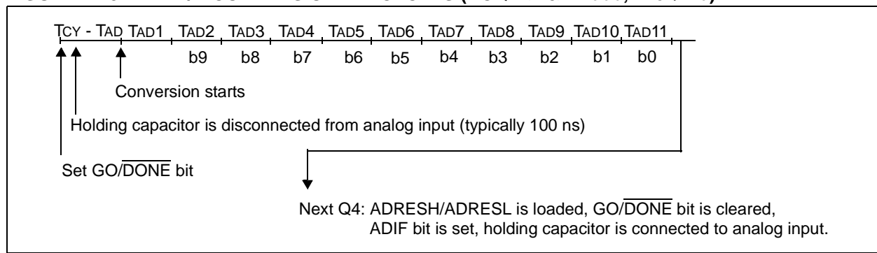
FIGURE 12-3: A/D CONVERSION TAD CYCLES ( \text{ACQT}<2:0> = 000 , \text{TACQ} = 0 )
