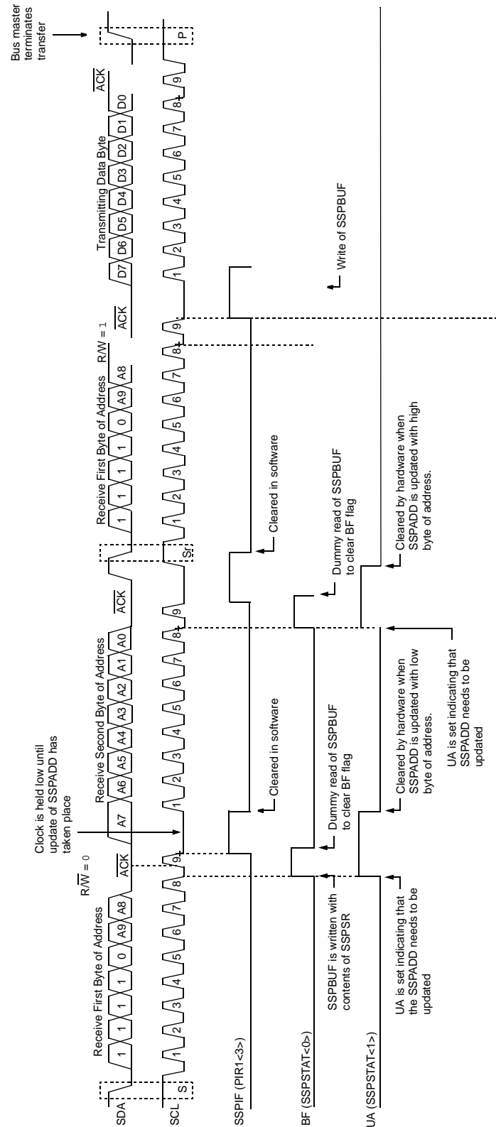
FIGURE 10-11: I 2 C™ SLAVE MODE TIMING (TRANSMISSION, 10-BIT ADDRESS)
