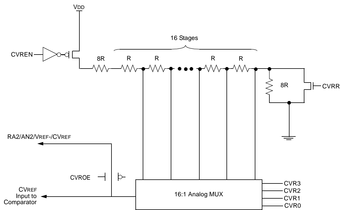
FIGURE 14-1: COMPARATOR VOLTAGE REFERENCE BLOCK DIAGRAM
