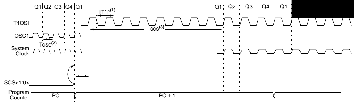
FIGURE 4-8: TIMING DIAGRAM FOR SWITCHING TO SEC_RUN MODE
