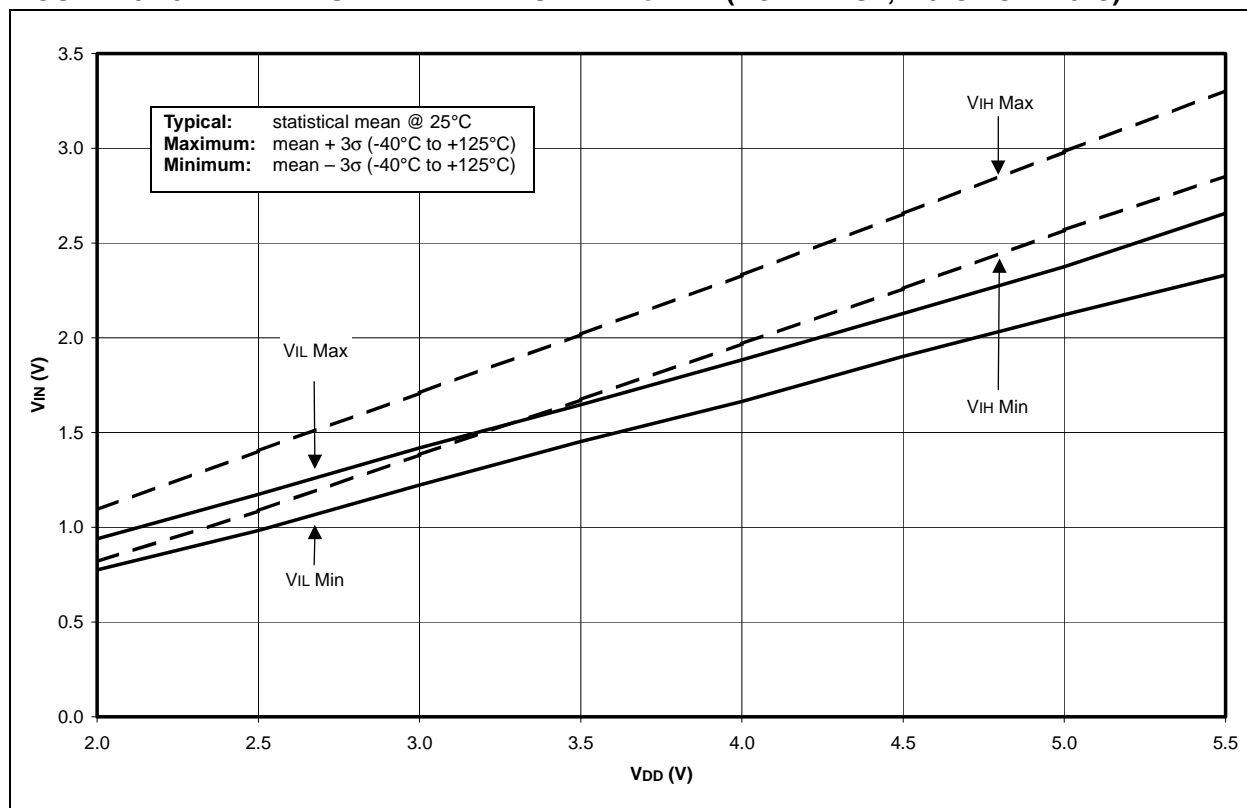
FIGURE 19-25: MINIMUM AND MAXIMUM V_{IH} vs. V_{DD} ( I^2C^TM INPUT, -40^{\circ}C TO +125^{\circ}C )
