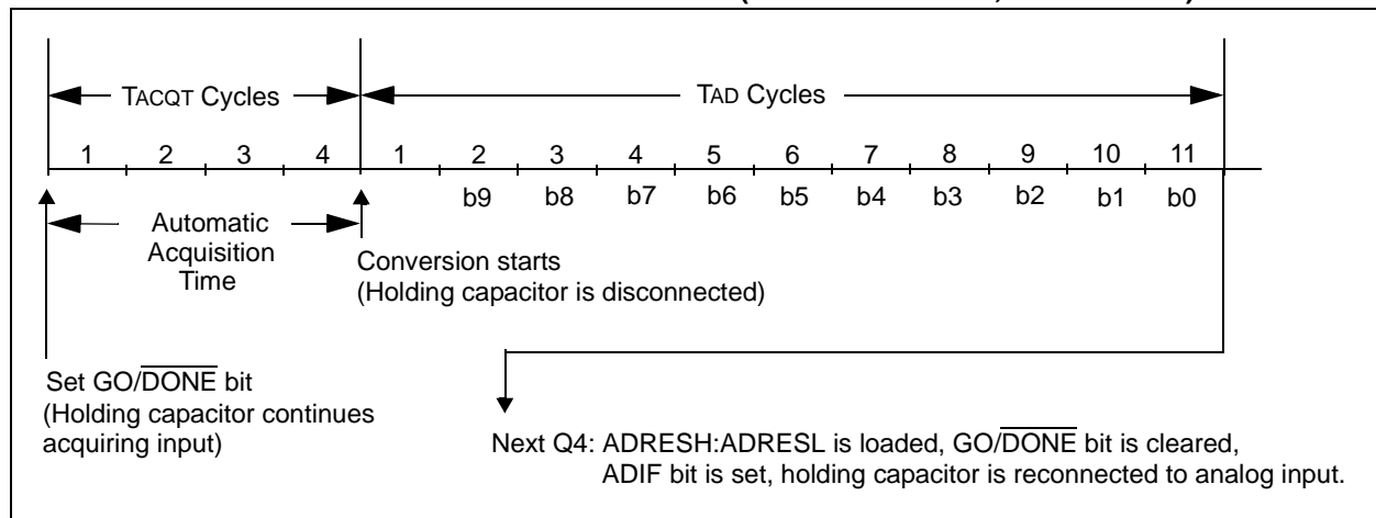
FIGURE 12-4: A/D CONVERSION TAD CYCLES ( \text{ACQT}<2:0> = 010 , \text{TACQ} = 4 \text{ TAD} )
