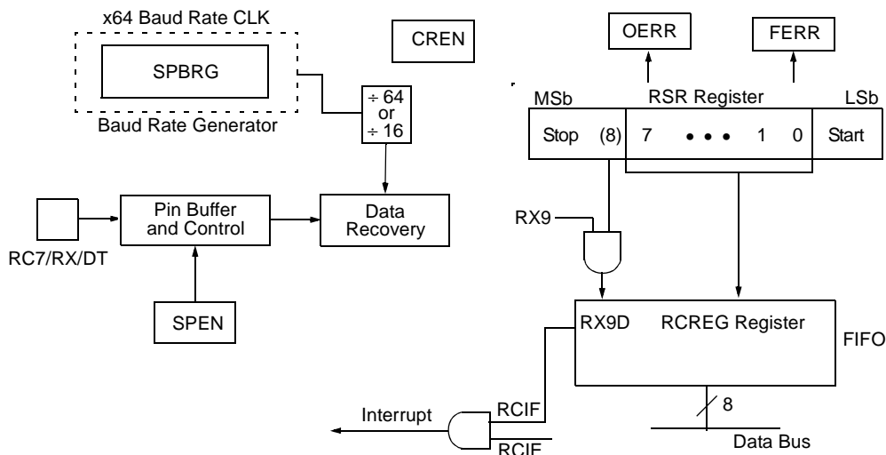
FIGURE 11-4: AUSART RECEIVE BLOCK DIAGRAM
