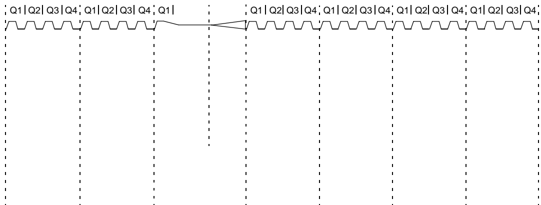
FIGURE 15-16: WAKE-UP FROM SLEEP THROUGH INTERRUPT
