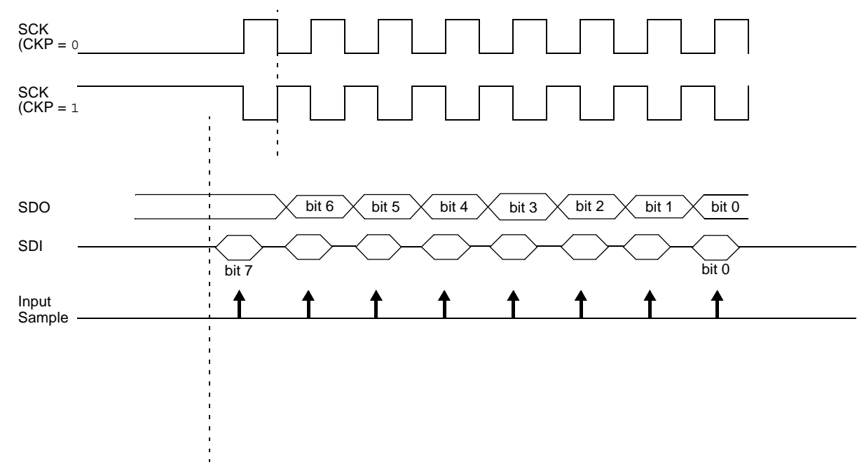
FIGURE 10-6: SPI™ MODE WAVEFORM (SLAVE MODE WITH CKE = 1)
