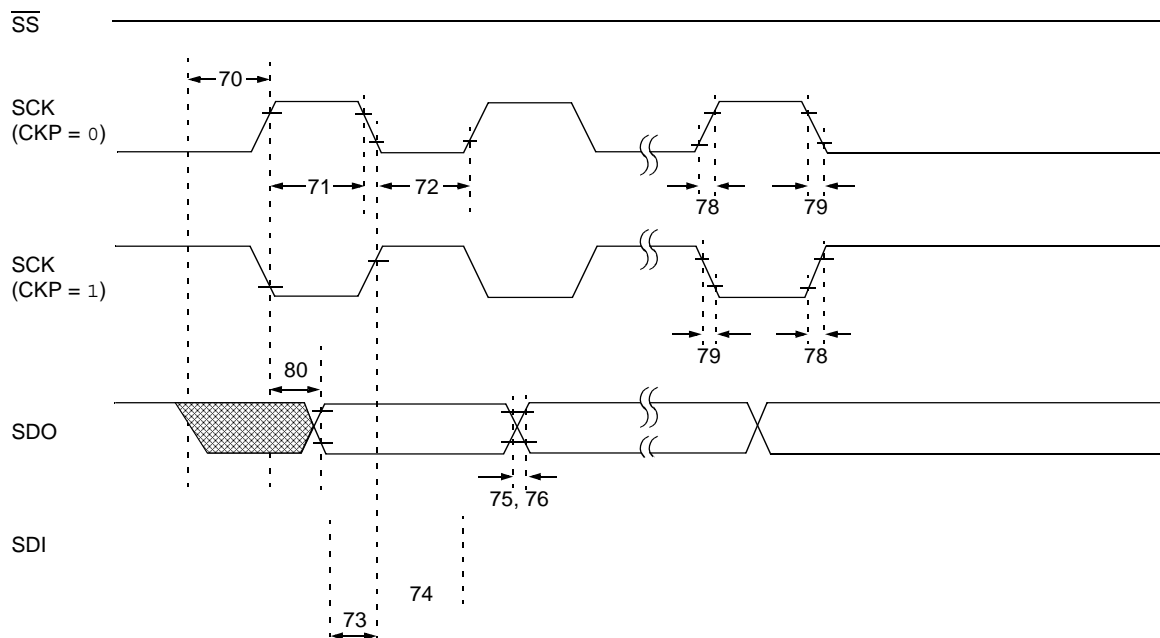
FIGURE 18-12: SPI™ MASTER MODE TIMING (CKE = 0, SMP = 0)
