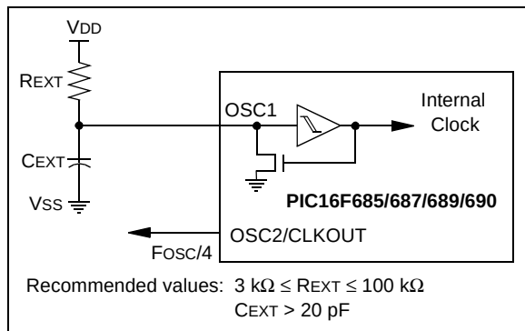
FIGURE 3-5: RC MODE
