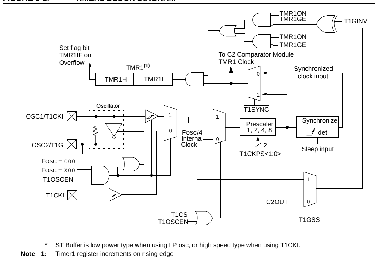
FIGURE 6-1: TIMER1 BLOCK DIAGRAM
