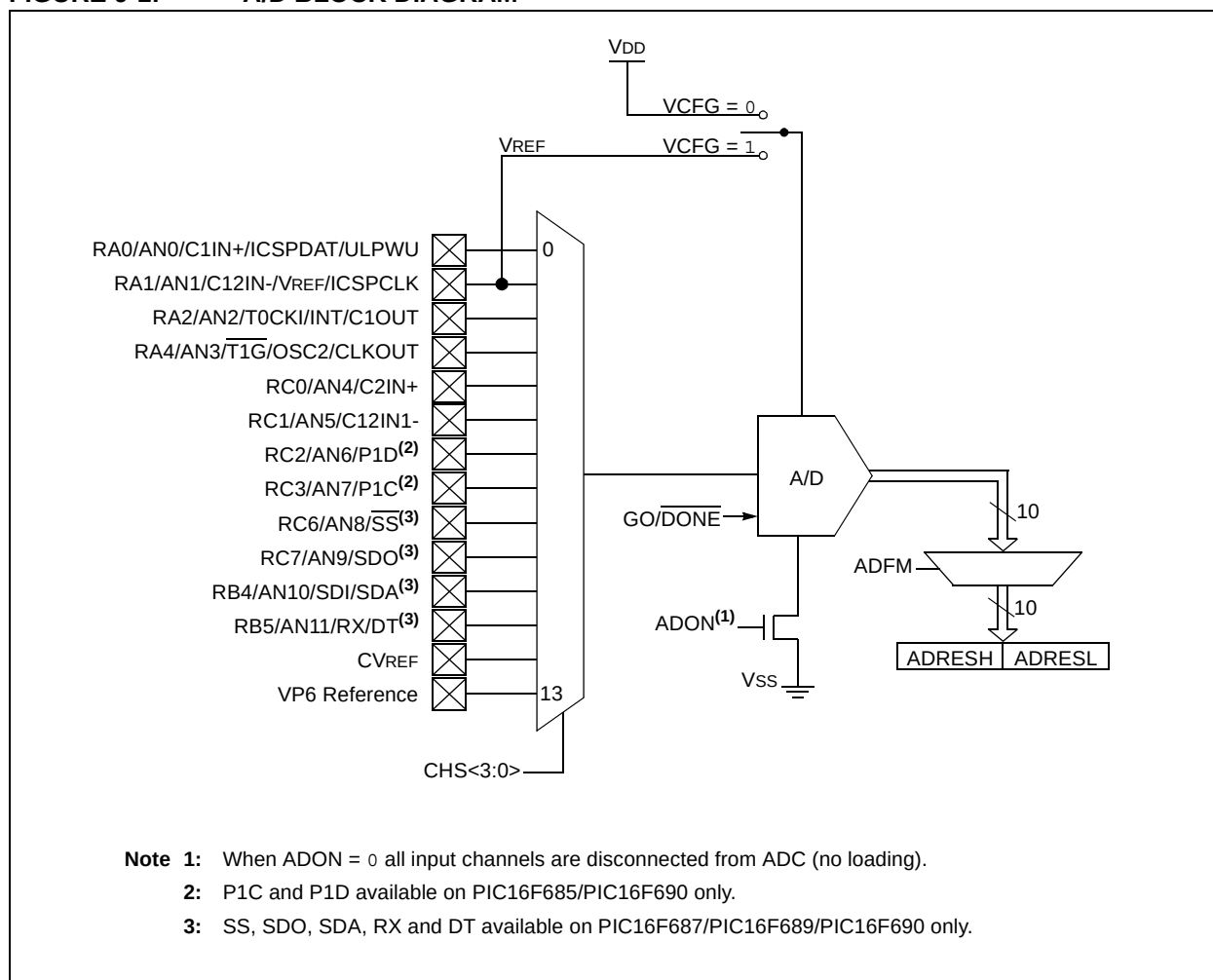
FIGURE 9-1: A/D BLOCK DIAGRAM
