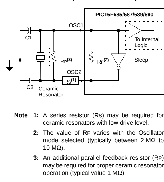
FIGURE 3-4: CERAMIC RESONATOR OPERATION (XT OR HS MODE)
