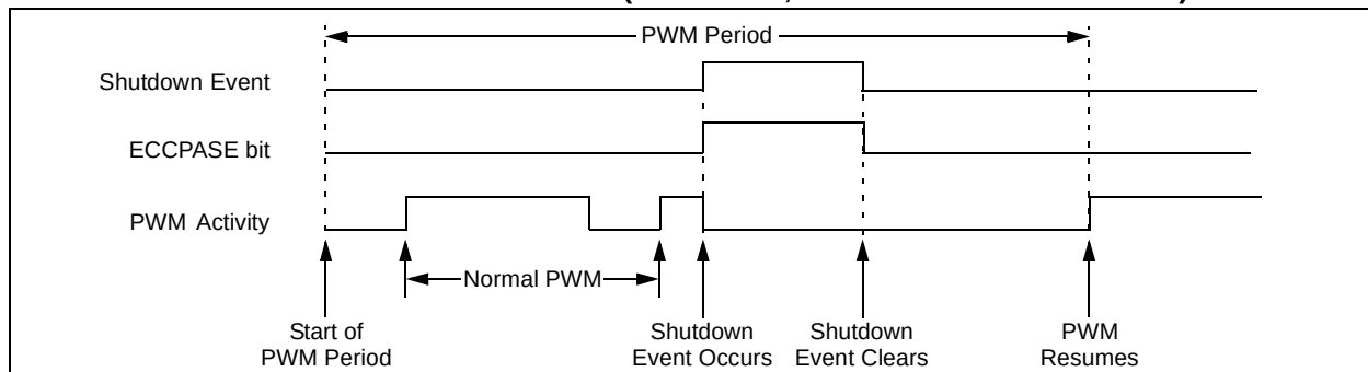
FIGURE 11-14: PWM AUTO-SHUTDOWN (PRSEN = 1, AUTO-RESTART ENABLED)
