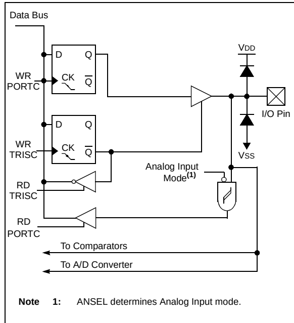
FIGURE 4-11: BLOCK DIAGRAM OF RC0 AND RC1
