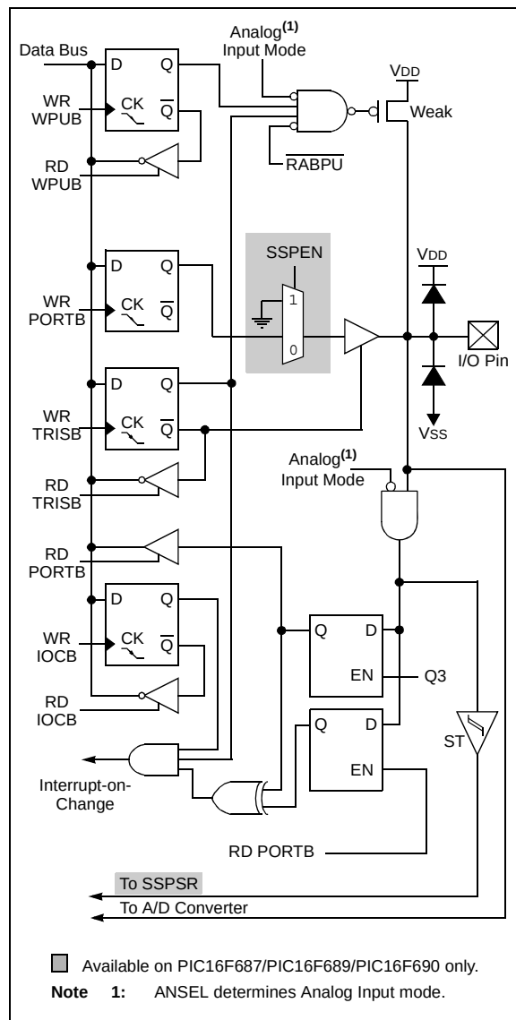
FIGURE 4-7: BLOCK DIAGRAM OF RB4
