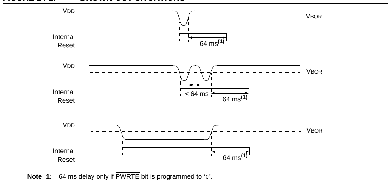
FIGURE 14-2: BROWN-OUT SITUATIONS
