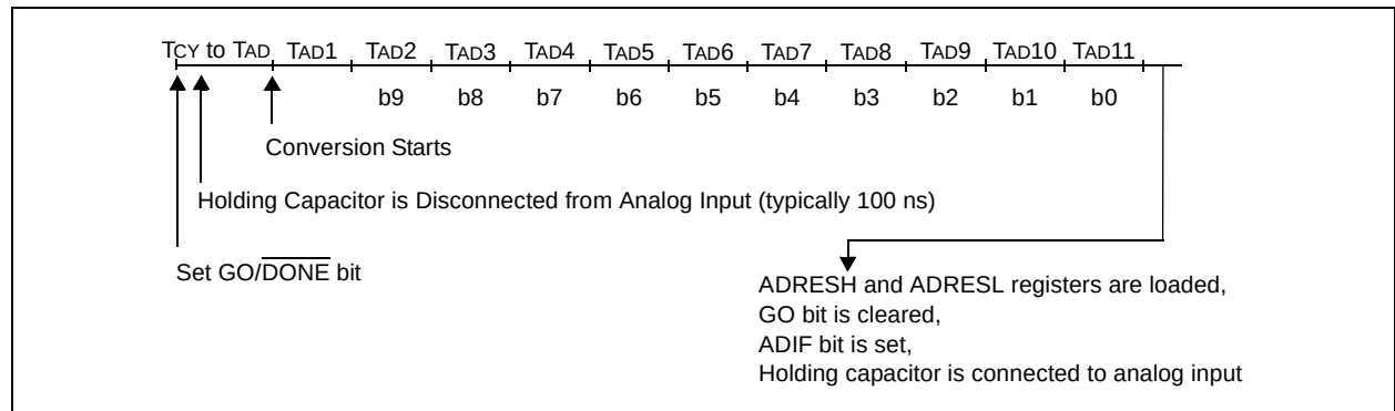
FIGURE 9-2: A/D CONVERSION TAD CYCLES
