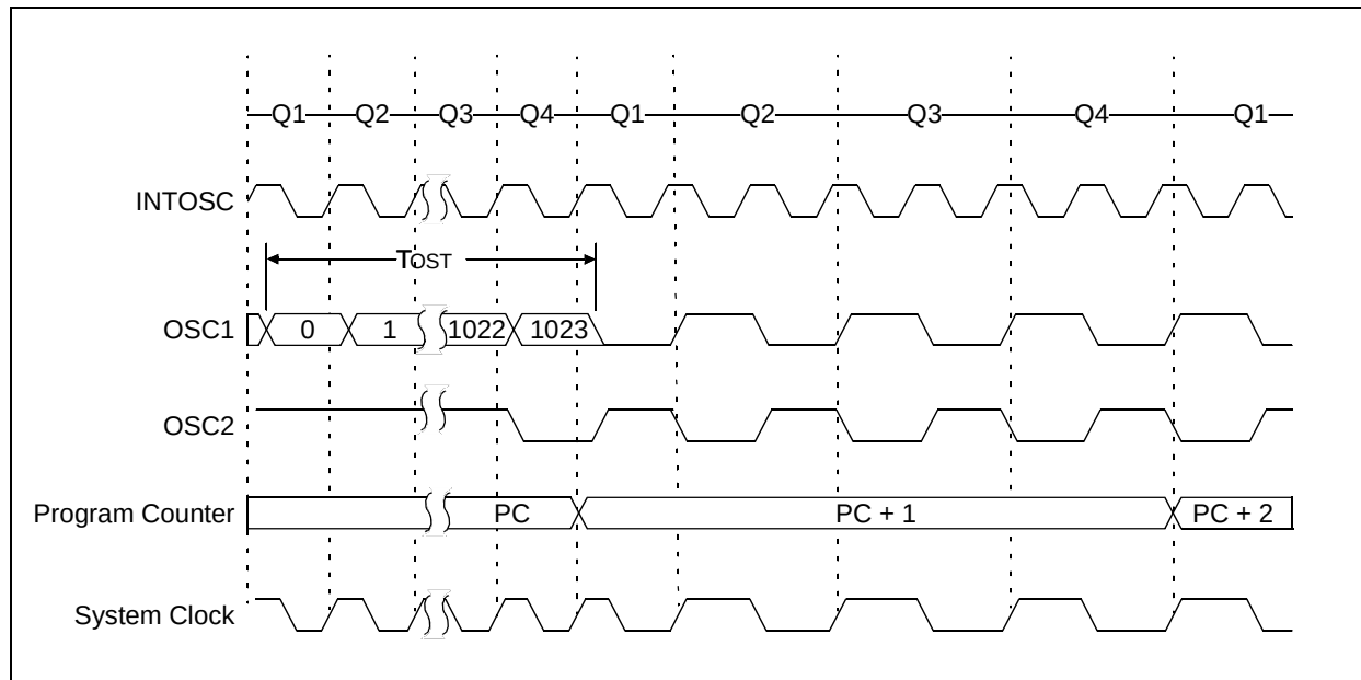
FIGURE 3-7: TWO-SPEED START-UP
