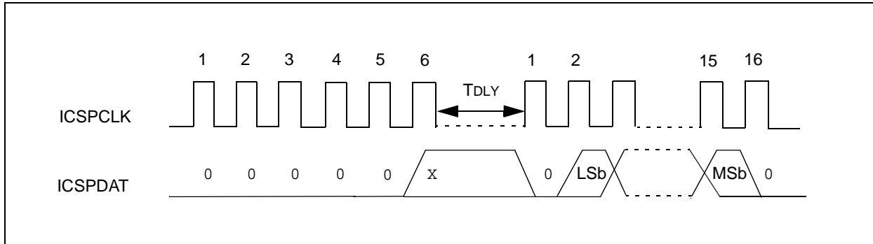
FIGURE 4-1: LOAD CONFIGURATION
