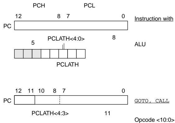
FIGURE 4-17: LOADING OF PC IN DIFFERENT SITUATIONS
