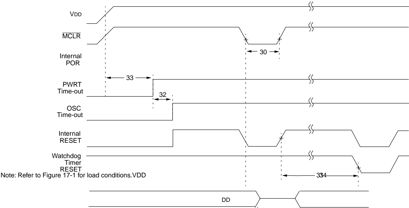
FIGURE 17-4: RESET, WATCHDOG TIMER, OSCILLATOR START-UP TIMER AND POWER-UP TIMER TIMING
