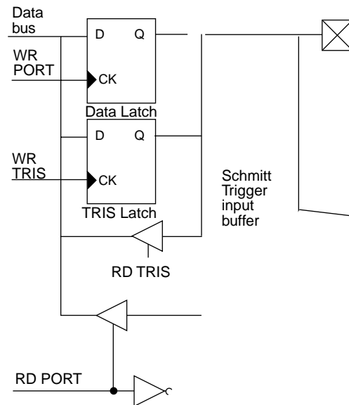
FIGURE 5-8: PORTE BLOCK DIAGRAM (IN I/O PORT MODE)
