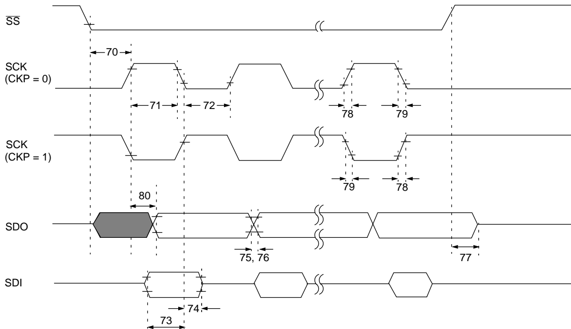
FIGURE 17-8: SPI MODE TIMING
