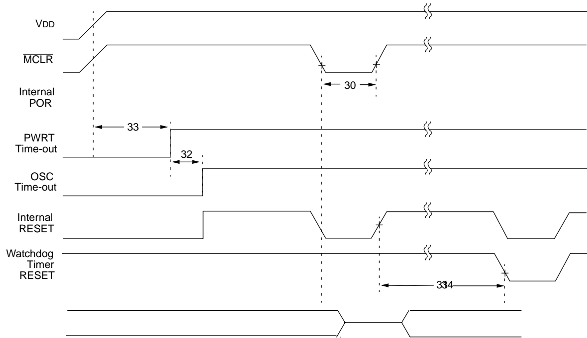
FIGURE 19-4: RESET, WATCHDOG TIMER, OSCILLATOR START-UP TIMER AND POWER-UP TIMER TIMING
