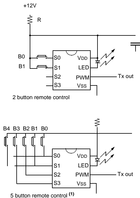
FIGURE 2-1: TYPICAL CIRCUITS
