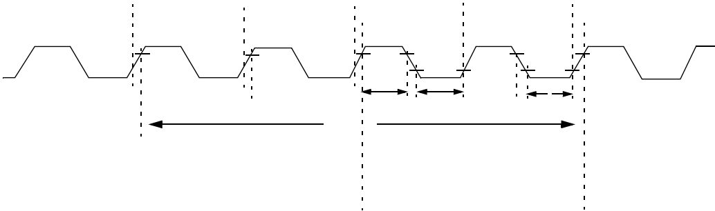
FIGURE 24-4: EXTERNAL CLOCK TIMING
