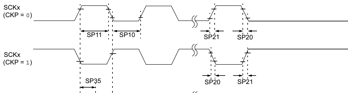
FIGURE 24-17: SPI MODULE MASTER MODE (CKE = 0) TIMING CHARACTERISTICS
