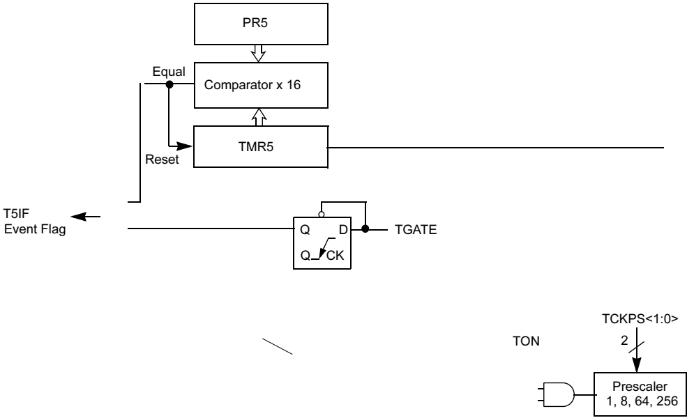
FIGURE 11-3: 16-BIT TIMER5 BLOCK DIAGRAM (TYPE C TIMER)
