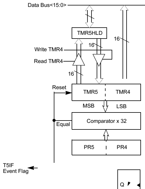
FIGURE 11-1: 32-BIT TIMER4/5 BLOCK DIAGRAM
