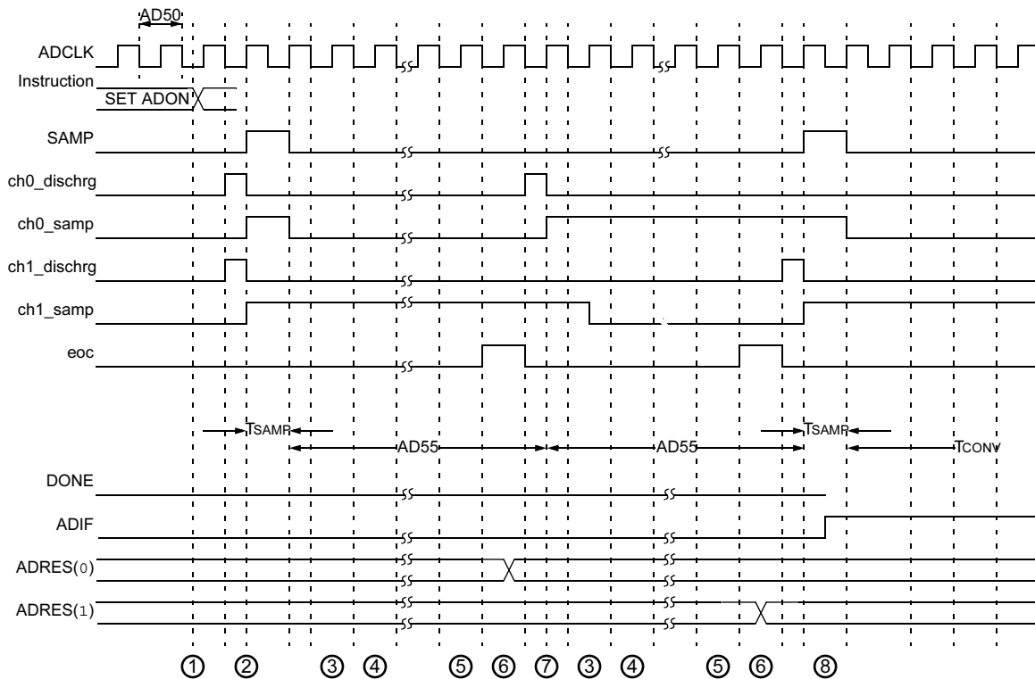
FIGURE 24-27: 10-BIT HIGH-SPEED A/D CONVERSION TIMING CHARACTERISTICS (CHPS = 01, SIMSAM = 0, ASAM = 1, SSRC = 111, SAMC = 00001)
