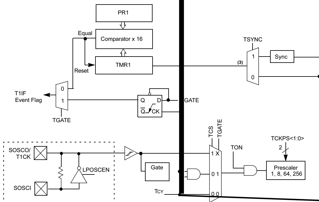
FIGURE 9-1: 16-BIT TIMER1 MODULE BLOCK DIAGRAM (TYPE A TIMER)
