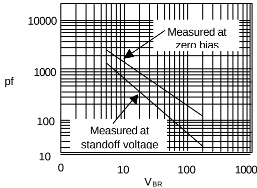
Figure 3 - Typical Capacitance
