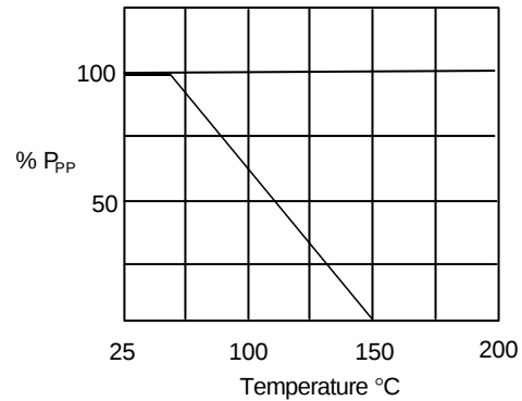
Figure 4 - Derating Curve
