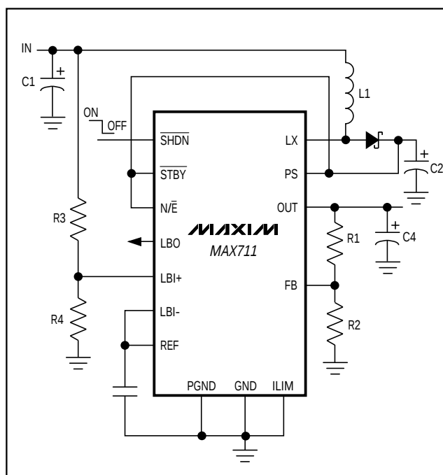
Figure 3. MAX711 Adjustable Output Voltage
