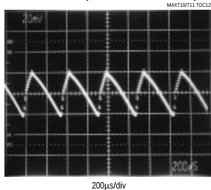
OUTPUT RIPPLE (HIGH-EFFICIENCY MODE)
