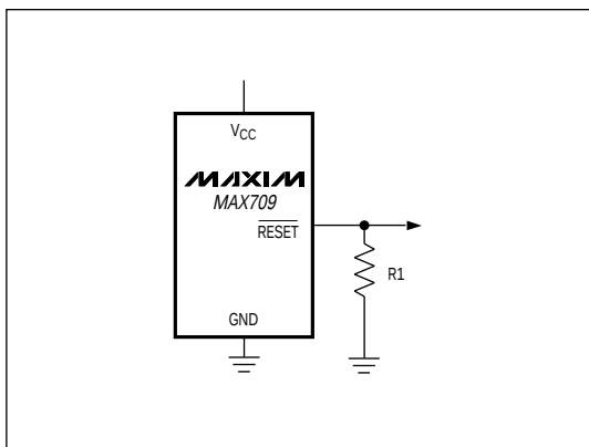
Figure 2. \overline{\text{RESET}} Valid to V_{CC} = Ground Circuit
