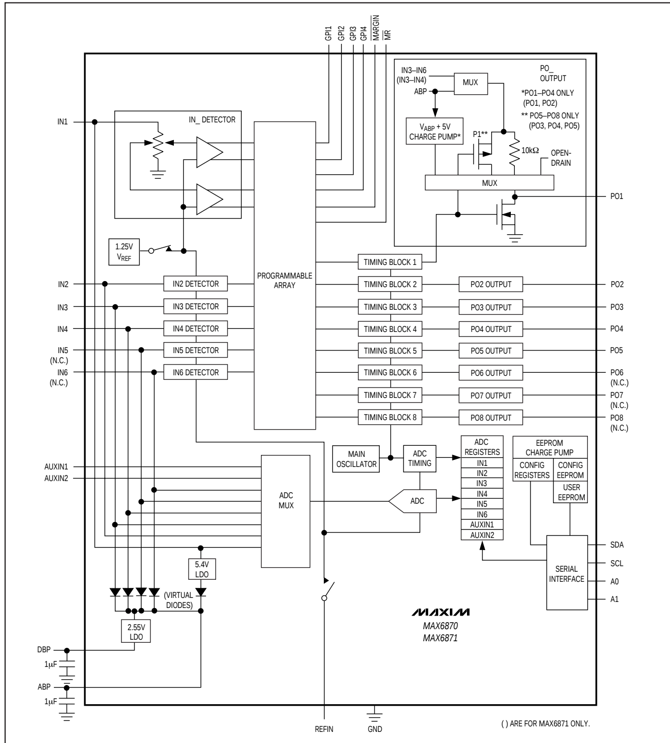
Functional Diagram
