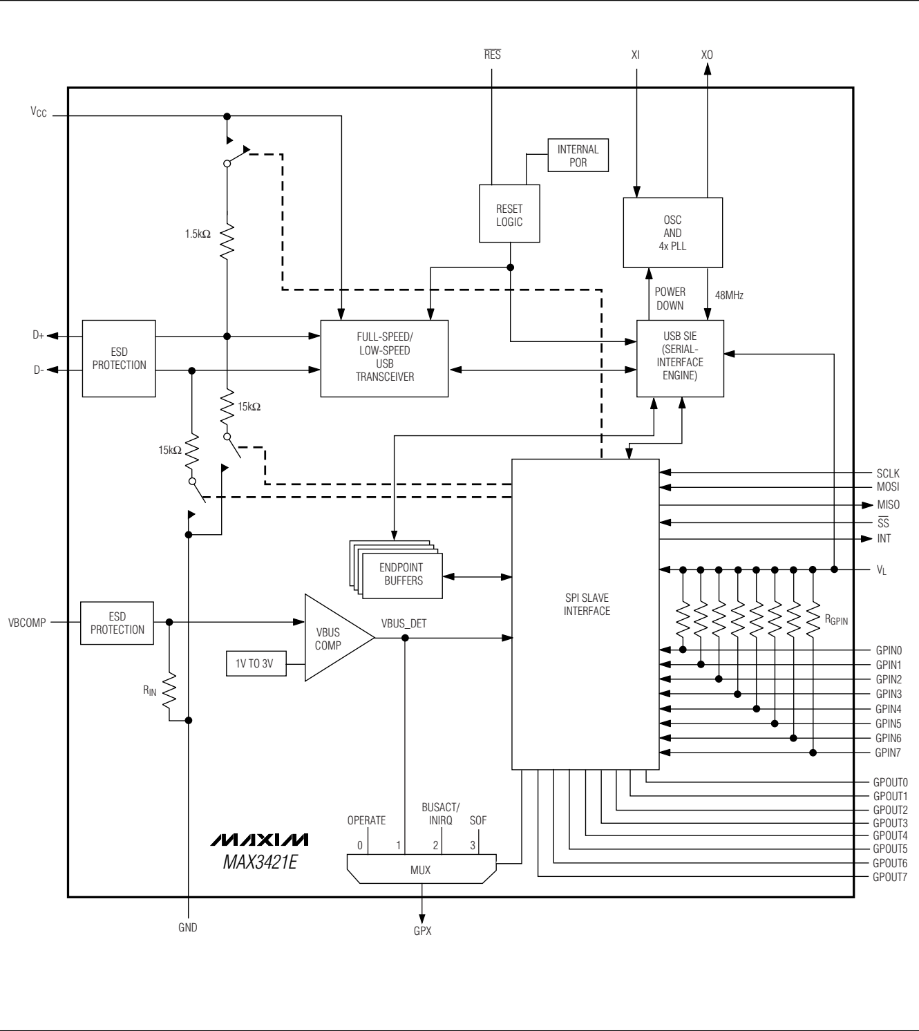
Functional Diagram
