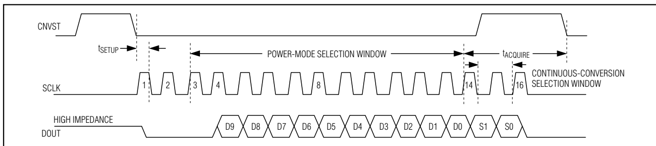
Figure 5. Interface-Timing Sequence
