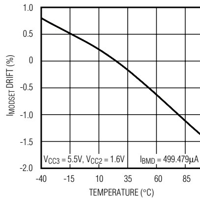
I_{MODSET} DRIFT vs. TEMPERATURE
