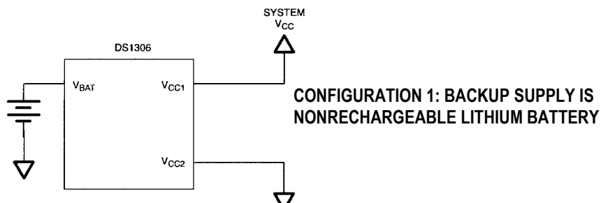
Figure 4. POWER SUPPLY CONFIGURATIONS
