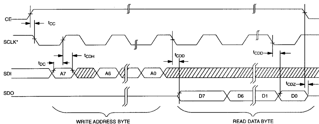
Figure 12. TIMING DIAGRAM: SPI READ DATA TRANSFER
