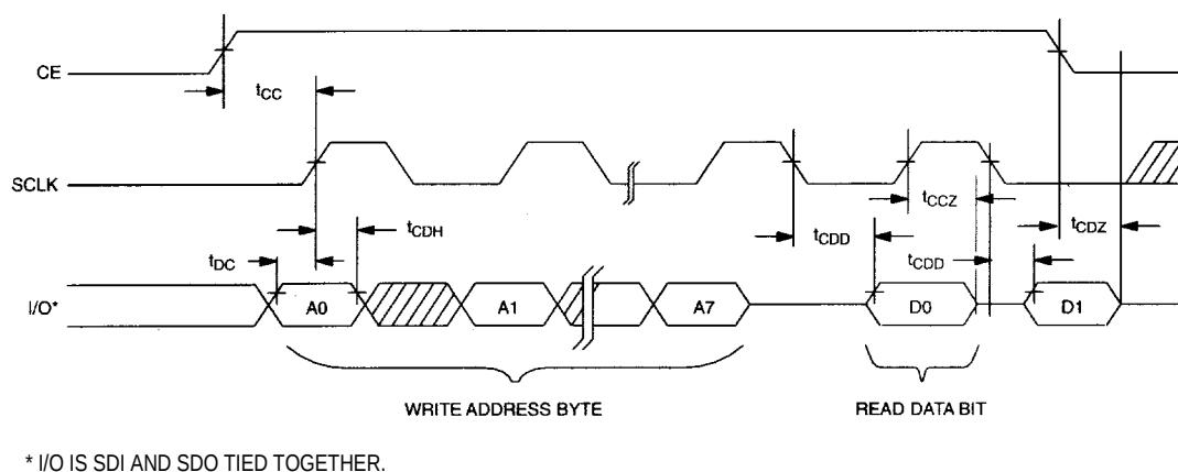
Figure 10. TIMING DIAGRAM: 3-WIRE READ DATA TRANSFER
