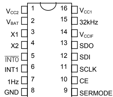
DIP (300 mils)
