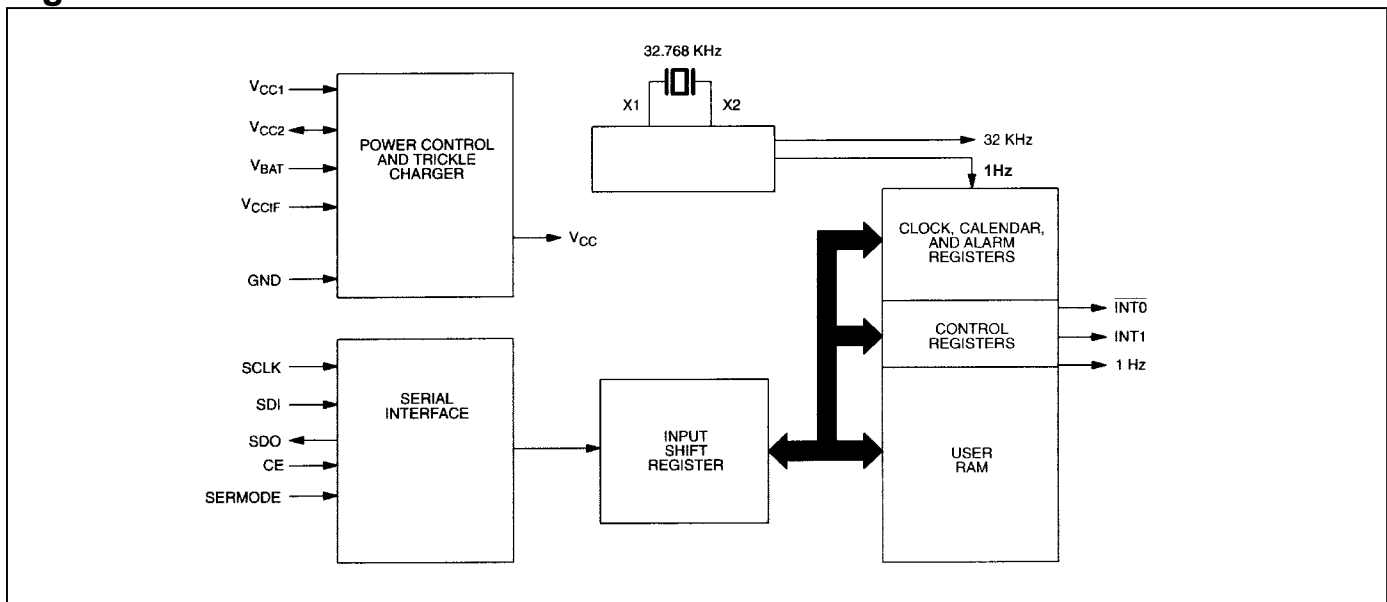
Figure 1. BLOCK DIAGRAM
