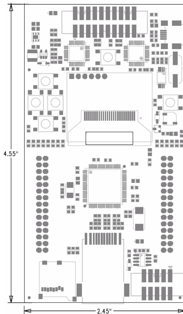
Figure B-2. LM3S8962 Evaluation Board Dimensions
