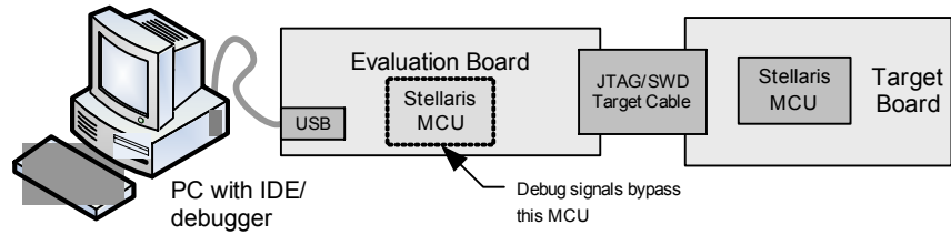
Figure 2-1. ICD Interface Mode
