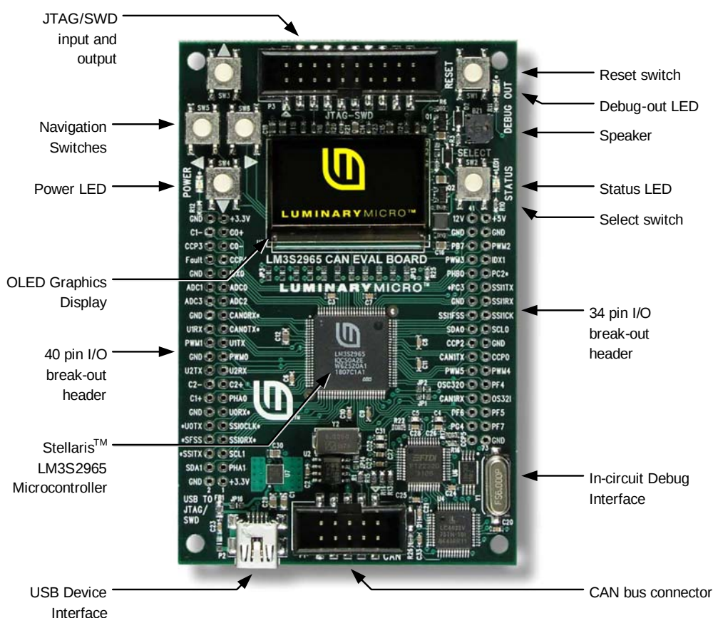
Figure 1-1. Stellaris LM3S2965 Evaluation Board Layout
