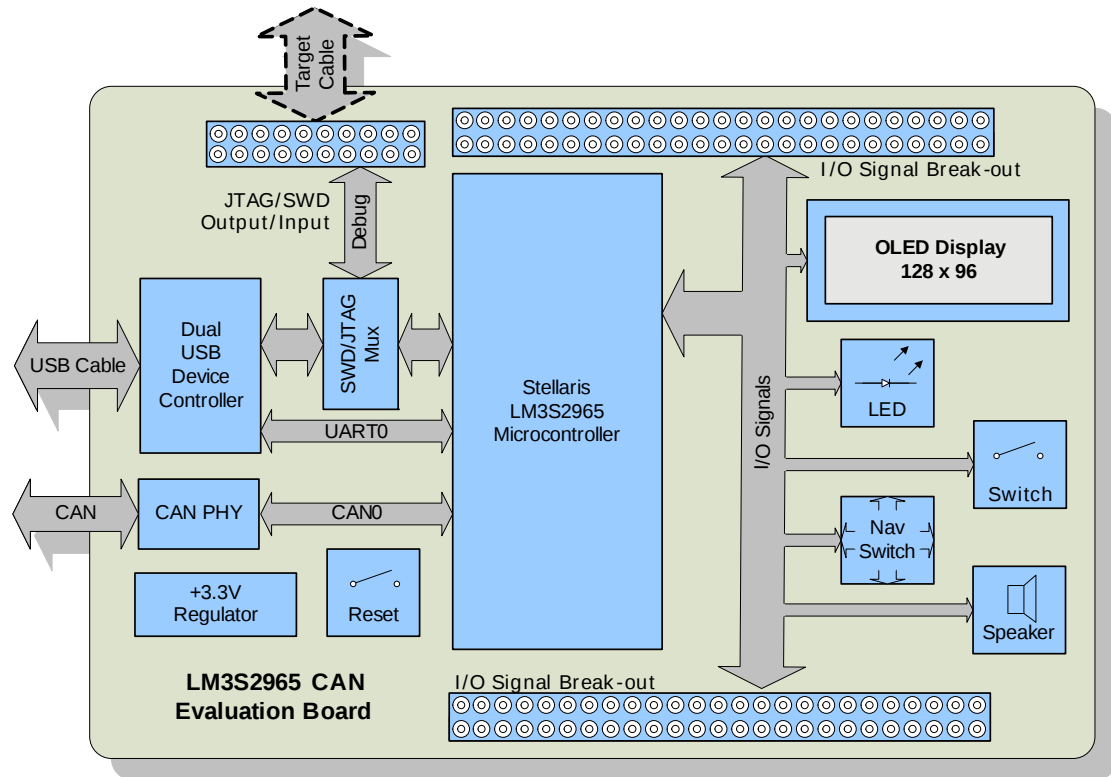
Figure 1-3. LM3S2965 Evaluation Board Block Diagram
