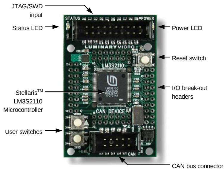
Figure 1-2. Stellaris LM3S2110 CAN Device Board
