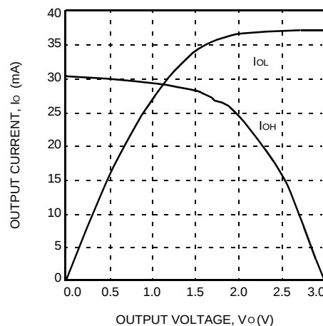
Figure 86. Sinklim ( T_J = 125^\circ\text{C} , V_{DD} = 3.0\text{ V} )
