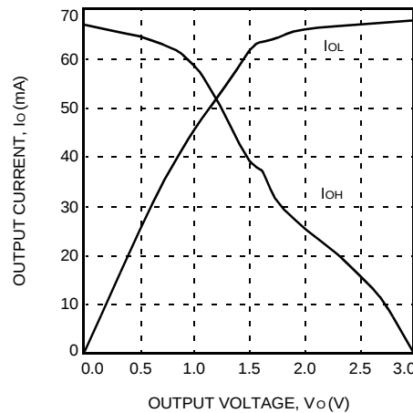
Figure 88. Fast ( T_J = 125^\circ\text{C} , V_{DD} = 3.0\text{ V} )
