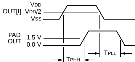
Figure 75. Output Buffer Delays
