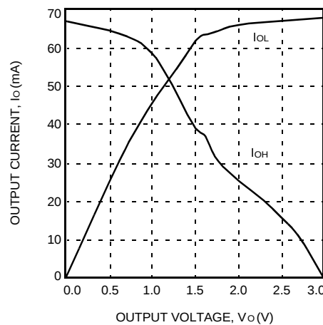
Figure 87. Slewlim ( T_J = 125^\circ\text{C} , V_{DD} = 3.0\text{ V} )
