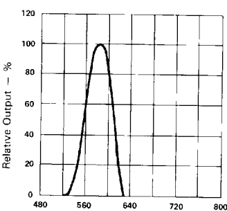
Fig 2 SPECTRAL RESPONSE
