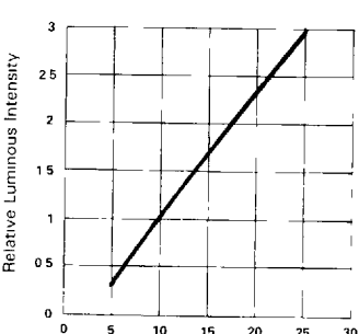
Fig 3 RELATIVE LUMINOUS INTENSITY V s FORWARD CURRENT (PFR SEGMENT)
