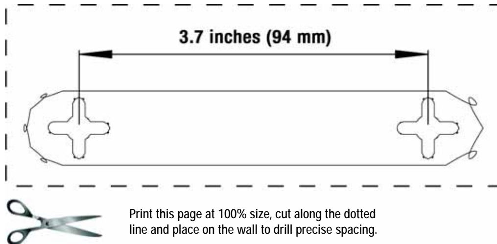
Figure 3-6: Wall-Mount Template
