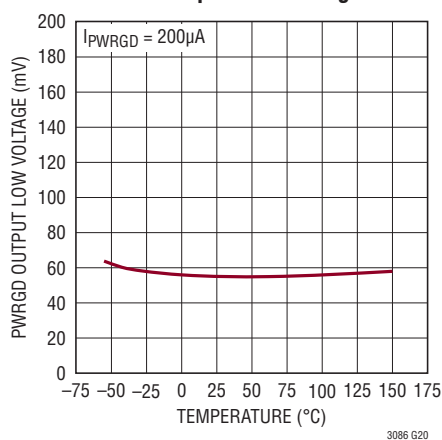
PWRGD Output Low Voltage
