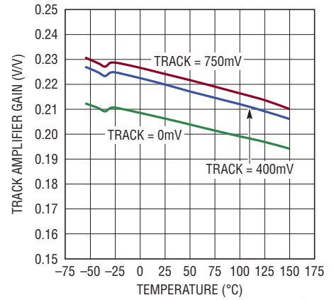
TRACK Amplifier Gain
