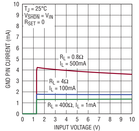
GND Pin Current, V_{OUT} = 0.4\text{V} (Light Load)
