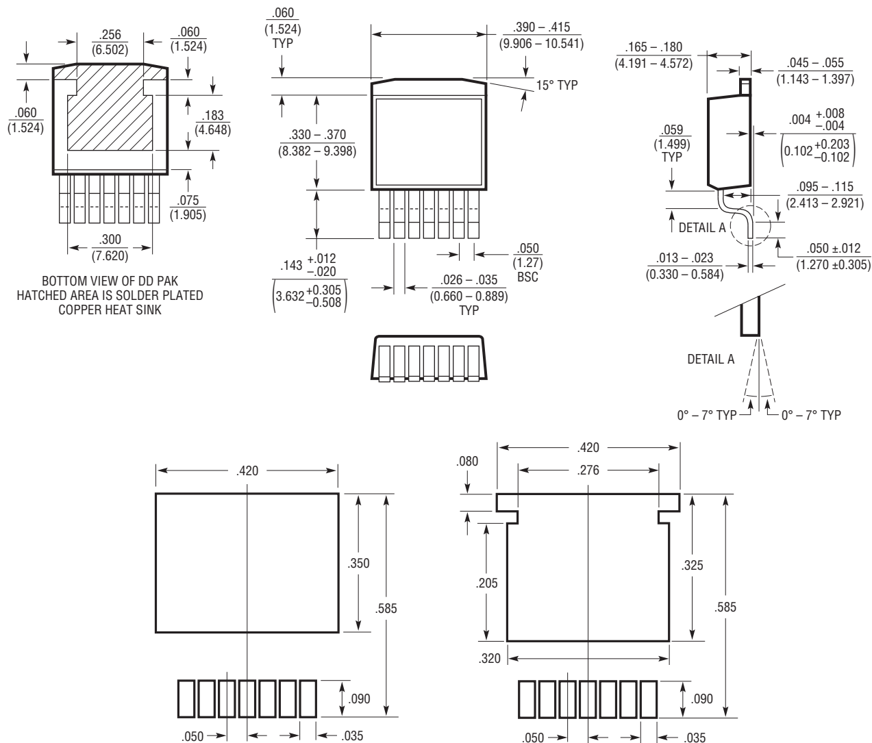
R Package 7-Lead Plastic DD Pak (Reference LTC DWG # 05-08-1462 Rev F)
