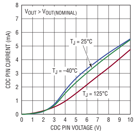
CDC Pin Internal Clamp Fault Current
