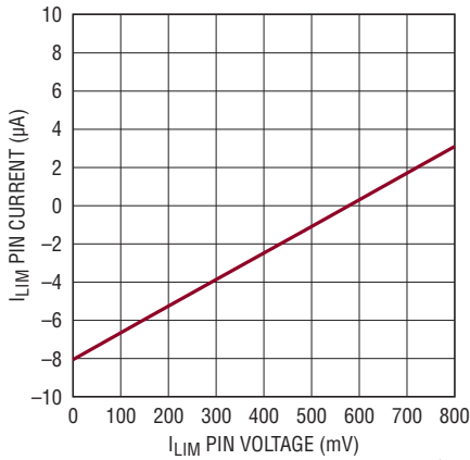
I_{LIM} Pin Input Current
