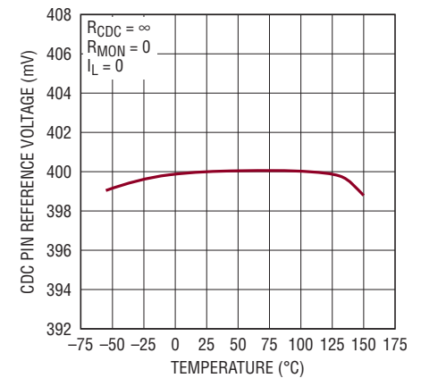
CDC Pin Reference Voltage
