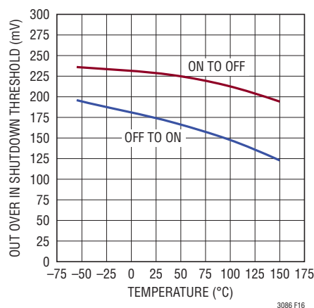
Figure 16. OUT Over IN Shutdown Threshold
