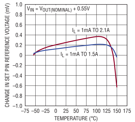
Reference Voltage Load Regulation
