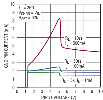
GND Pin Current, V_{OUT} = 5\text{V} (Light Load)
