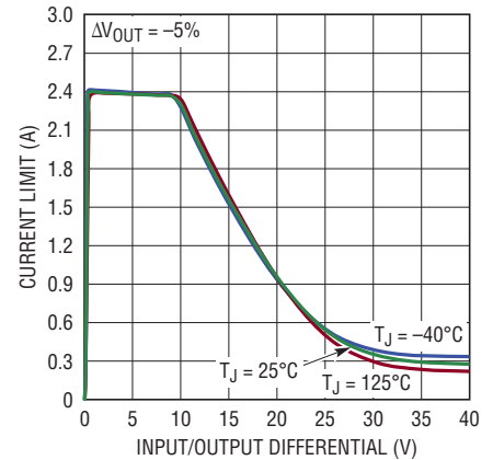
Internal Current Limit vs V_{IN} - V_{OUT}
