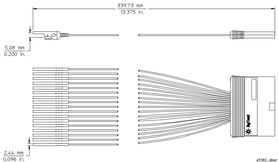
E5382A Single-ended Flying Lead Probe Set Dimensions
