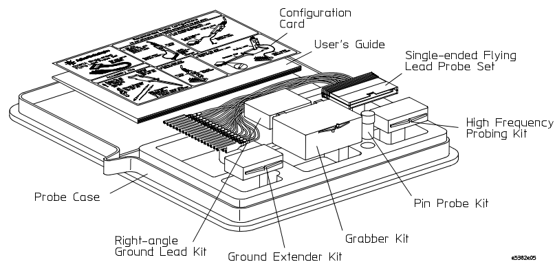
Probe case contents
