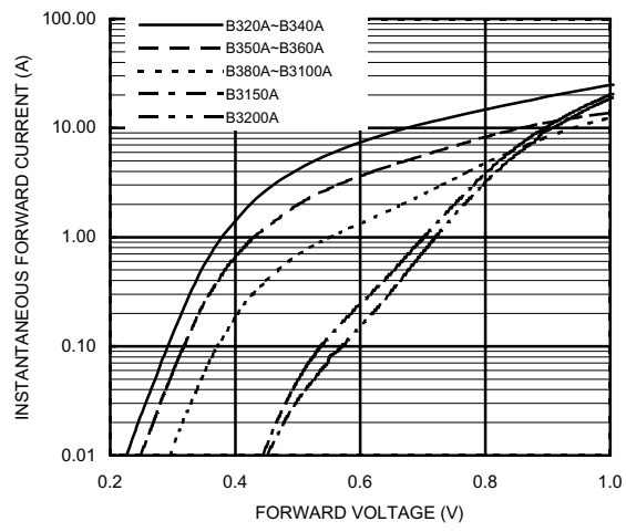
FIG. 2-TYPICAL FORWARD CHARACTERISTICS
