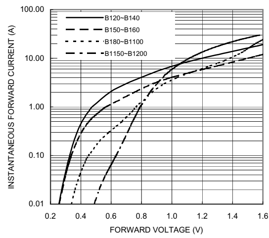
FIG. 2-TYPICAL FORWARD CHARACTERISTICS
