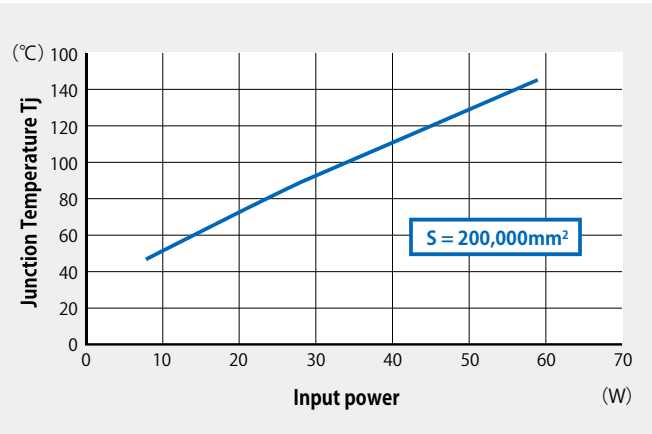
Figure-9 ( b ) Characteristic of input power - junction temperature Tj
