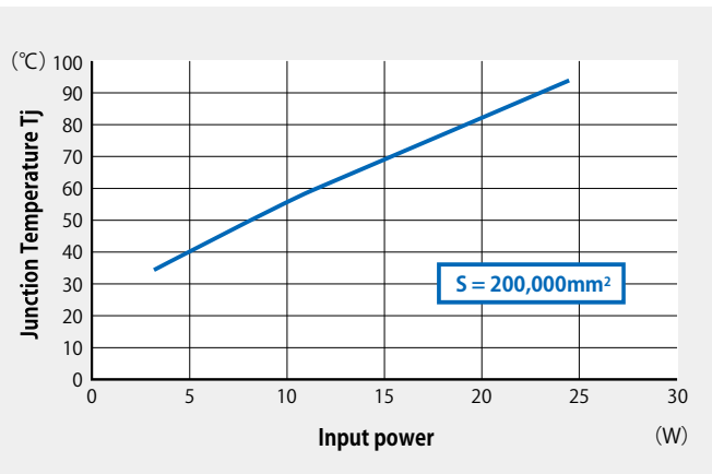
Figure-6 ( b ) Characteristic of input power - junction temperature T_j
