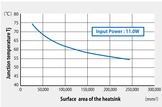
Figure-6 ( a ) Characteristic of heat sink surface area - junction temperature T_j
