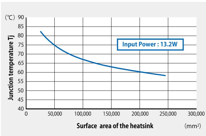
Figure-7 ( a ) Characteristic of heat sink surface area - junction temperature T_j
