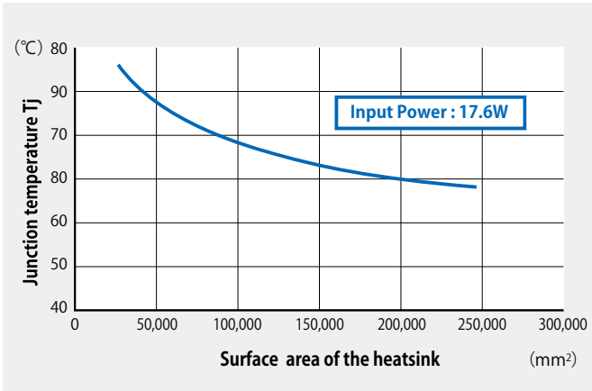
Figure-8 ( a ) Characteristic of heat sink surface area - junction temperature Tj
