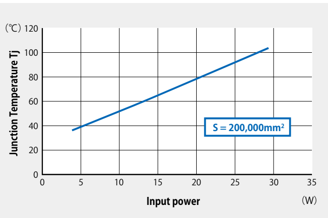
Figure-7 ( b ) Characteristic of input power - junction temperature T_j
