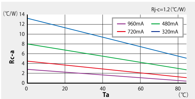
Figure-4 T_a - R_{c-a} ( CLL030-1208 A1 )
