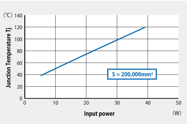
Figure-8 ( b ) Characteristic of input power - junction temperature Tj
