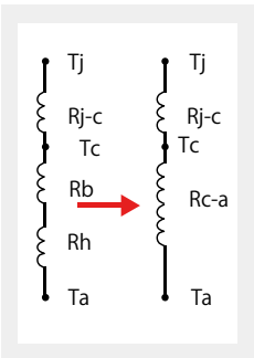
Figure-2 ( a ) Thermal Resistance Connection
