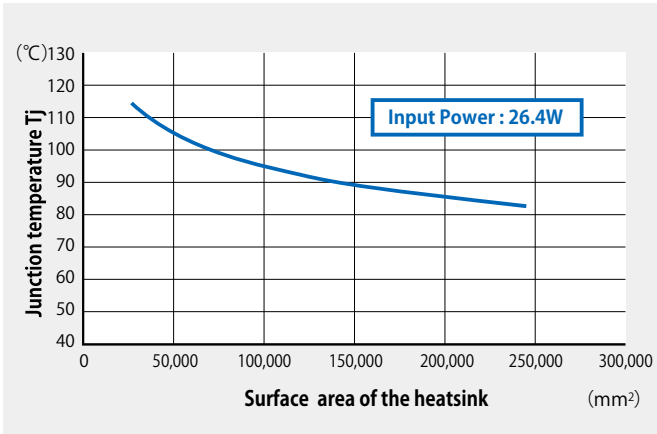
Figure-9 ( a ) Characteristic of heat sink surface area - junction temperature Tj
