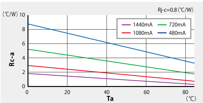
Figure-5 T_a - R_{c-a} ( CLL030-1212 A1 )
