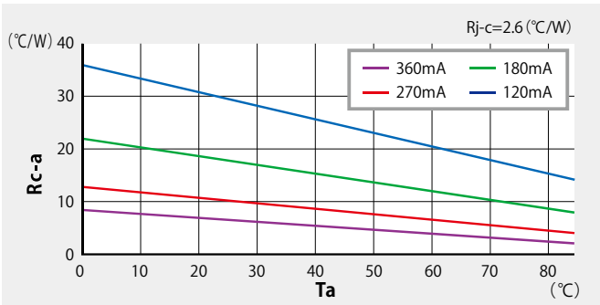
Figure-3 T_a - R_{c-a} ( CLL020-1203 A1 )
