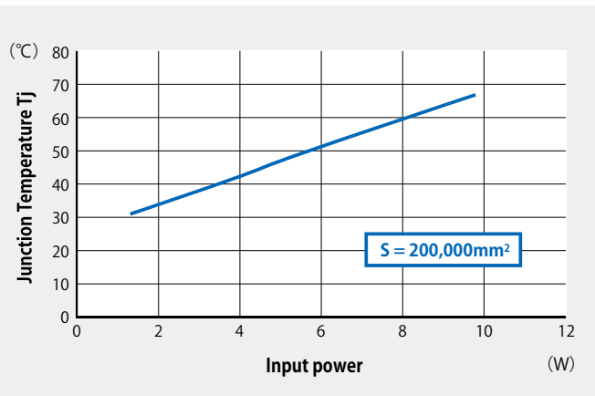
Figure-5 ( b ) Characteristic of input power - junction temperature T_j
