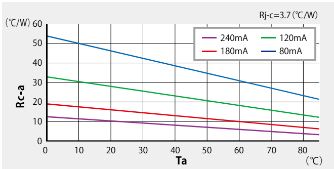
Figure-4 T_a - R_{c-a} ( CLL020-1204 A1 )
