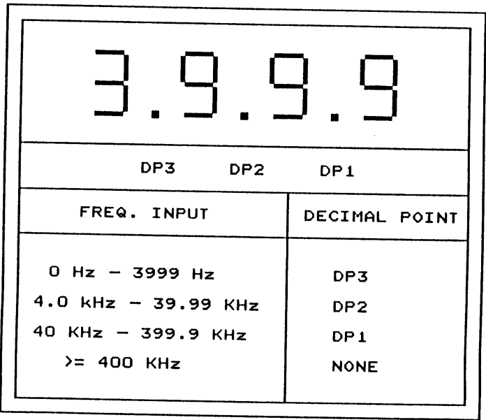
Fig.6 Autorange Decimal Point Selection Frequency Counter Input
