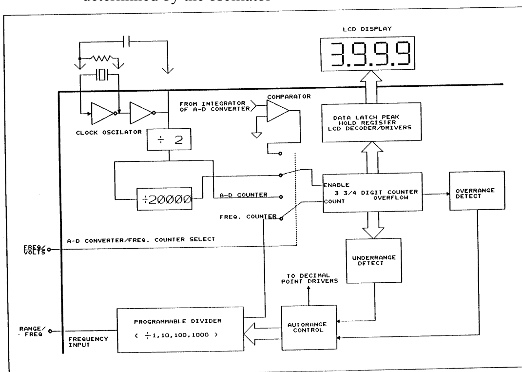
Fig. 5 Counter Operation
