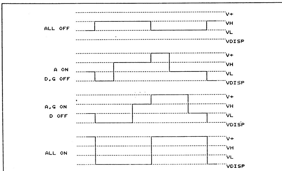
Fig.10 Typical Display Waveforms
