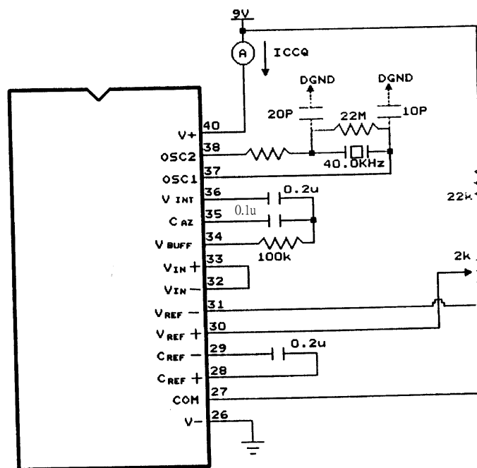
Fig.4 ICCQ Test Circuit
