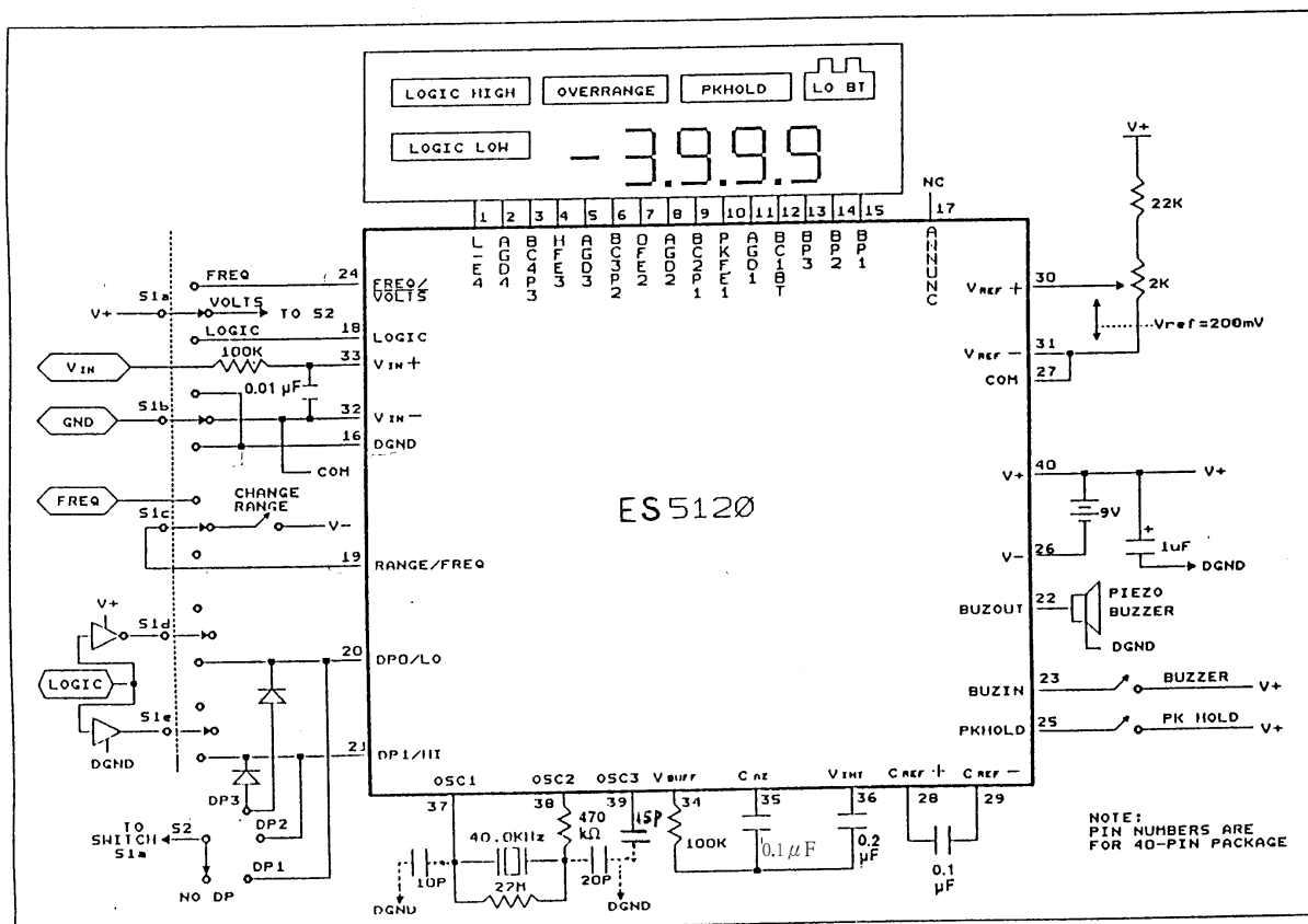
Fig. 1 Operating Circuit
