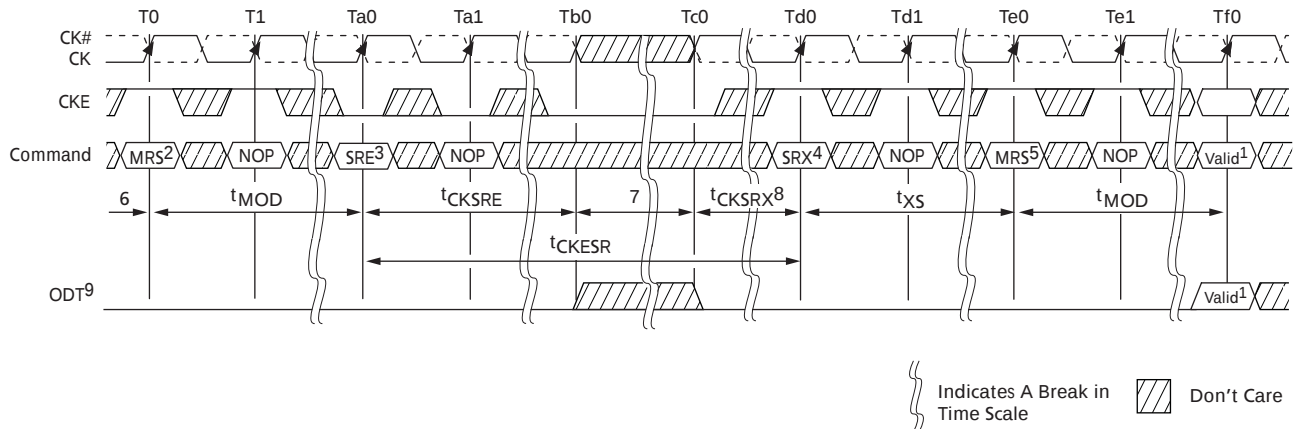
Figure 44: DLL Enable Mode to DLL Disable Mode
