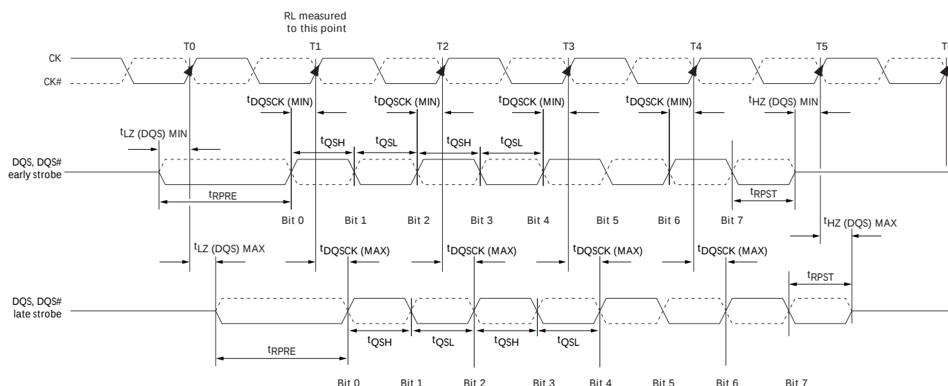
Figure 81: Method for Calculating t_{LZ} and t_{HZ}
