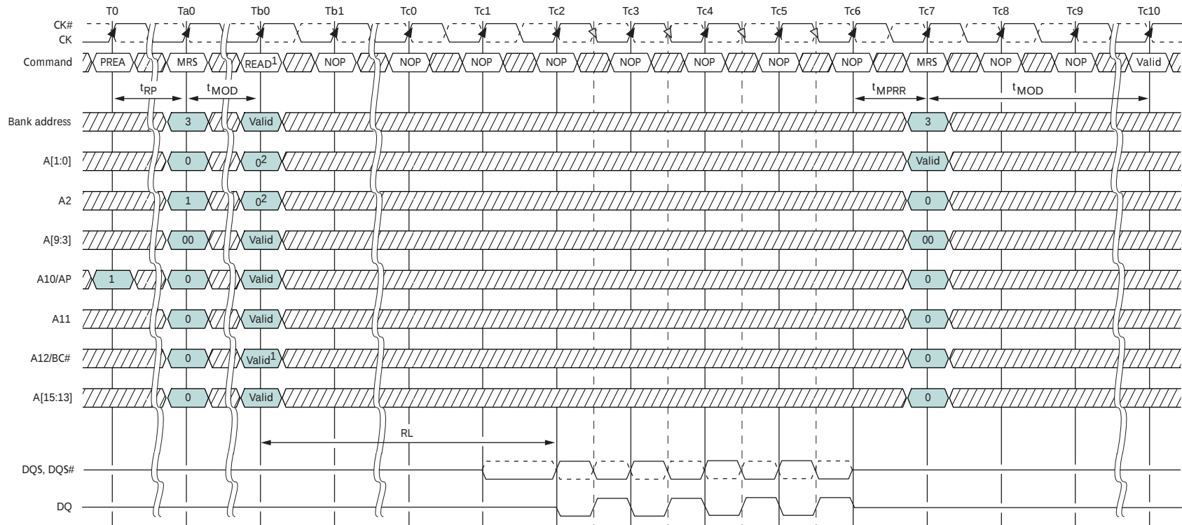
Figure 62: MPR System Read Calibration with BL8: Fixed Burst Order Single Readout
