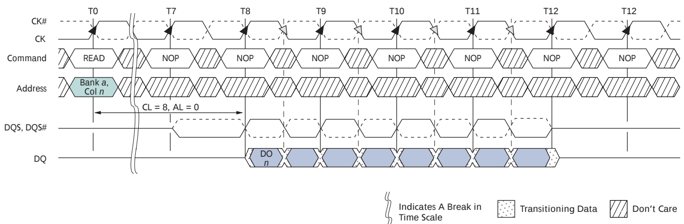
Figure 69: READ Latency
