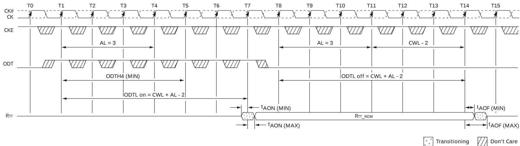
Figure 116: Synchronous ODT
