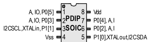
Figure 3. CY8C24123A 8-Pin PSoC Device
