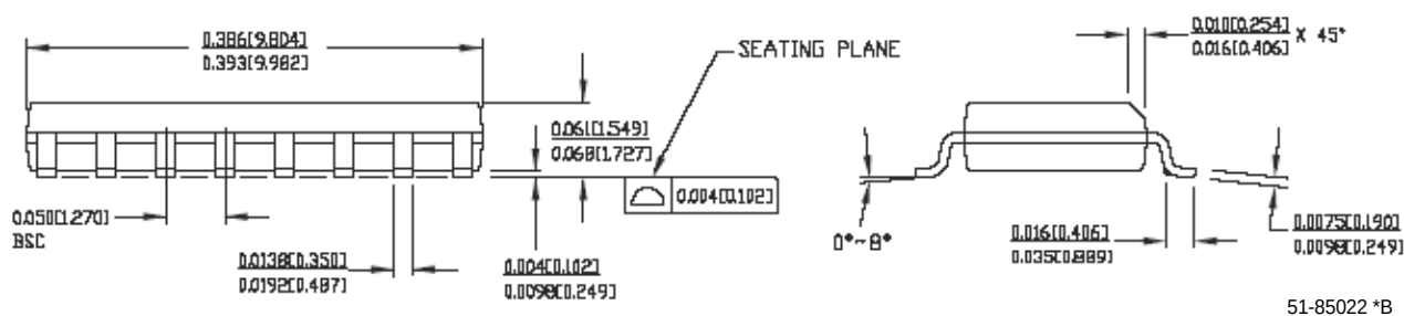
Figure 19. 16-Pin COL
