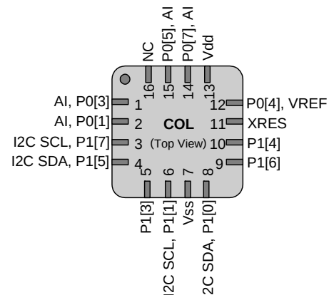
Figure 5. CY8C21223 16-Pin COL
