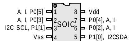
Figure 3. CY8C21123 8-Pin SOIC
