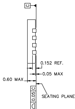
Figure 19. 16-Pin COL
