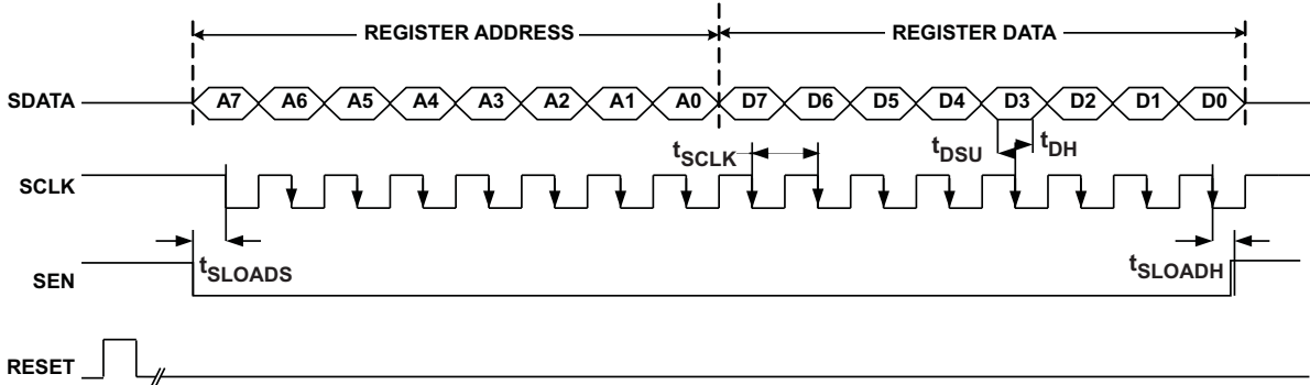
Figure 7. Serial Interface Timing
