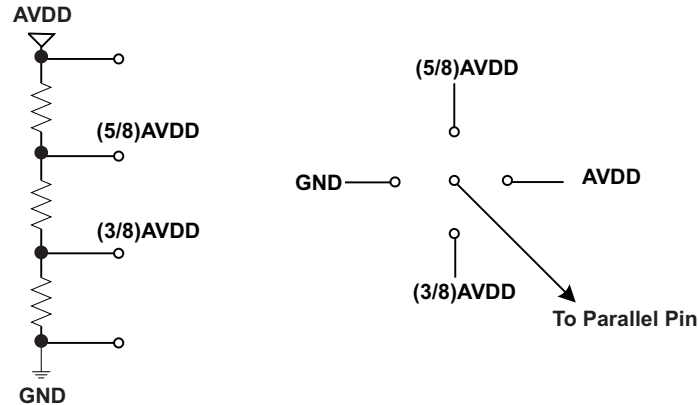
Figure 6. Simple Scheme to Configure Parallel Pins
