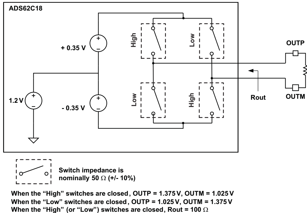
Figure 59. LVDS Buffer Equivalent Circuit
