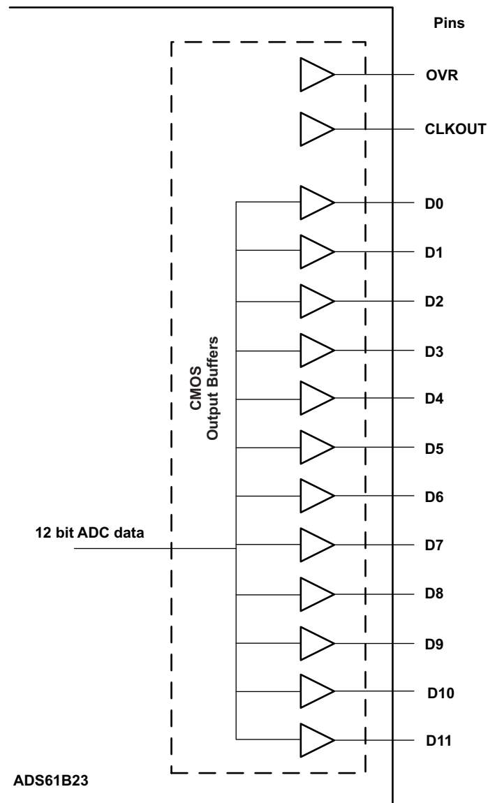
Figure 42. CMOS Output buffers
