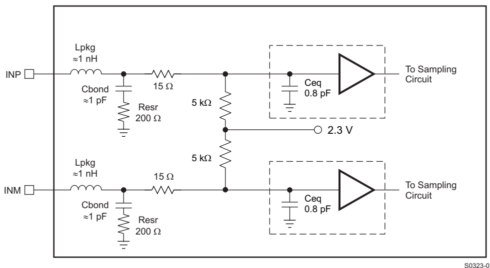
Figure 31. Input Stage
