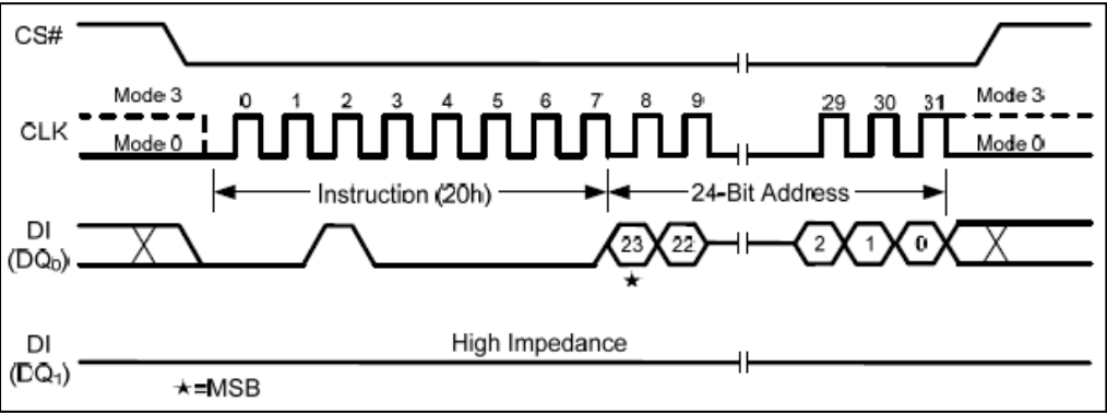
Figure 15 Sector erase instruction
