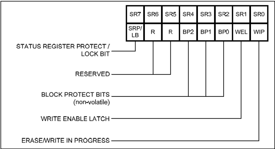
Figure 4 Status Register
