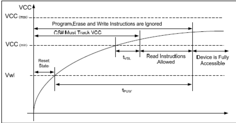
Figure 24 Power-up Timing
