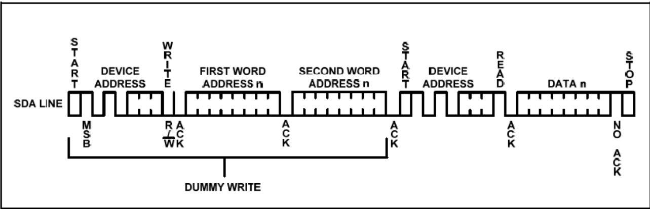
Figure 11 · Random Read
