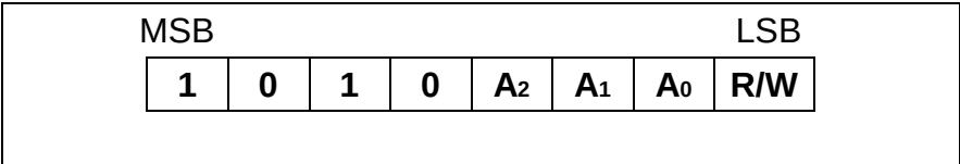
Figure 7 · Device Address
