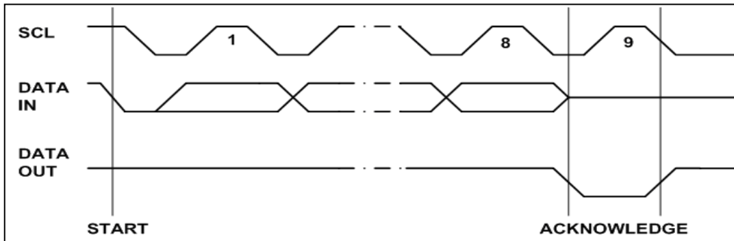
Figure 6 · Output Acknowledge
