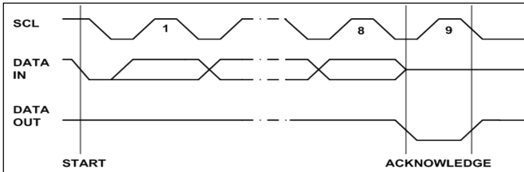
Figure 6 · Output Acknowledge
