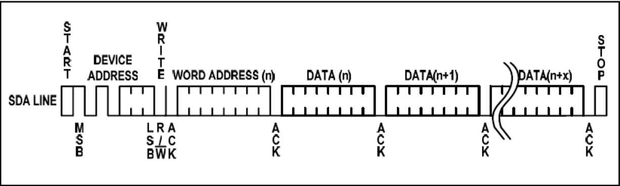
Figure 9 · Page Write
