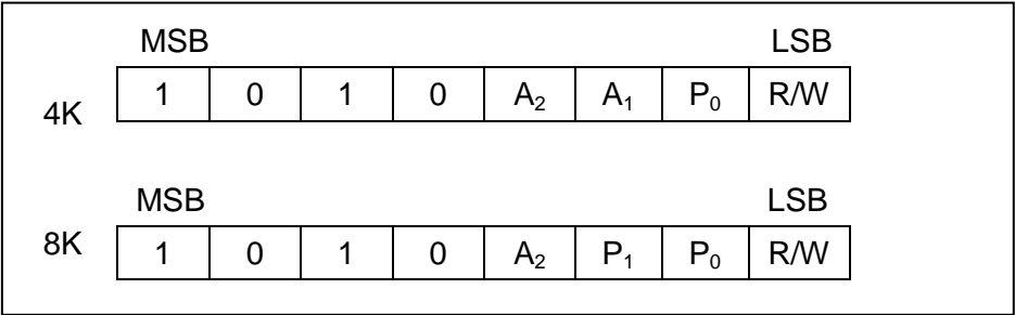
Figure 7 · Device Address
