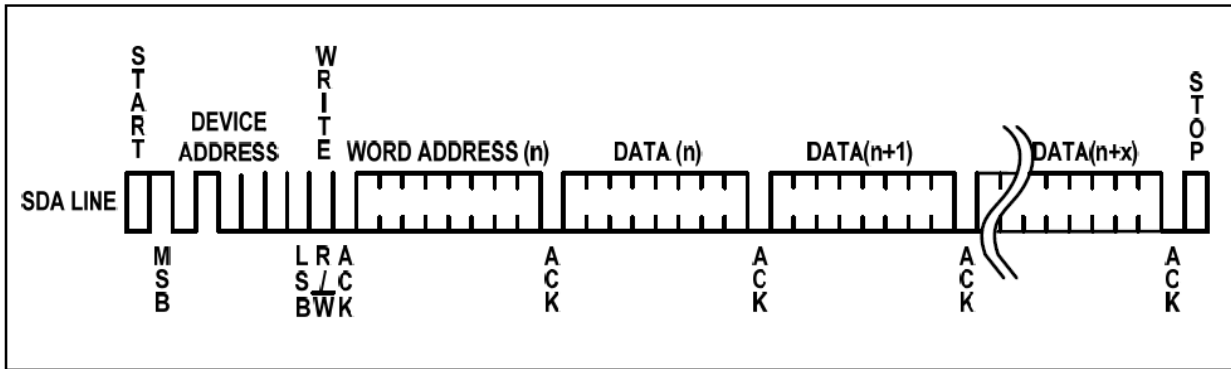
Figure 9 · Page Write
