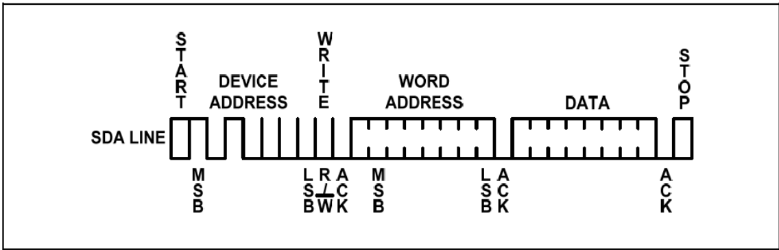
Figure 8 · Byte Write
