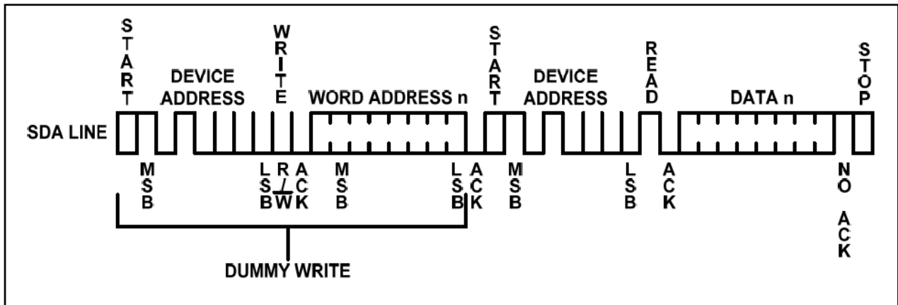
Figure 11 · Random Read
