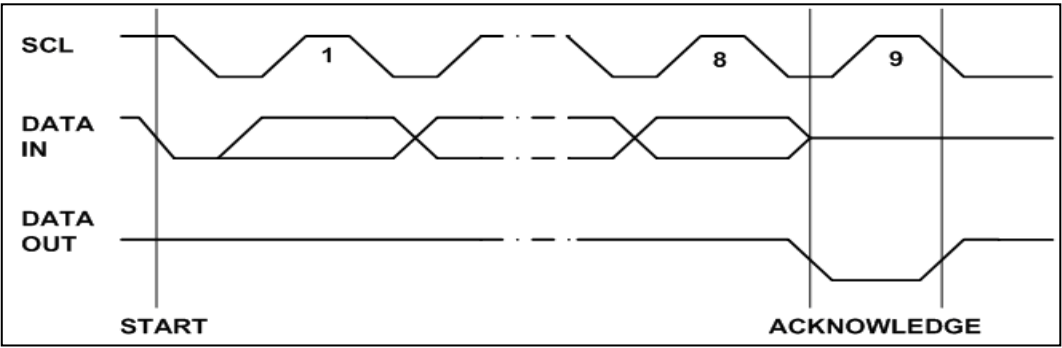
Figure 6 · Output Acknowledge
