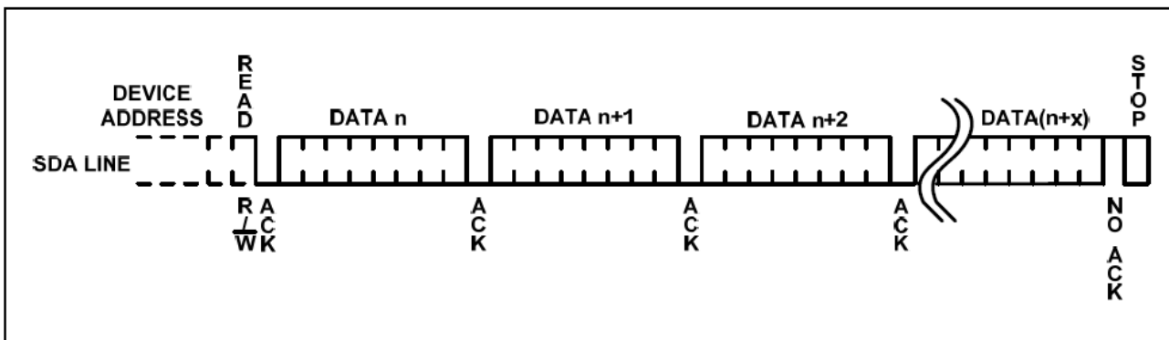
Figure 12 · Sequential Read
