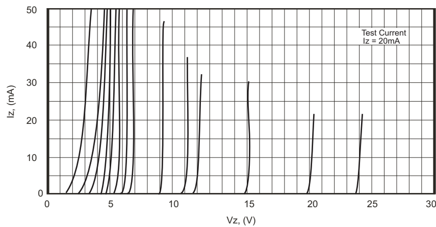
Fig.2 - Breakdown Characteristics
