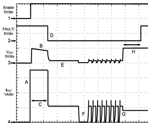
Figure 3. Kickstart Operation
