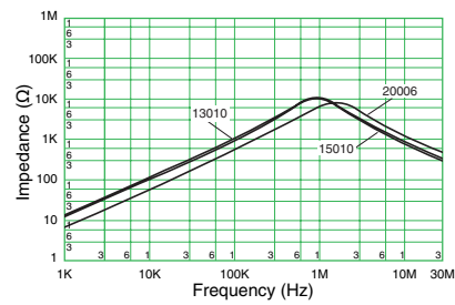
Frequency characteristic
