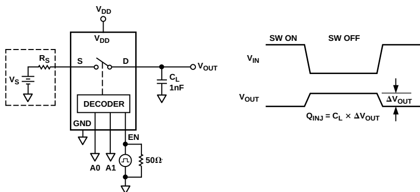
Test Circuit 6. Charge Injection
