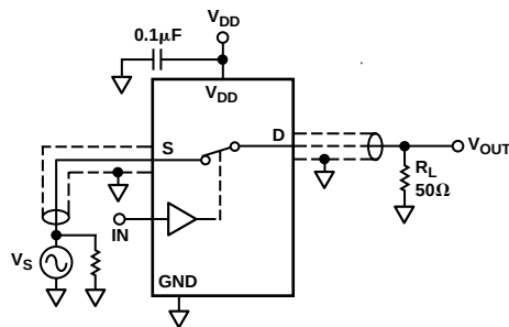
Test Circuit 9. Bandwidth
