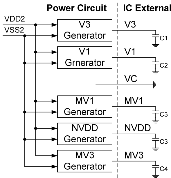
Fig 8. Power Circuit
