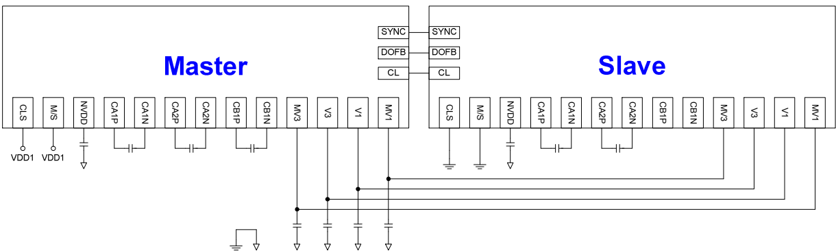
Fig 19. Reference Application Circuit: Master/Slave Connection with Internal Power
