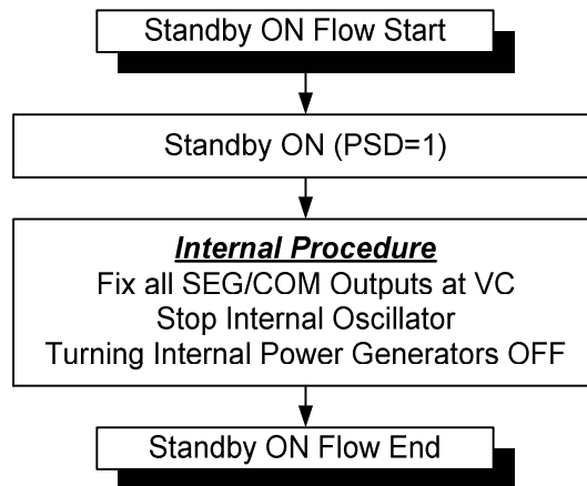
Fig 14. Standby ON Flow
