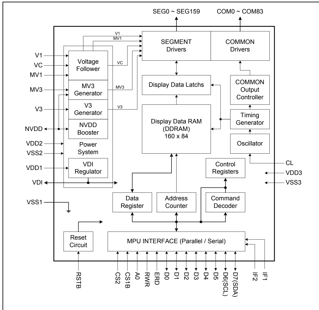
Fig 1. Block Diagram
