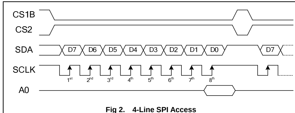
Fig 2. 4-Line SPI Access
