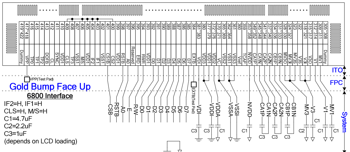
Fig 16. Reference Application Circuit: Parallel 6800 Interface
