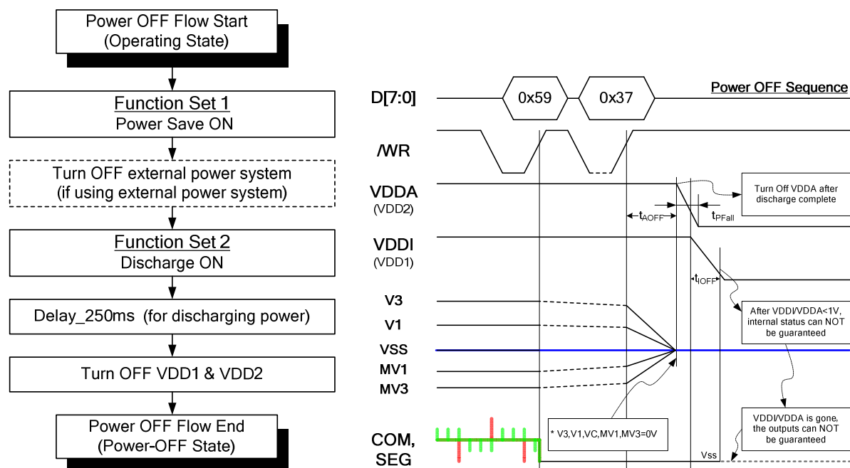
Power OFF Flow and Power OFF Sequence
