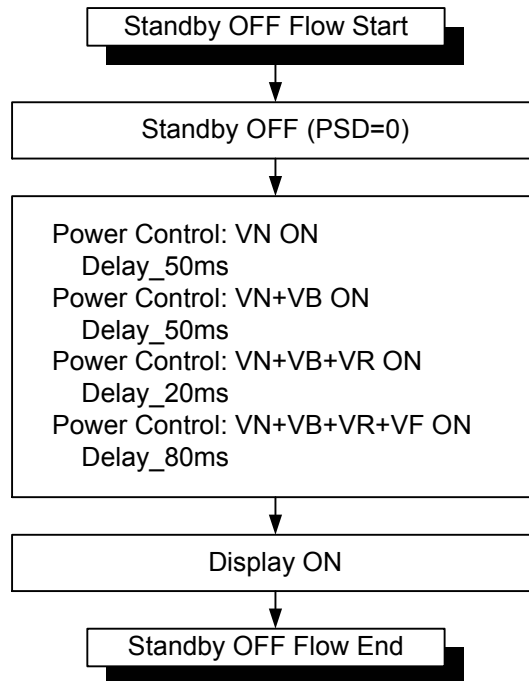
Fig 15. Standby OFF Flow
