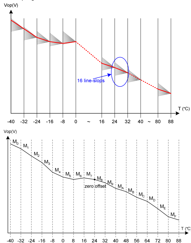
Fig 10. Programmable Vop Temperature Compensation
