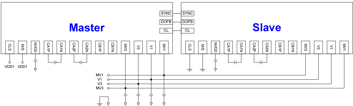
Fig 20. Reference Application Circuit: Master/Slave Connection with External Power
