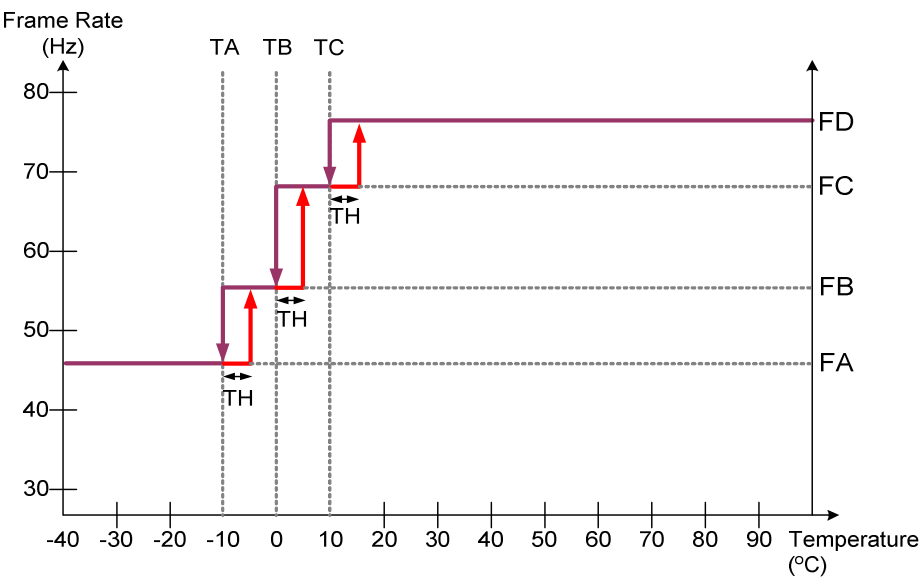
Fig 11. Frame Rate vs. Temperature
