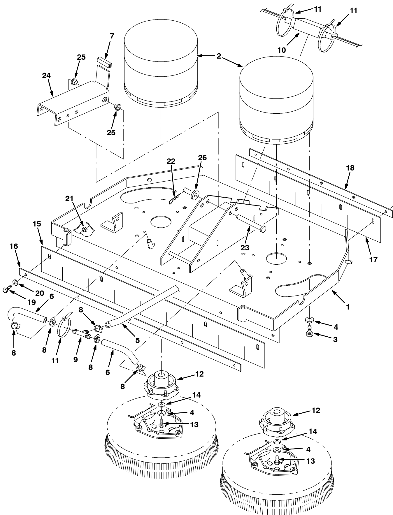
Fig. 28 - Rollout Battery Disk Scrub Head Drive Motor Group, 800 mm (32 in)
