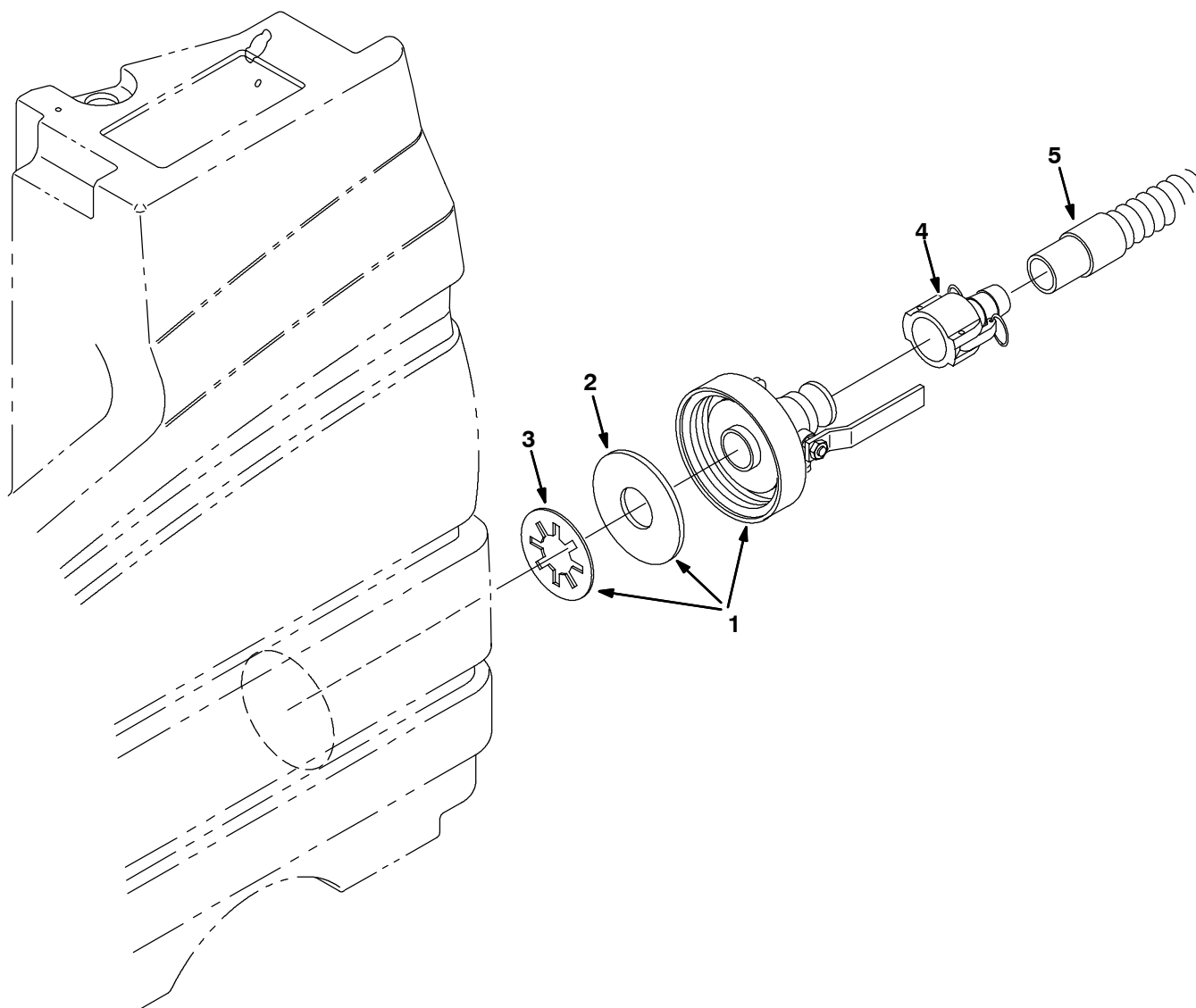
Fig. 45 - Positive Solution Control Drain Kit, Std
