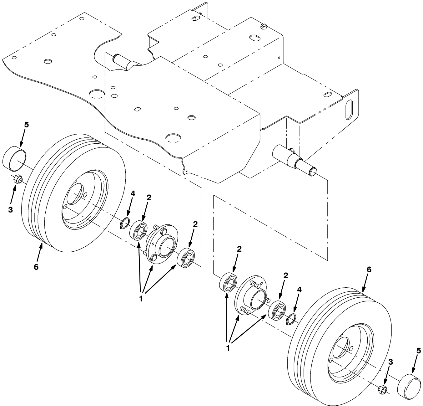
Fig. 15 - Rear Wheel Group
