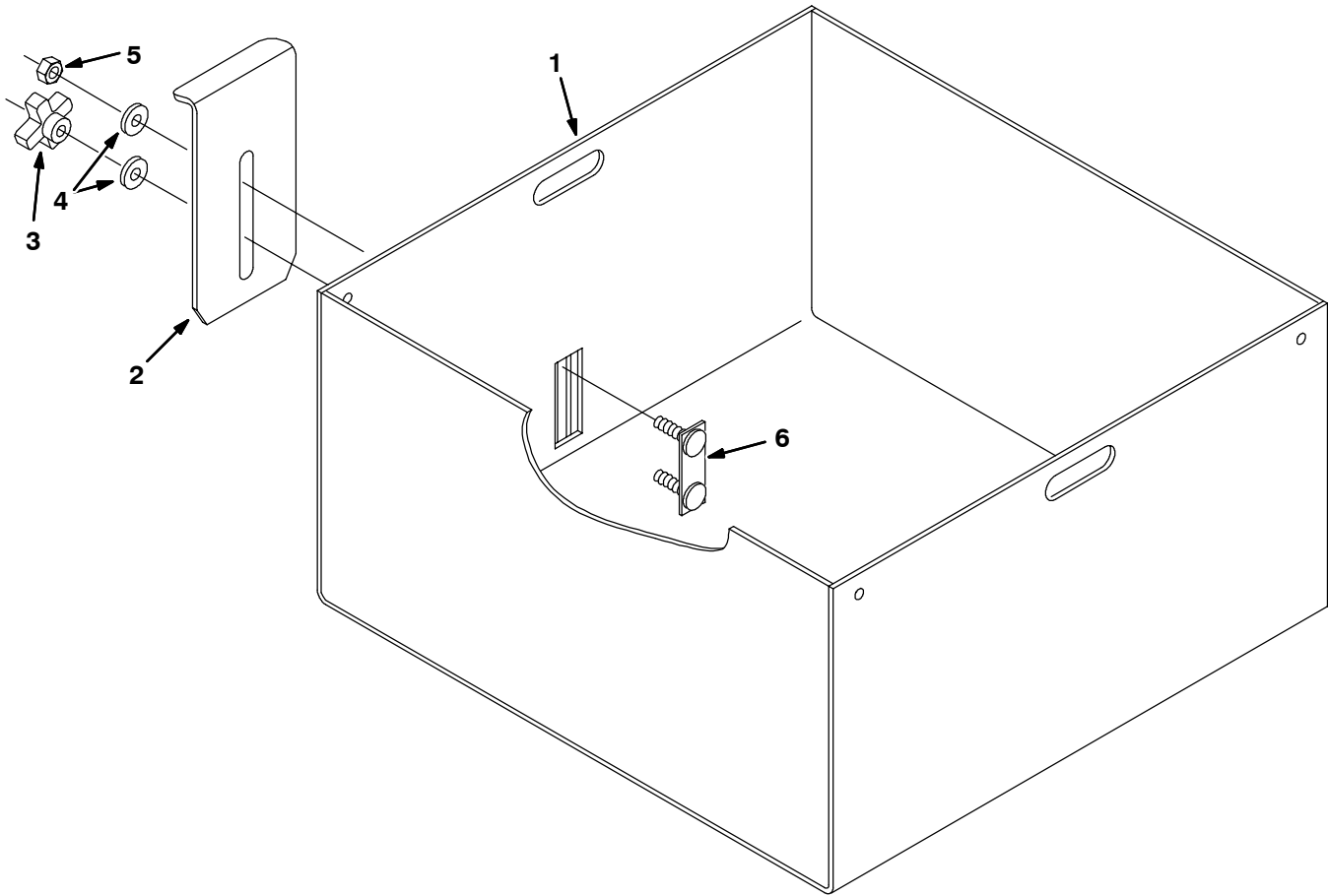
Fig. 32 - Rollout Battery Extra Case Kit
