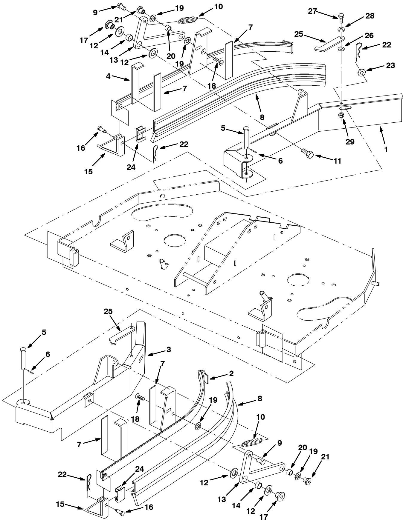
Fig. 19 - Disk Scrub Head Squeegee Group, 800 mm (32 in)
