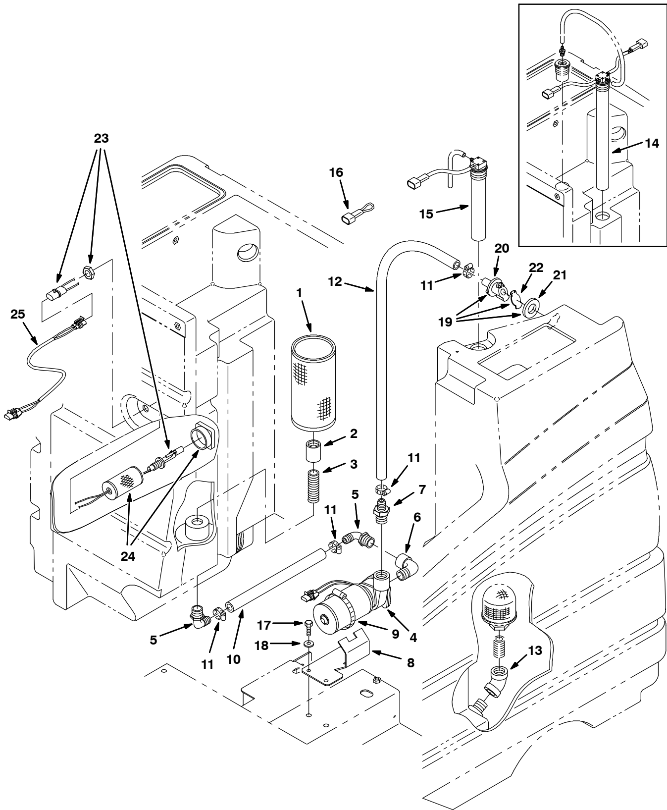
Fig. 2 - ES™ Pump Group
