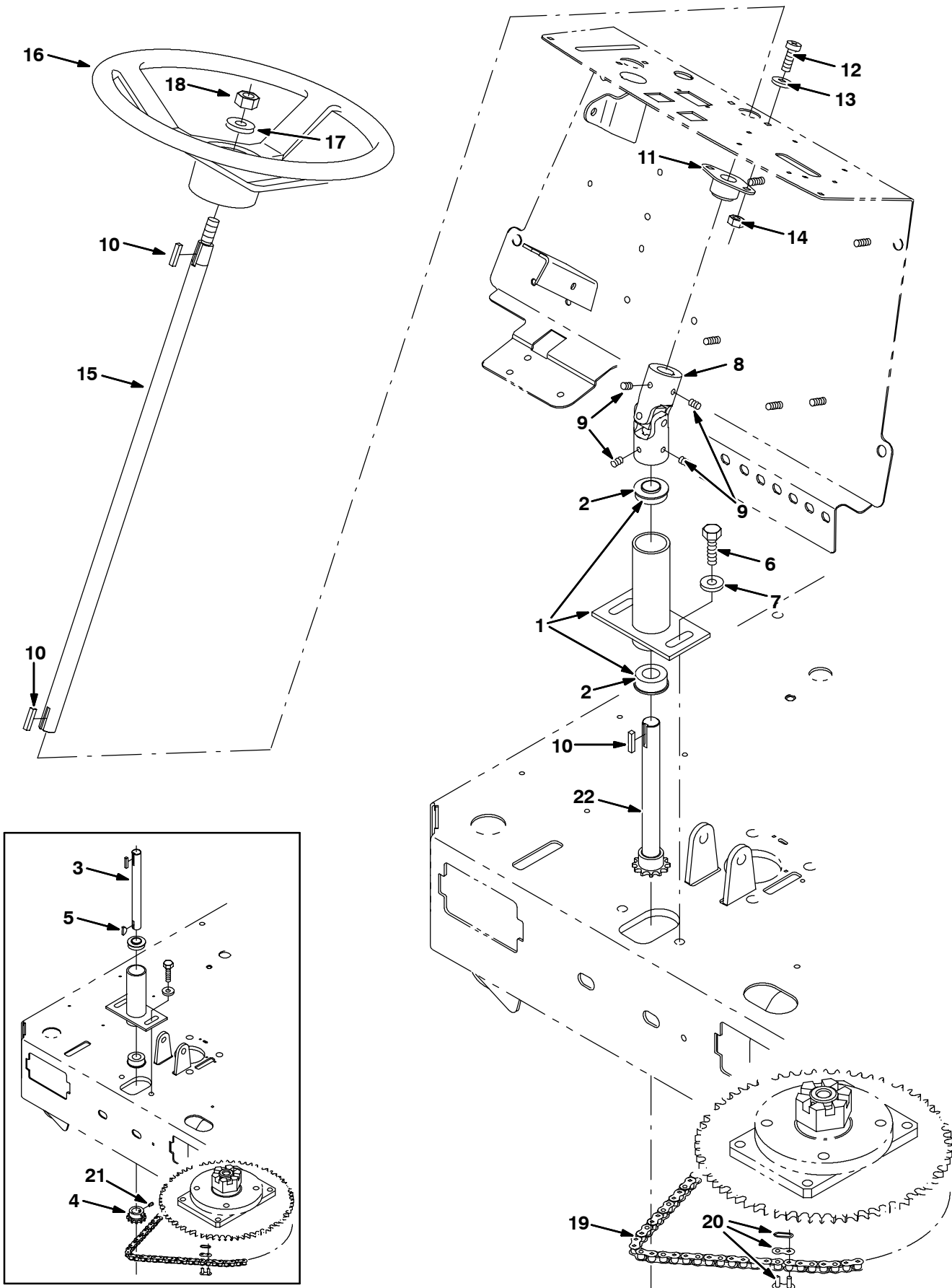
Fig. 7 - Steering Group
