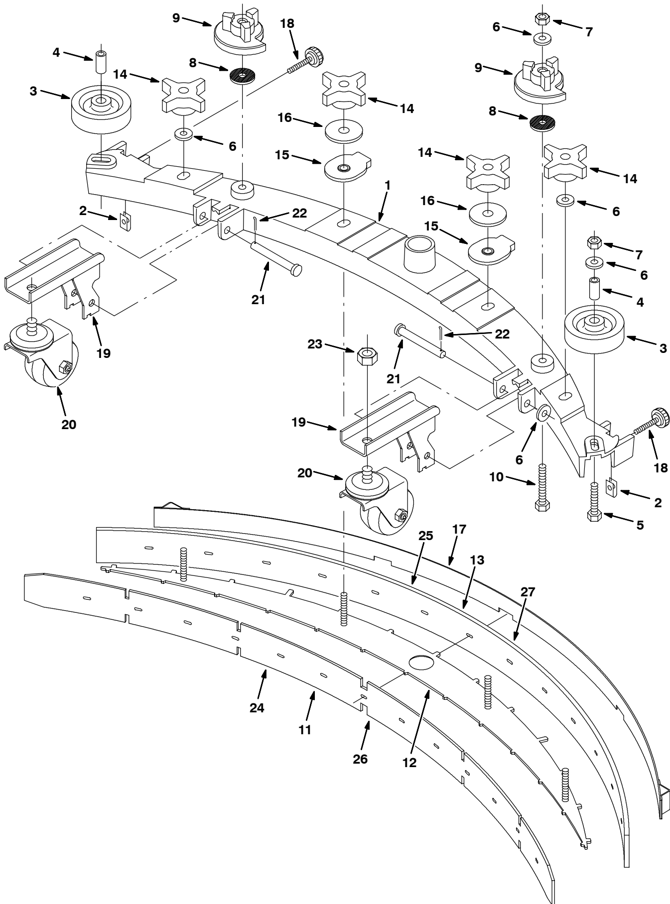
Fig. 37 - Rear Squeegee Group, 800 mm (32 in)
