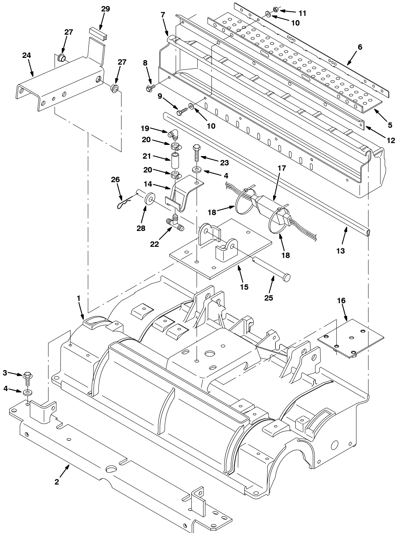
Fig. 29 - Rollout Battery Cylindrical Scrub Head Frame Group, 700 mm (28 in)
