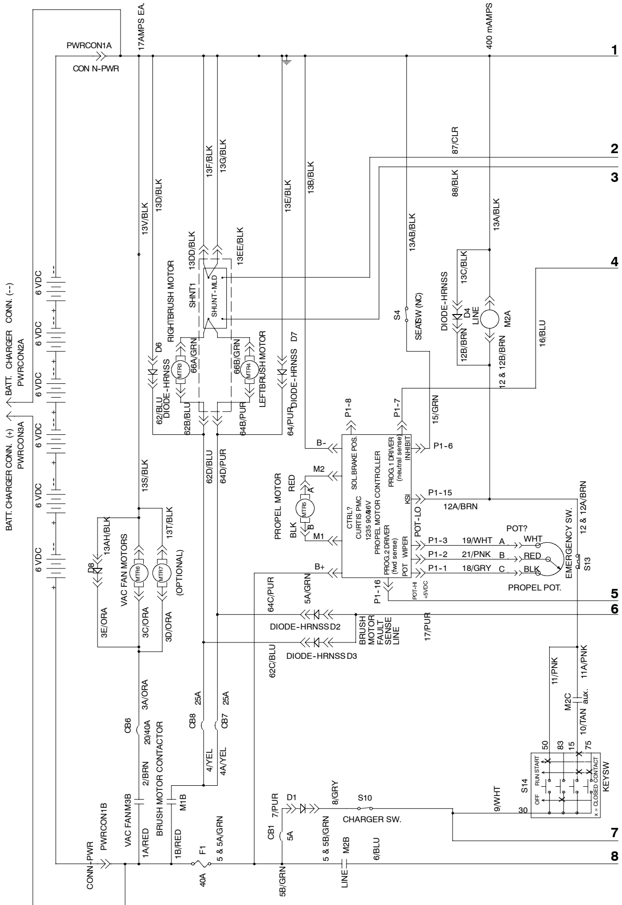
Fig. 29 - Electrical Schematic
