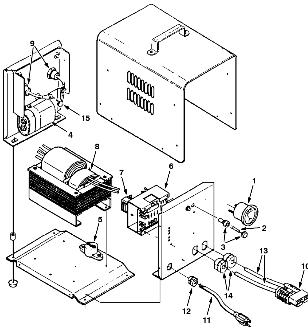
Fig. 5 - Battery Charger Breakdown, 50 Hz (305 Ah batteries), 222691
