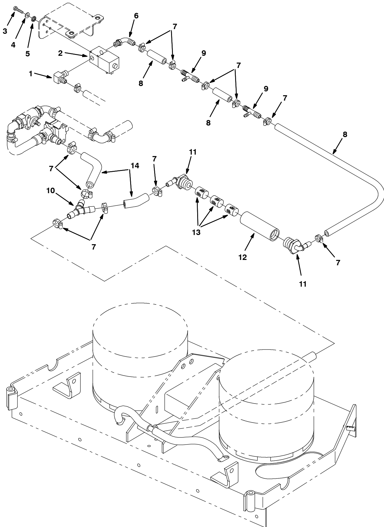
Fig. 6 - FaST™ Foam Filter Group, Disk Scrub Head
