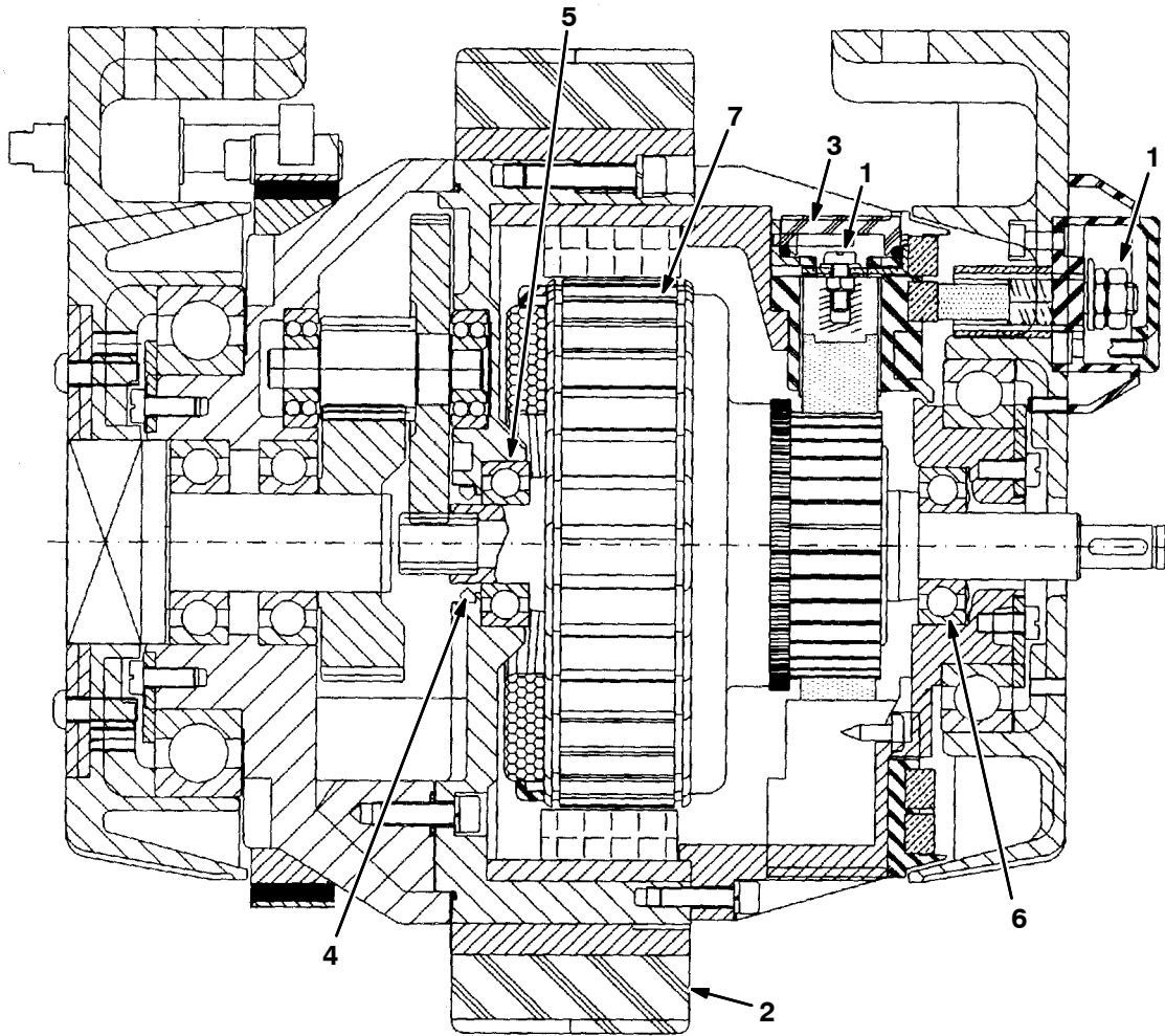
Fig. 7 - Front Wheel Gearbox Breakdown, 390851
