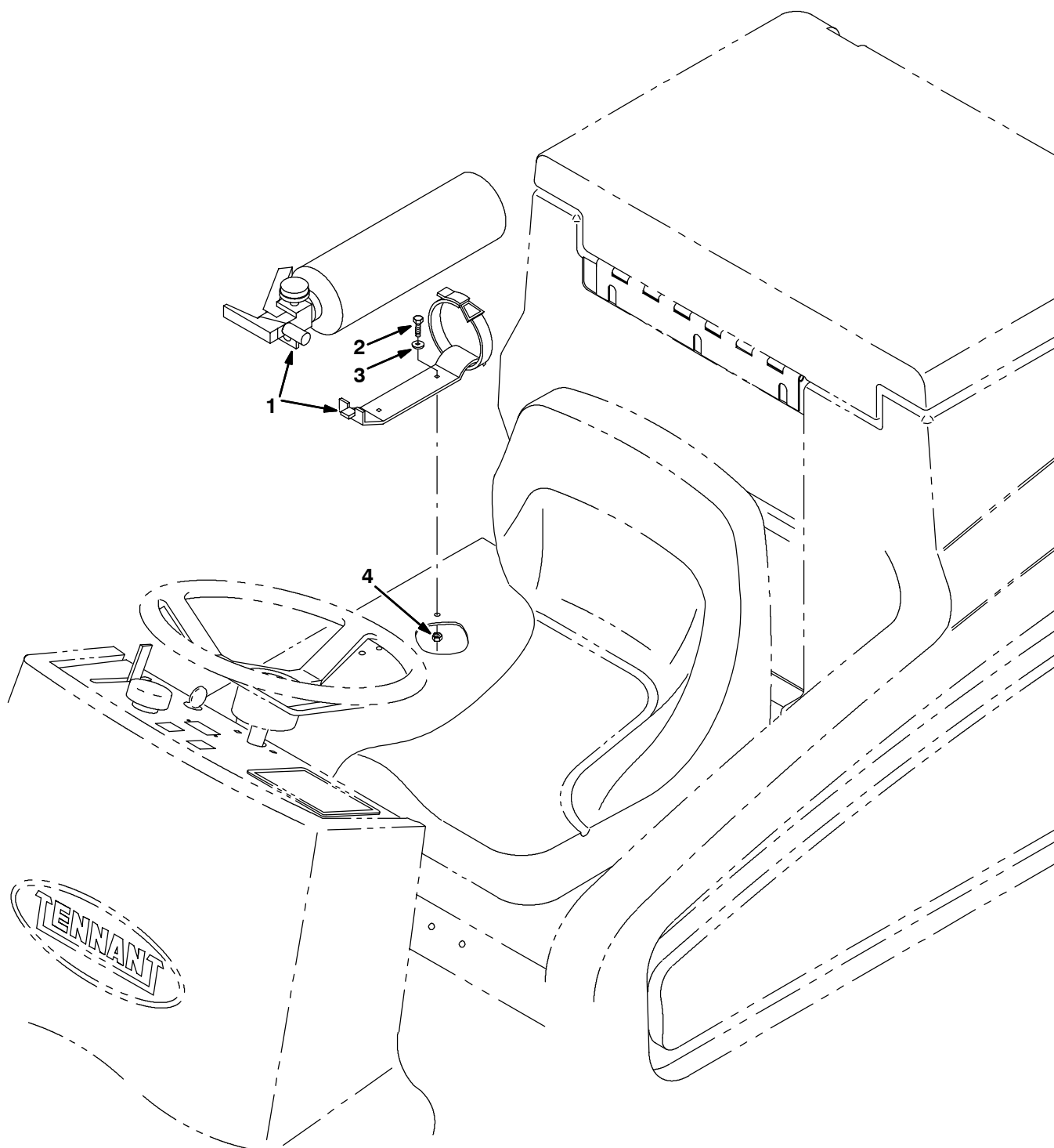
Fig. 41 - Fire Extinguisher Kit
