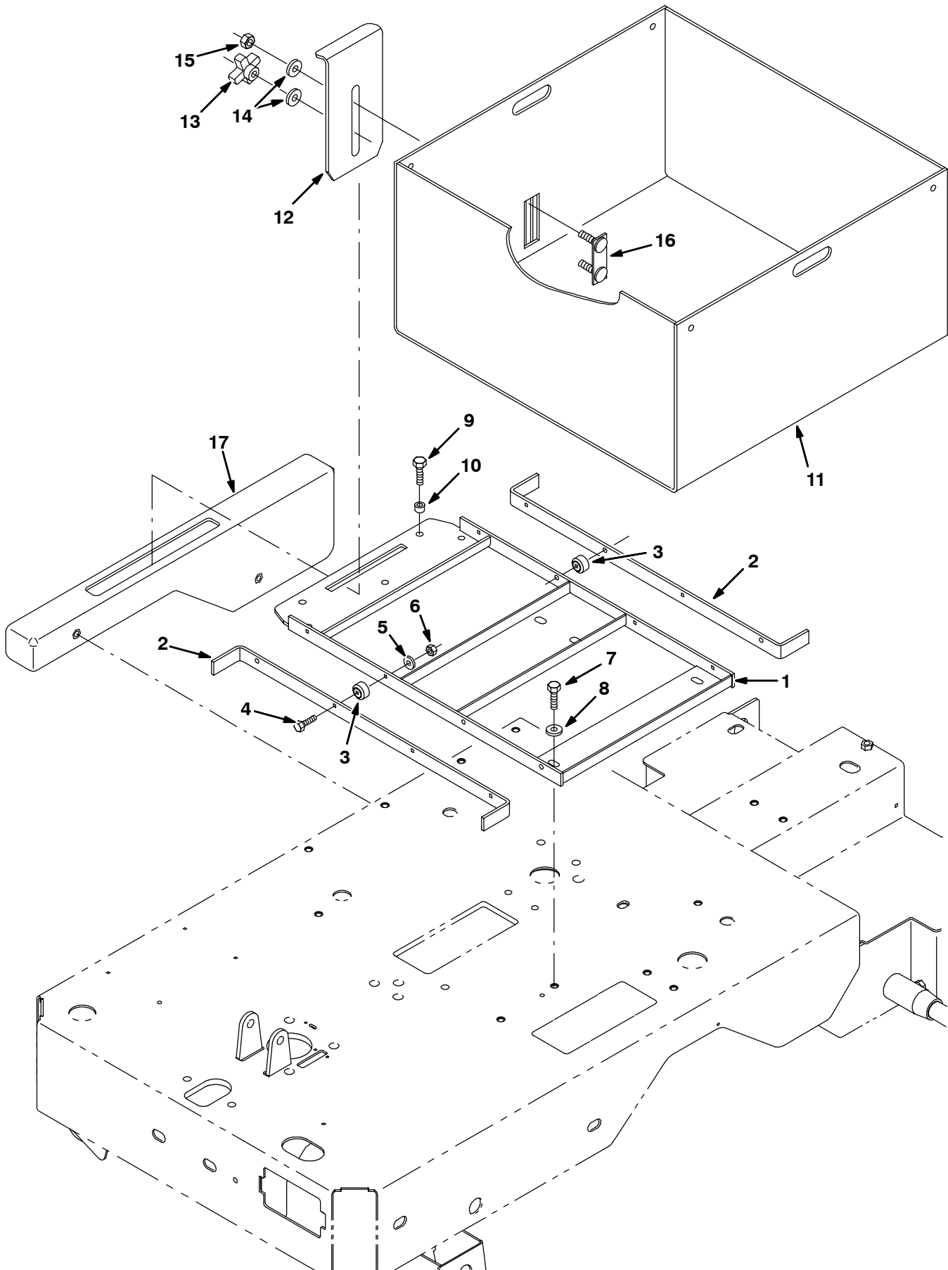
Fig. 31 - Rollout Battery Case Group
