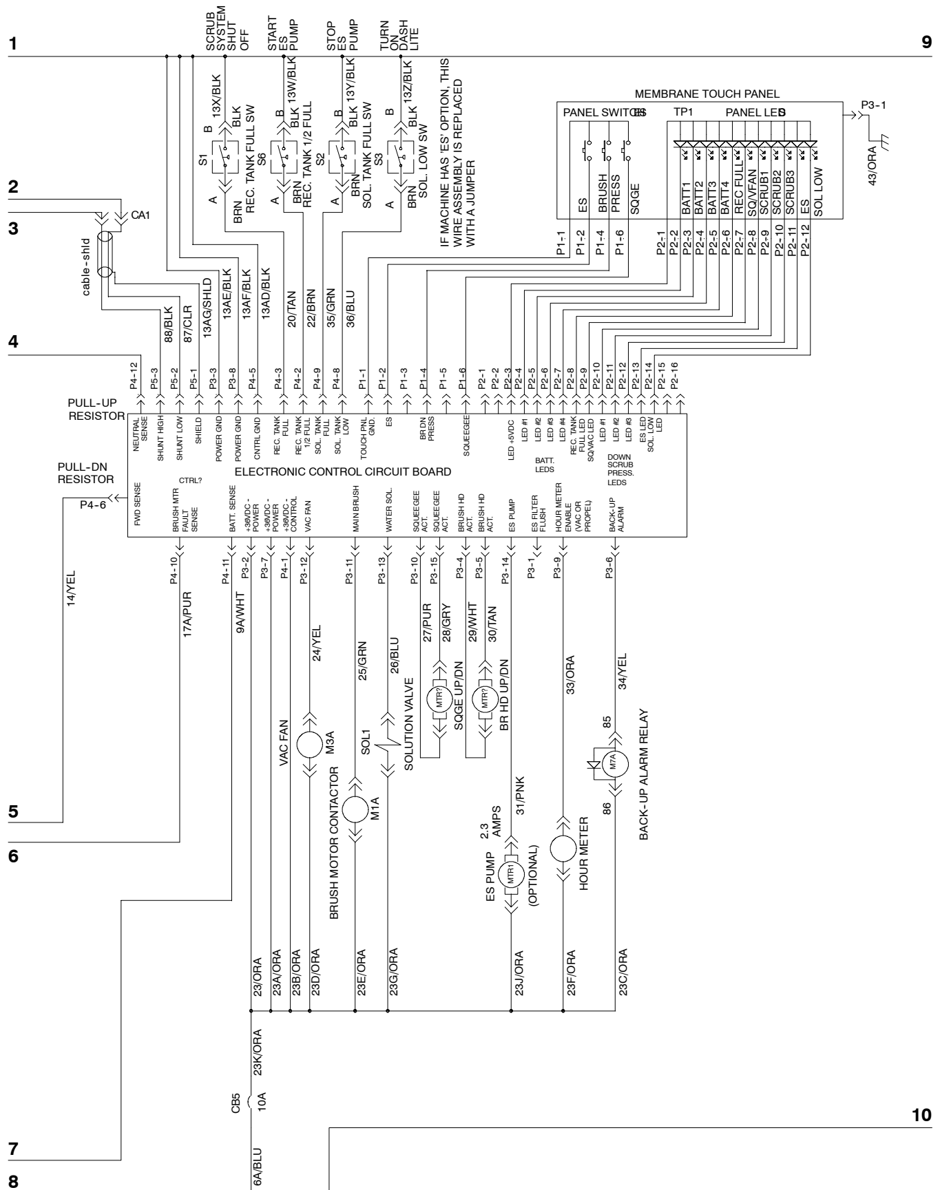
Fig. 29 - Electrical Schematic
