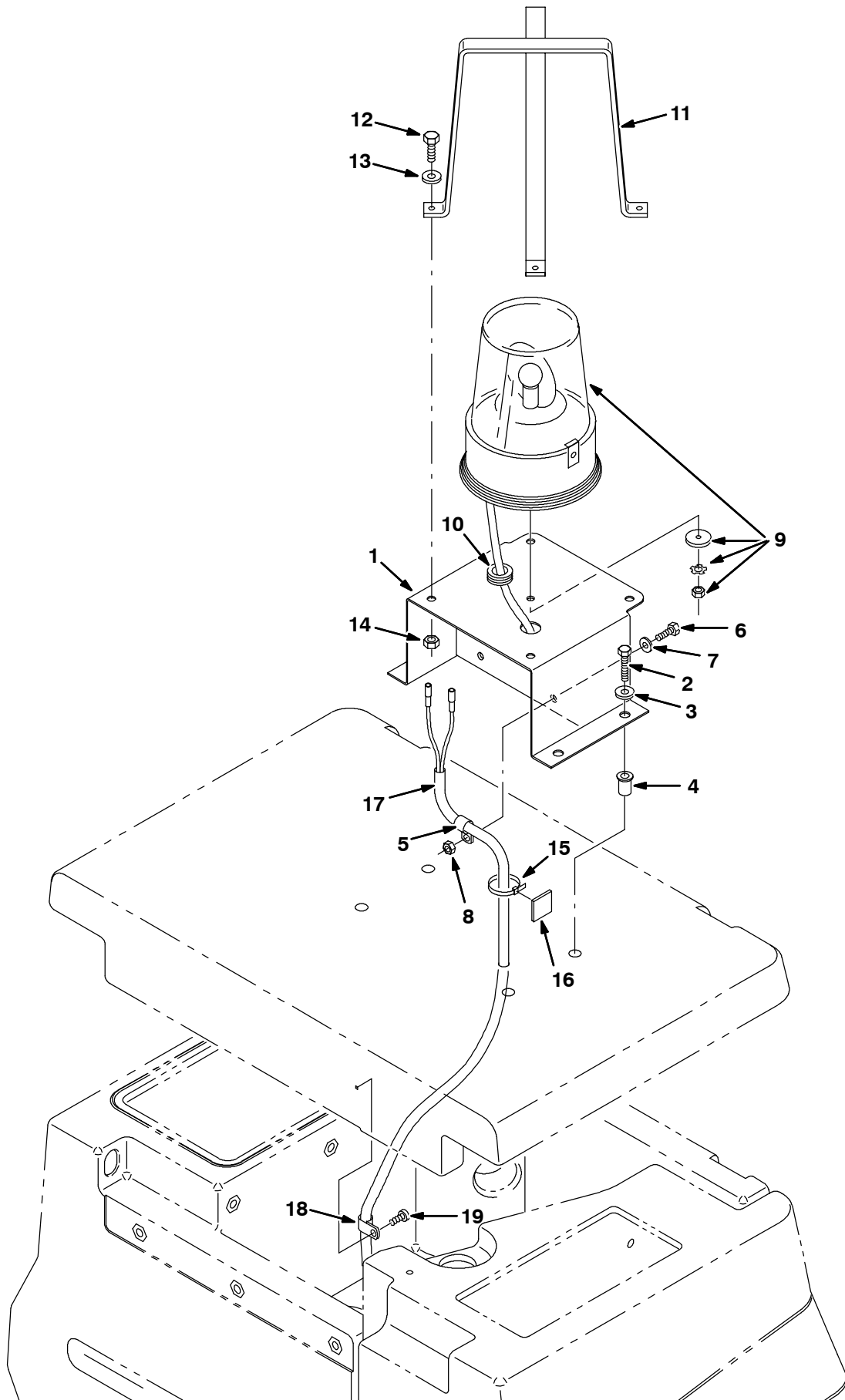
Fig. 42 - Revolving Light Kit
