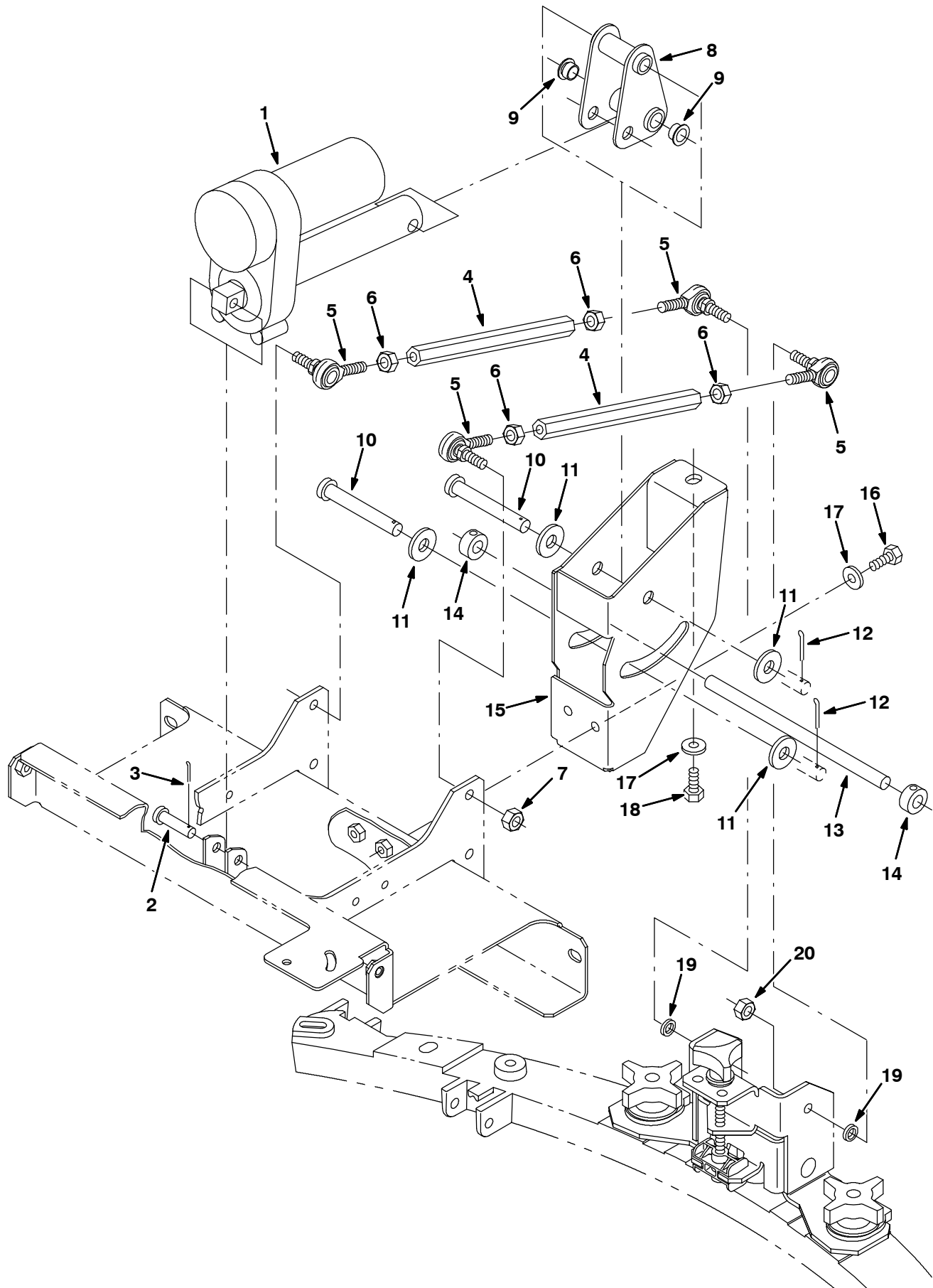
Fig. 26 - Rear Squeegee Lift Group
