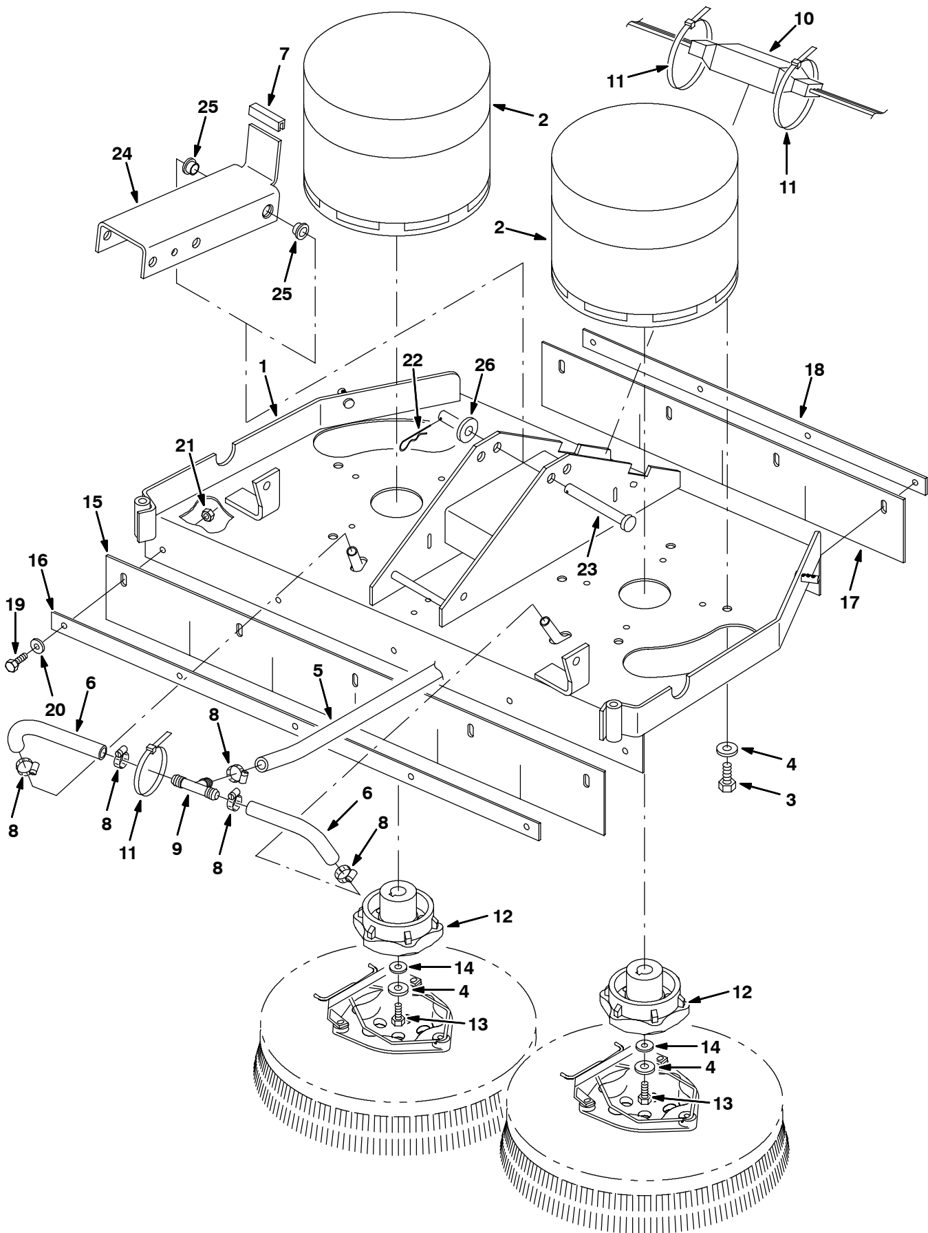
Fig. 26 - Rollout Battery Disk Scrub Head Drive Motor Group, 700 mm (28 in)
