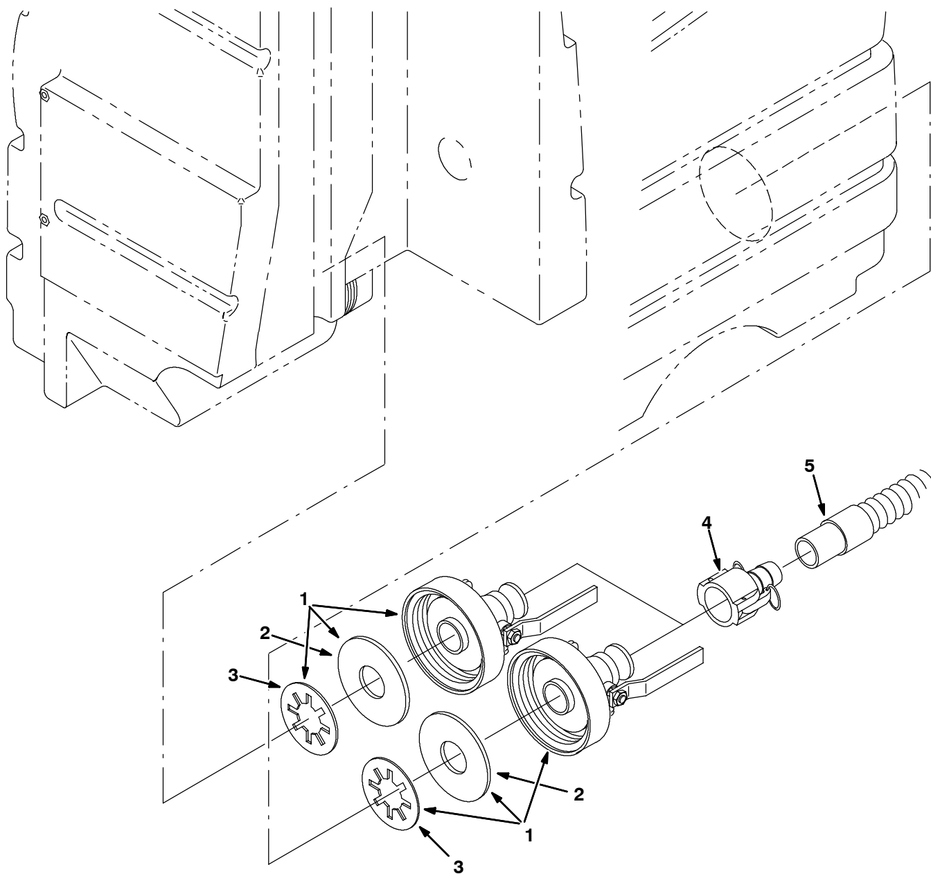
Fig. 46 - Positive Solution Control Drain Kit, ES™
