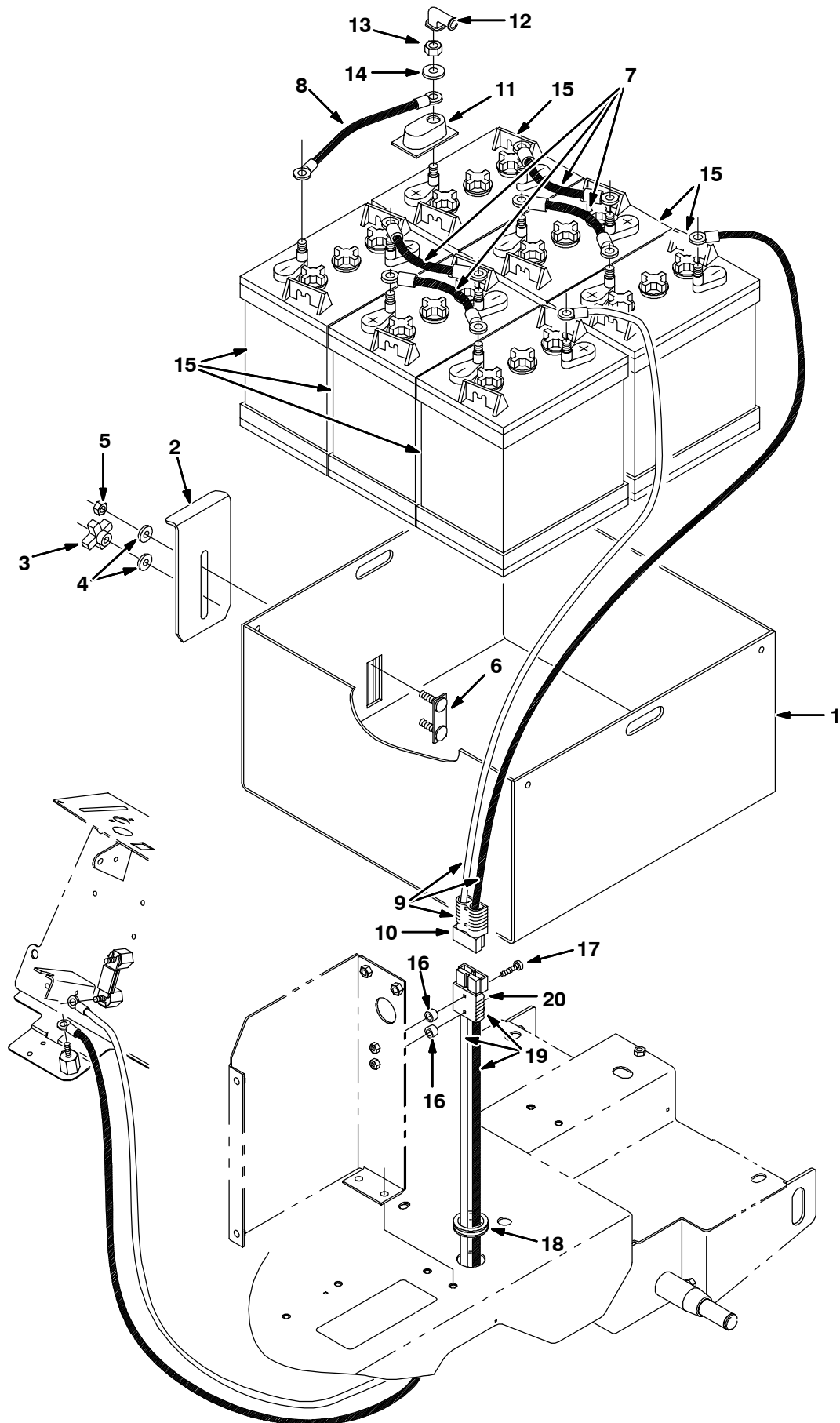
Fig. 35 - Rollout Battery Pack Kit
