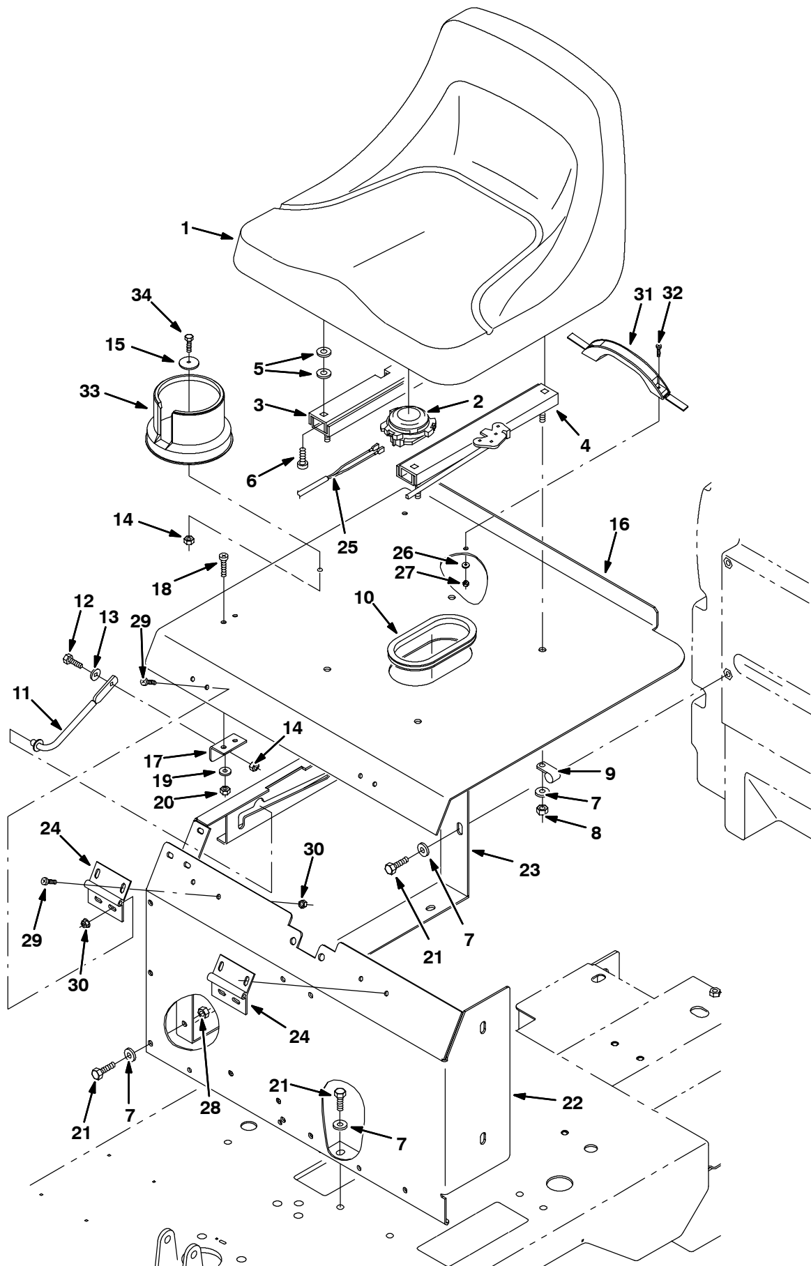
Fig. 6 - Seat Group (10108252- )
