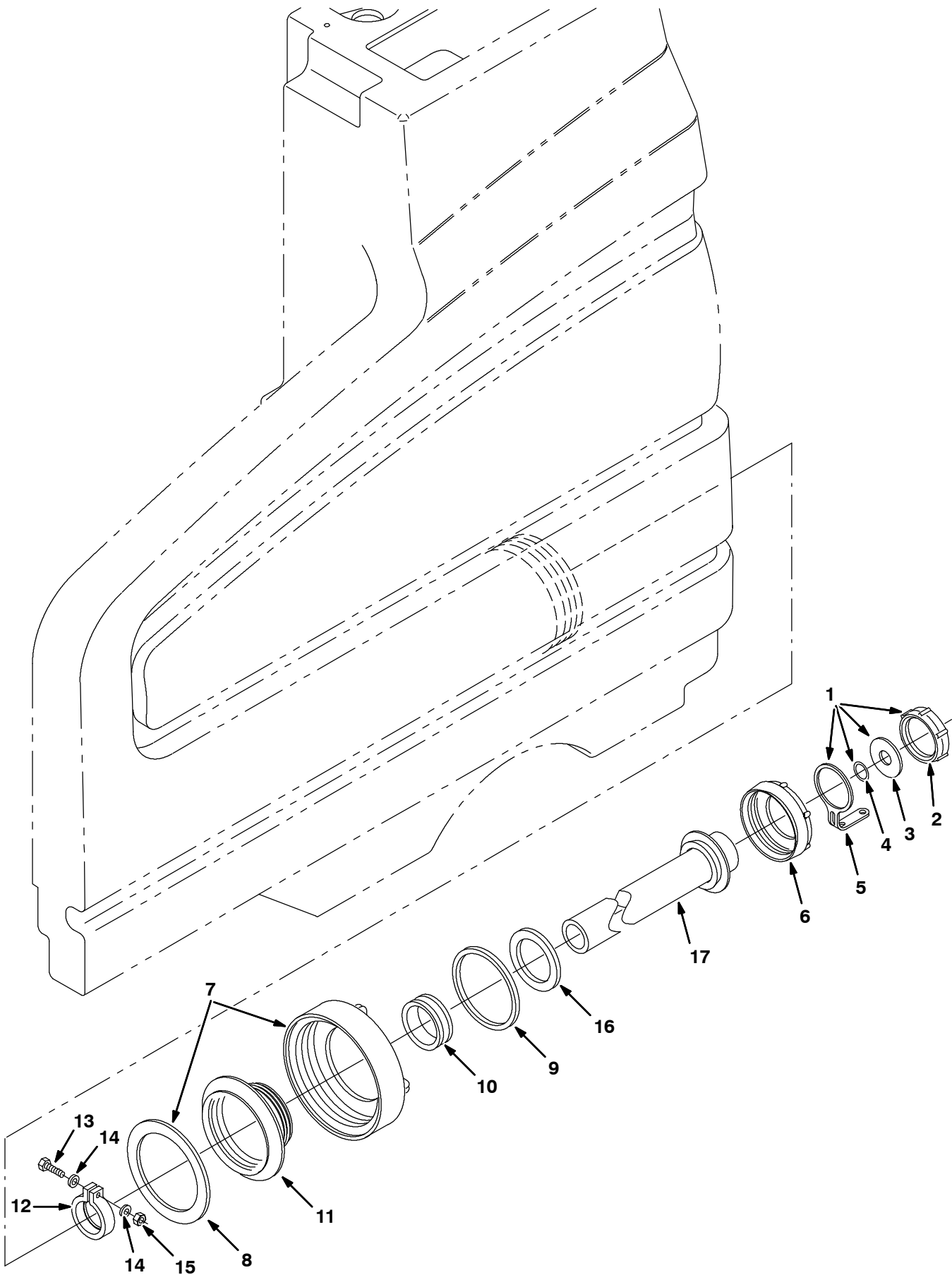
Fig. 3 - ES™ Drain Group
