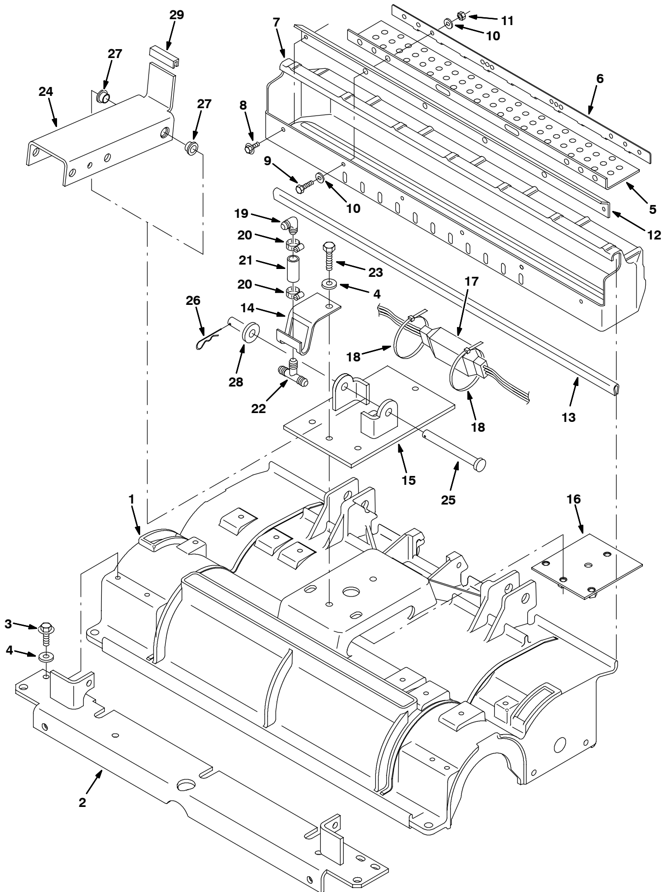
Fig. 30 - Rollout Battery Cylindrical Scrub Head Frame Group, 800 mm (32 in)
