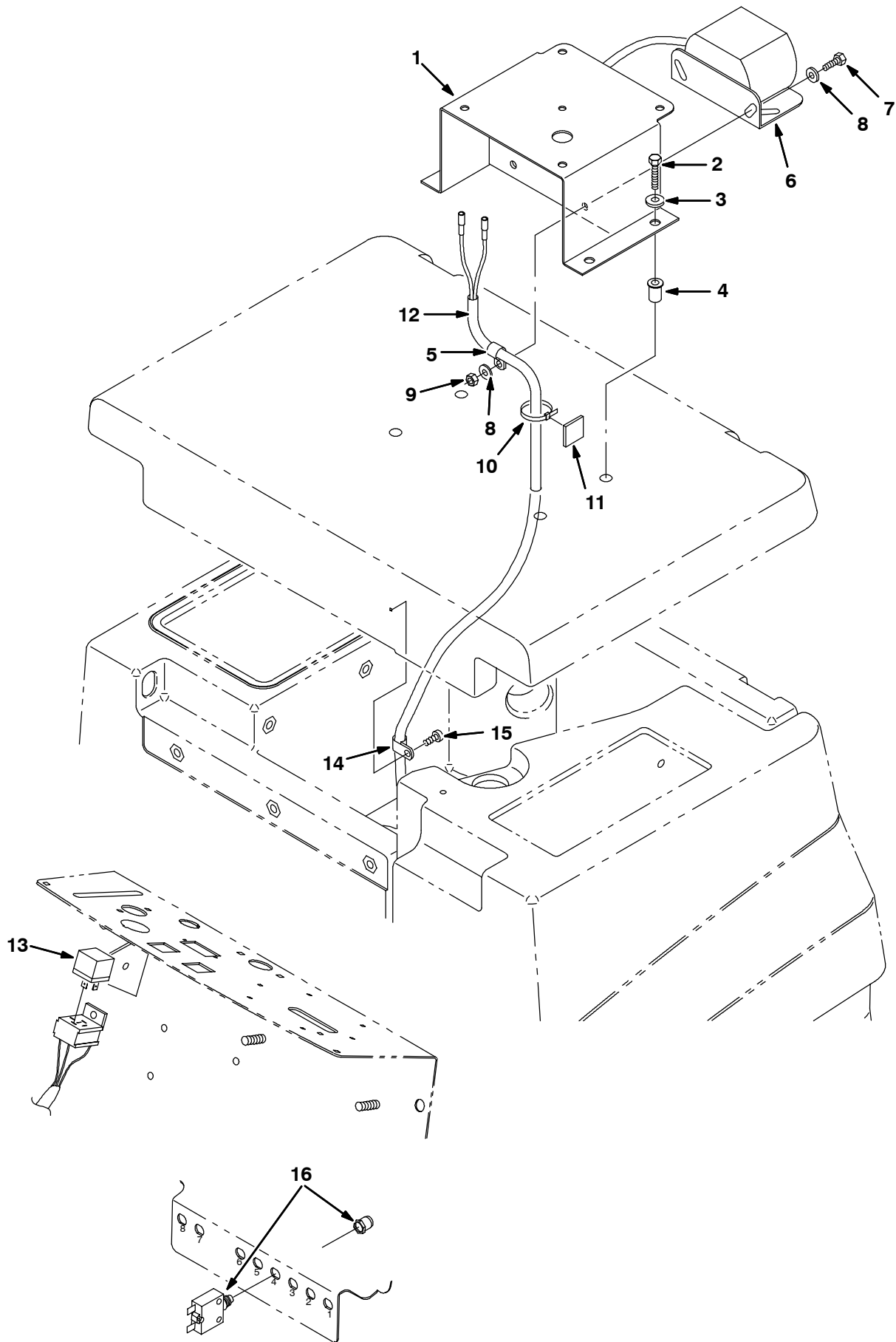
Fig. 44 - Backup Alarm Kit
