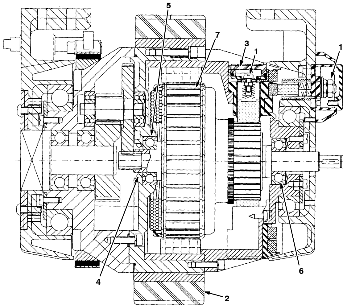
Fig. 6 - Front Wheel Gearbox Breakdown, 390850
