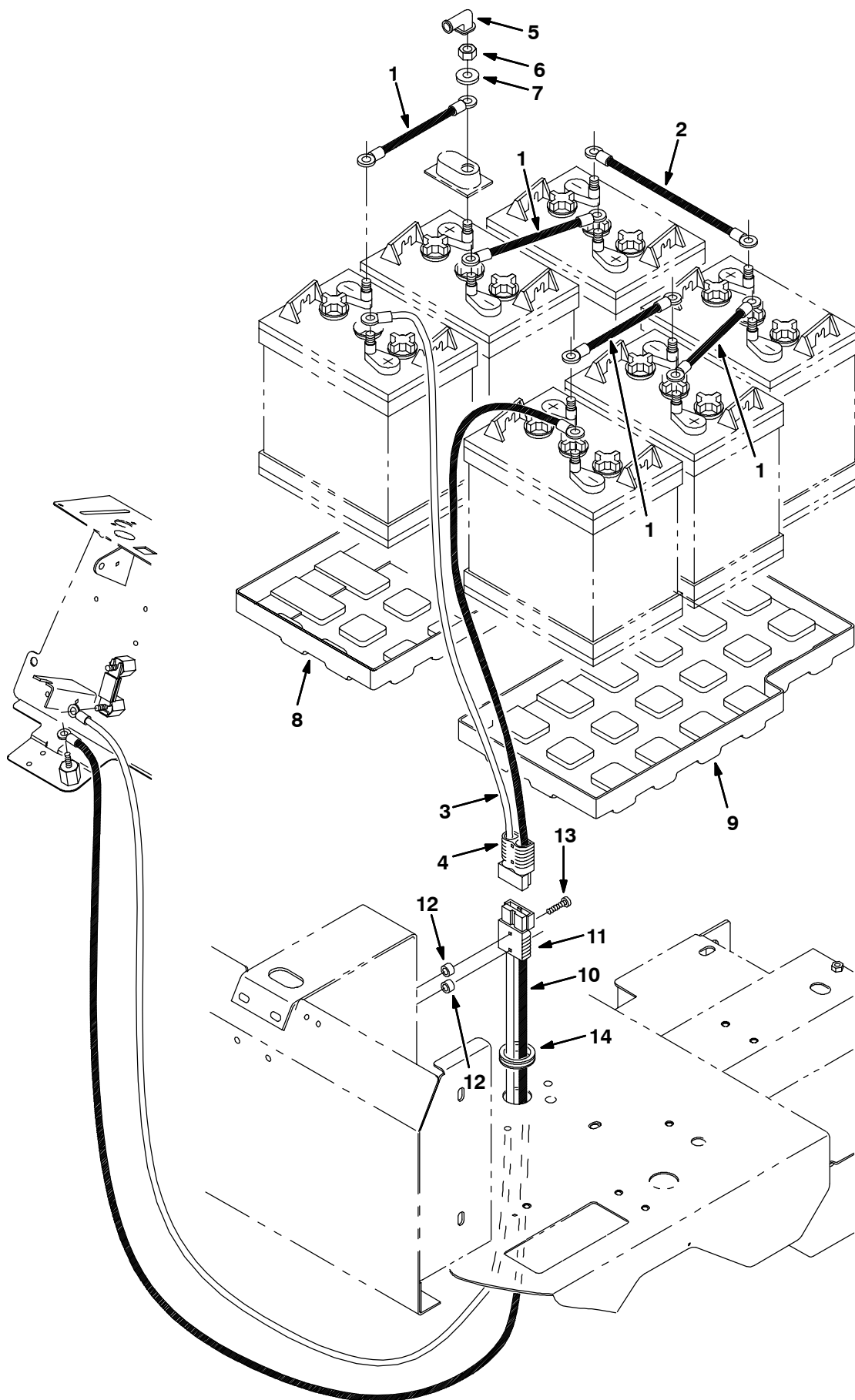
Fig. 25 - Battery Cable Group
