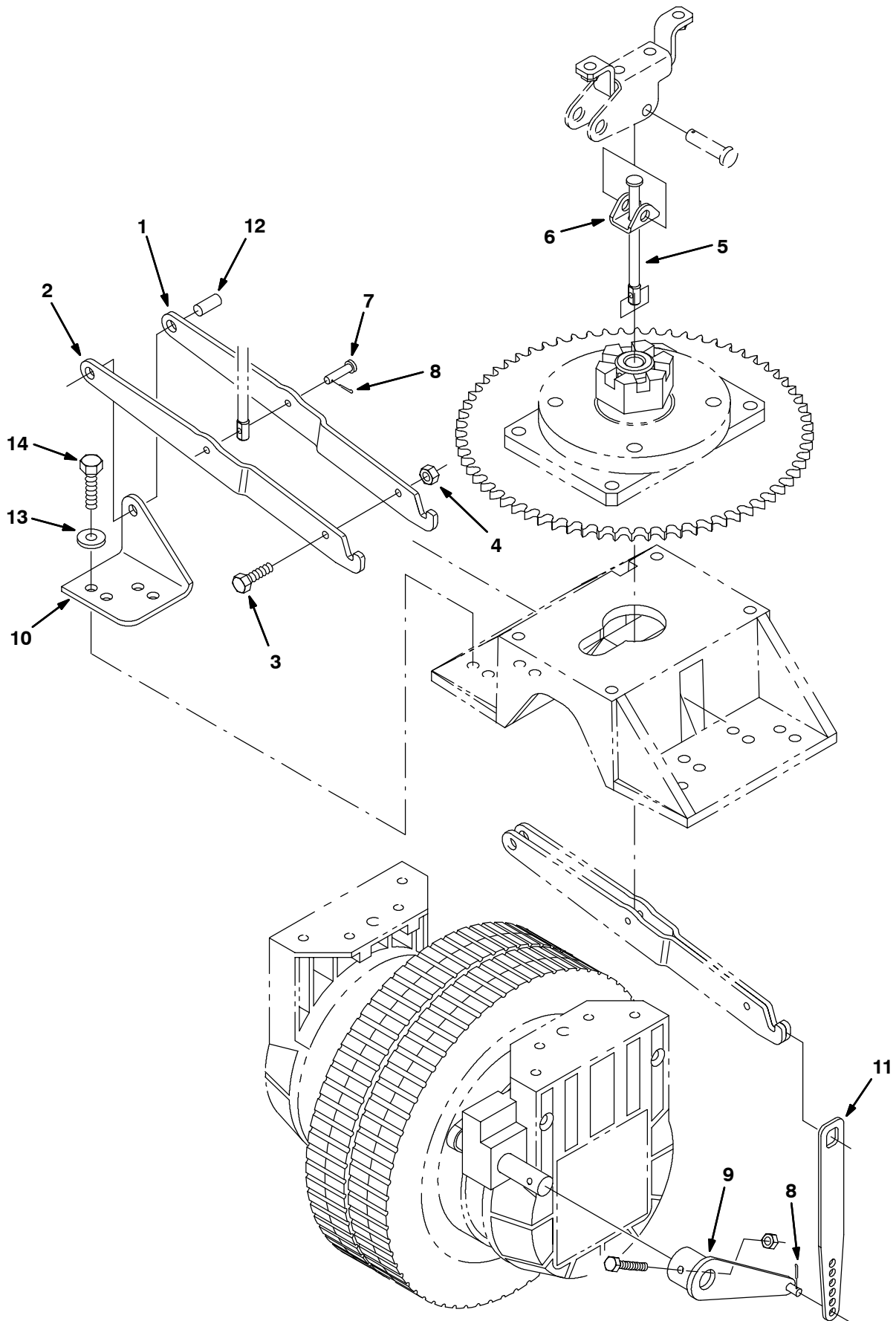
Fig. 13 - Front Brake Linkage Group (10160410- )
