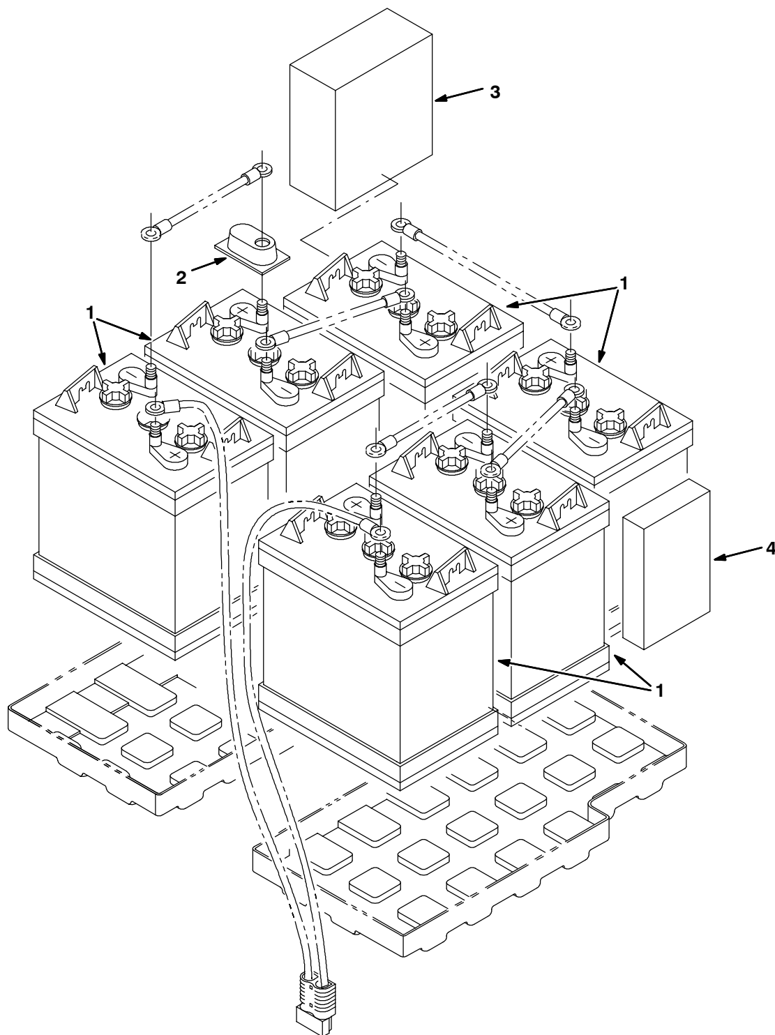
Fig. 38 - Battery Kit, Wet, 244AH
