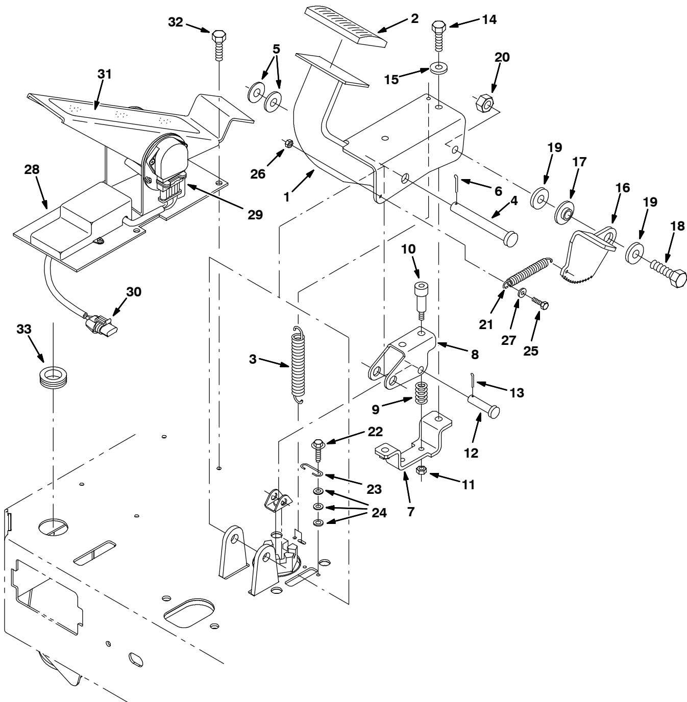
Fig. 14 - Brake Pedal and Directional Pedal Group
