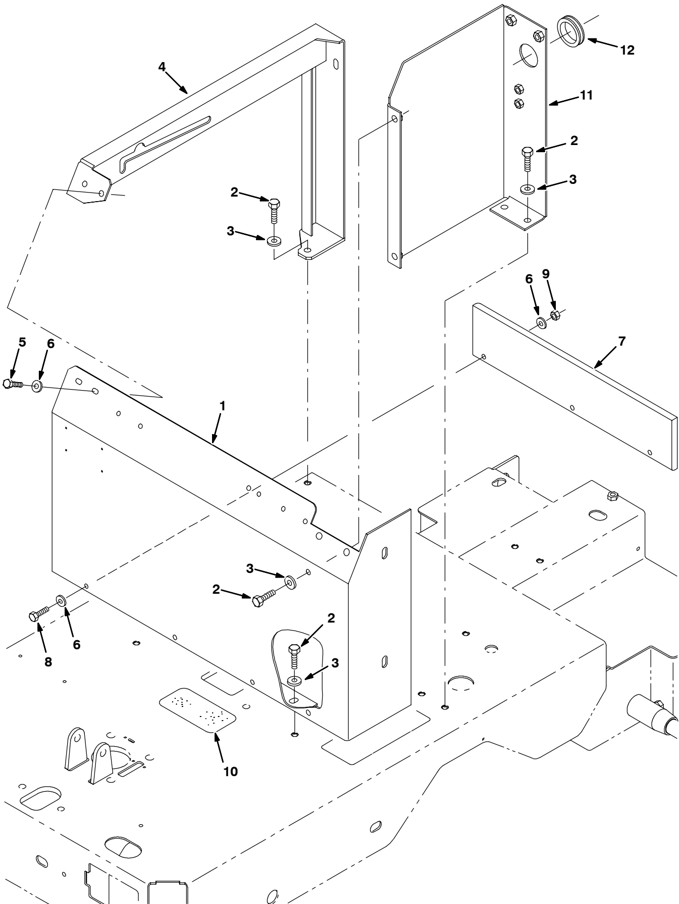
Fig. 33 - Rollout Battery Seat Support Group
