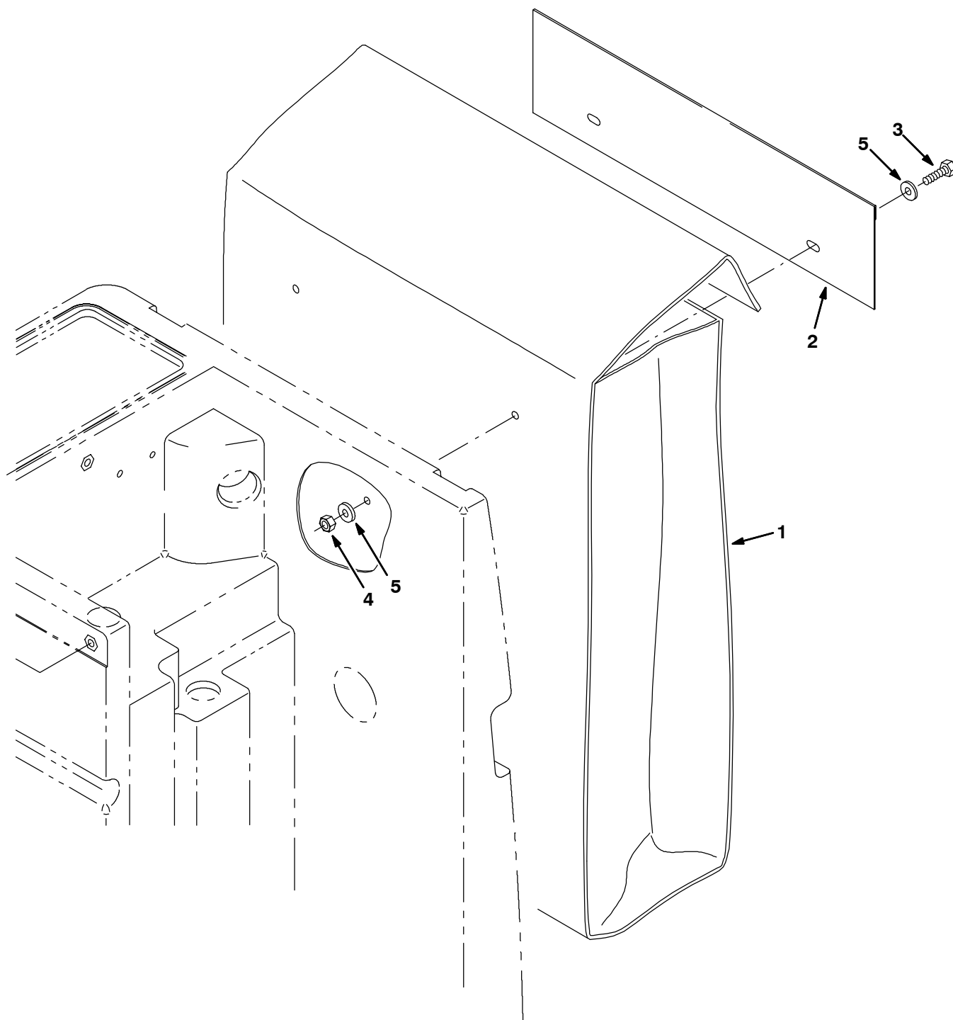
Fig. 48 - Storage Bag Kit
