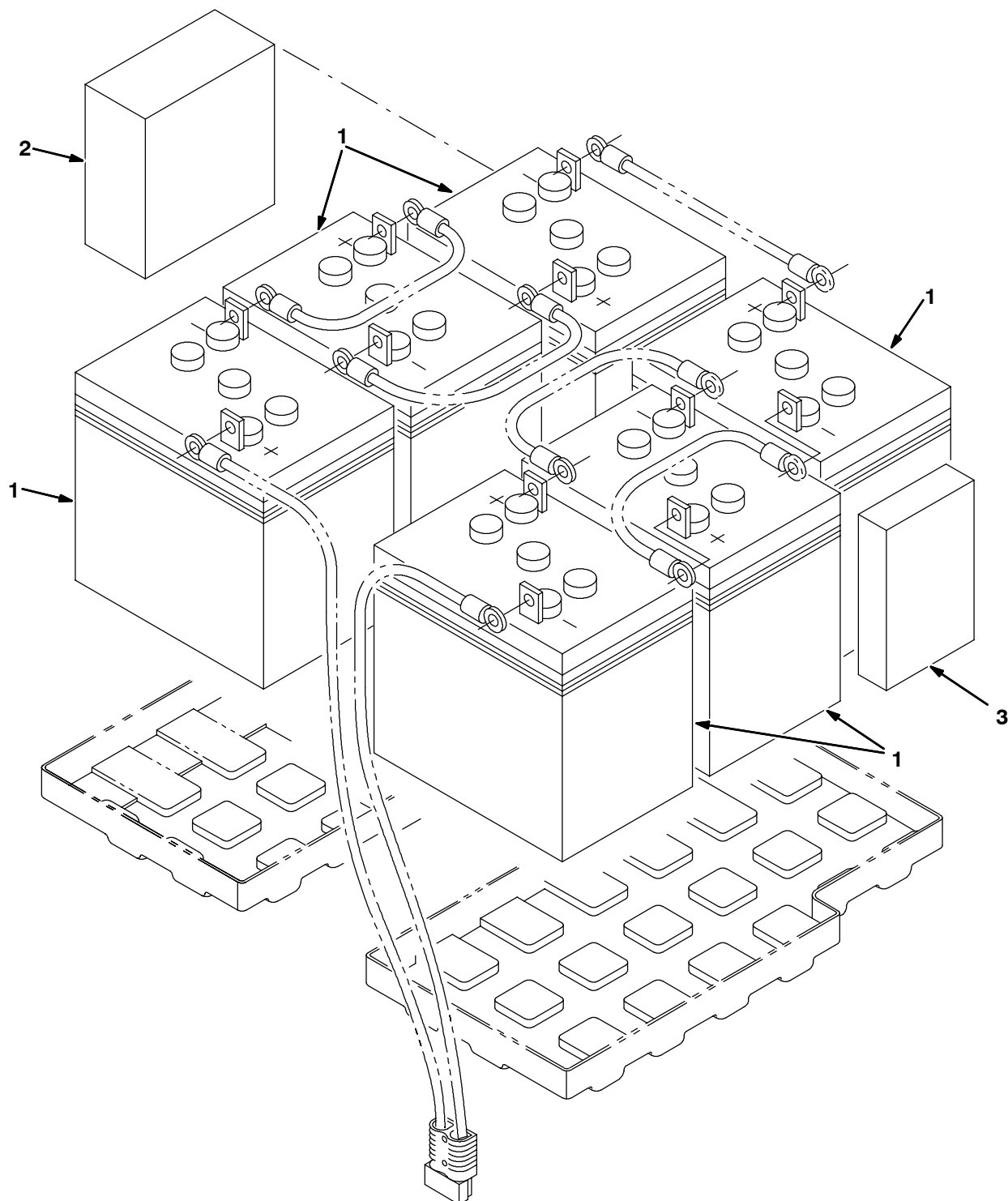
Fig. 39 - Battery Group, Maintenance Free, 180AH
