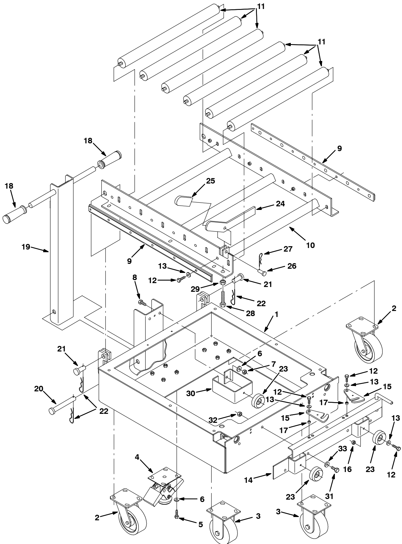
Fig. 36 - Rollout Battery Cart Kit
