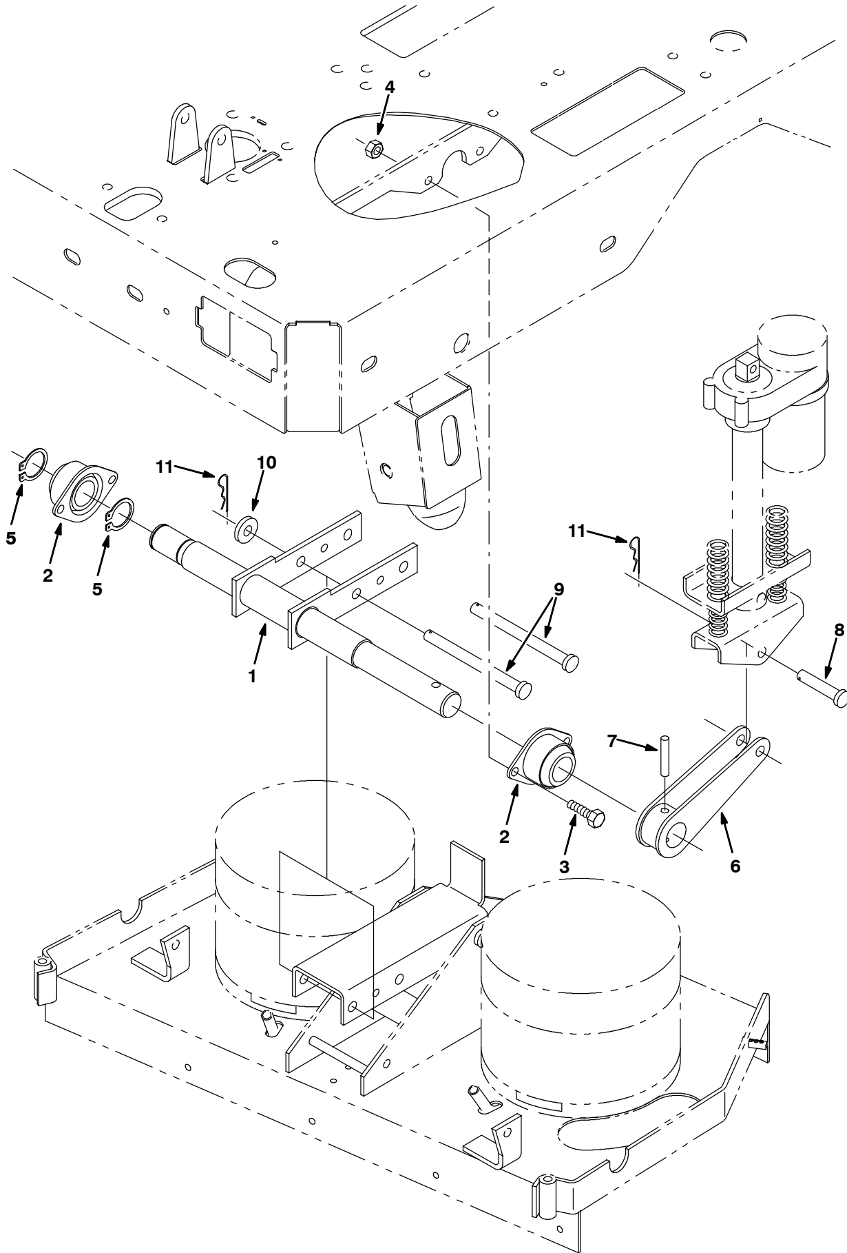
Fig. 34 - Rollout Battery Scrub Head Lift Group
