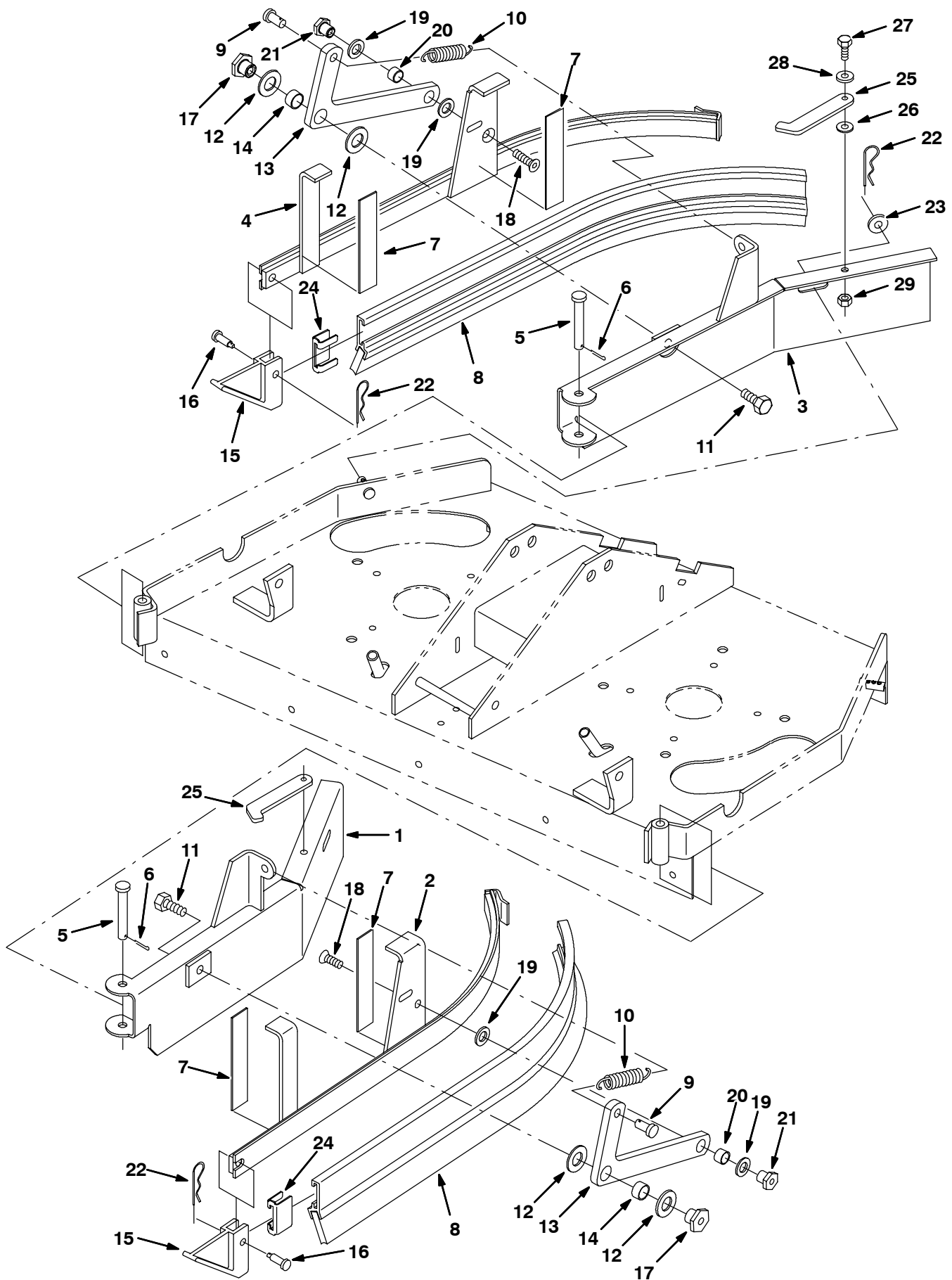
Fig. 27 - Rollout Battery Disk Scrub Head Squeegee Group, 700 mm (28 in)
