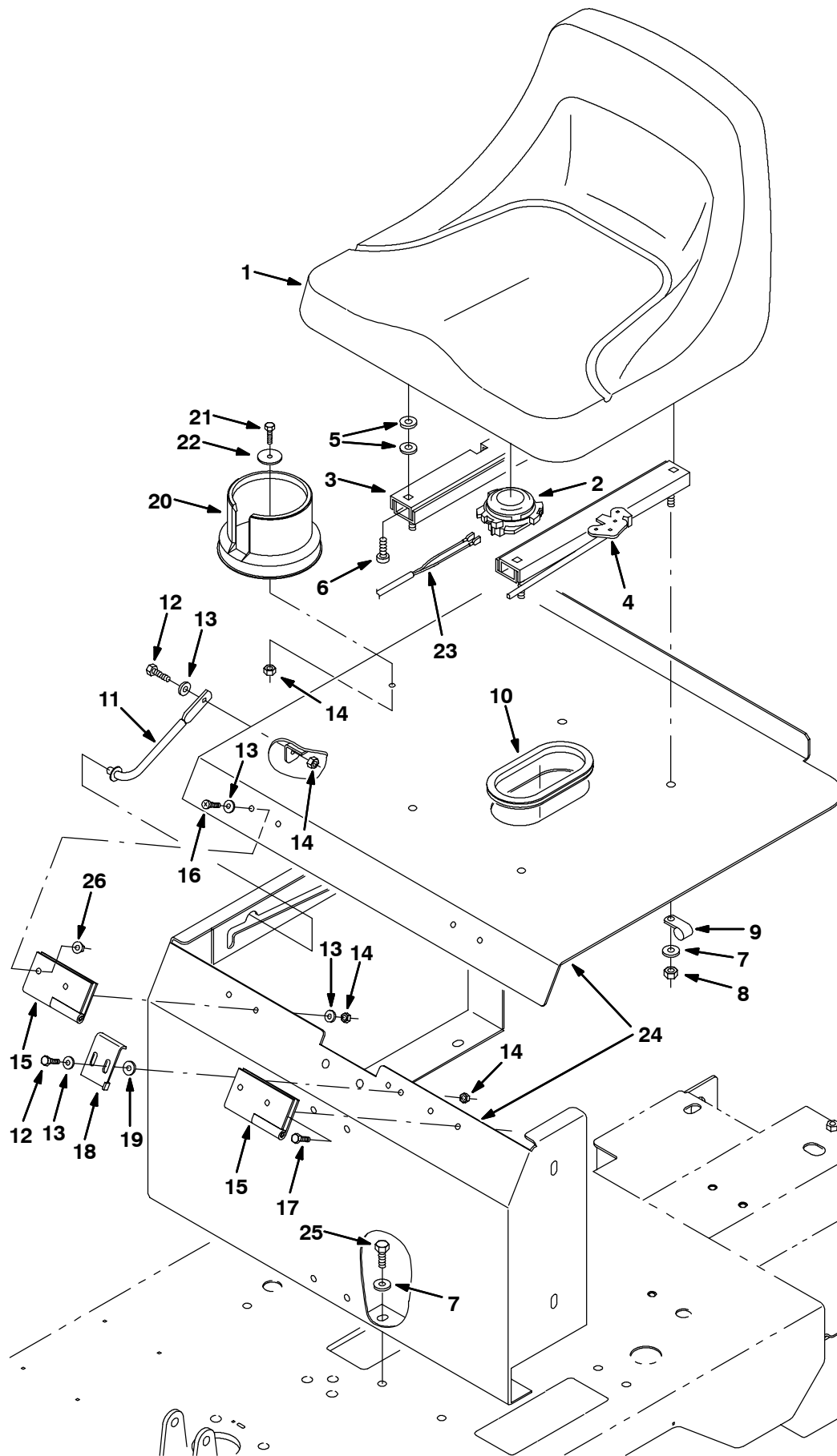
Fig. 5 - Seat Group (0000000-10108251)
