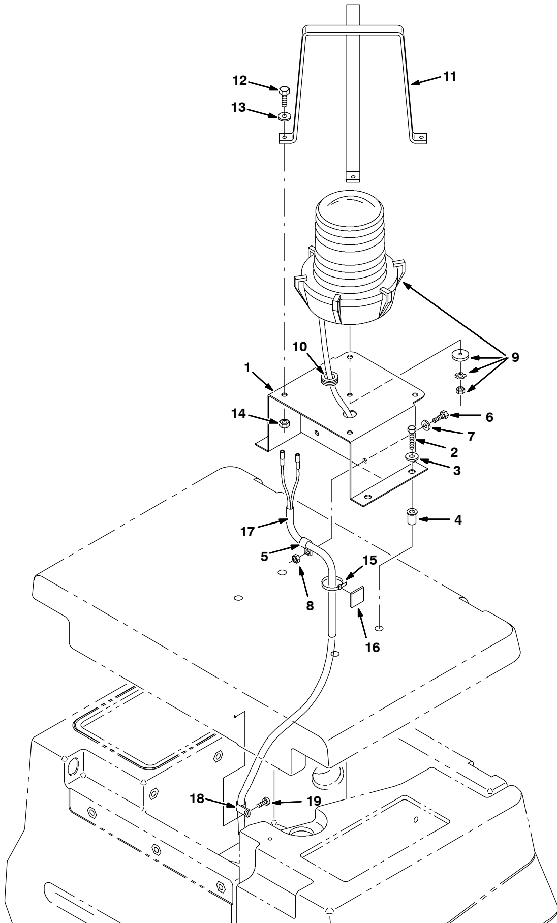
Fig. 43 - Flashing Light Kit
