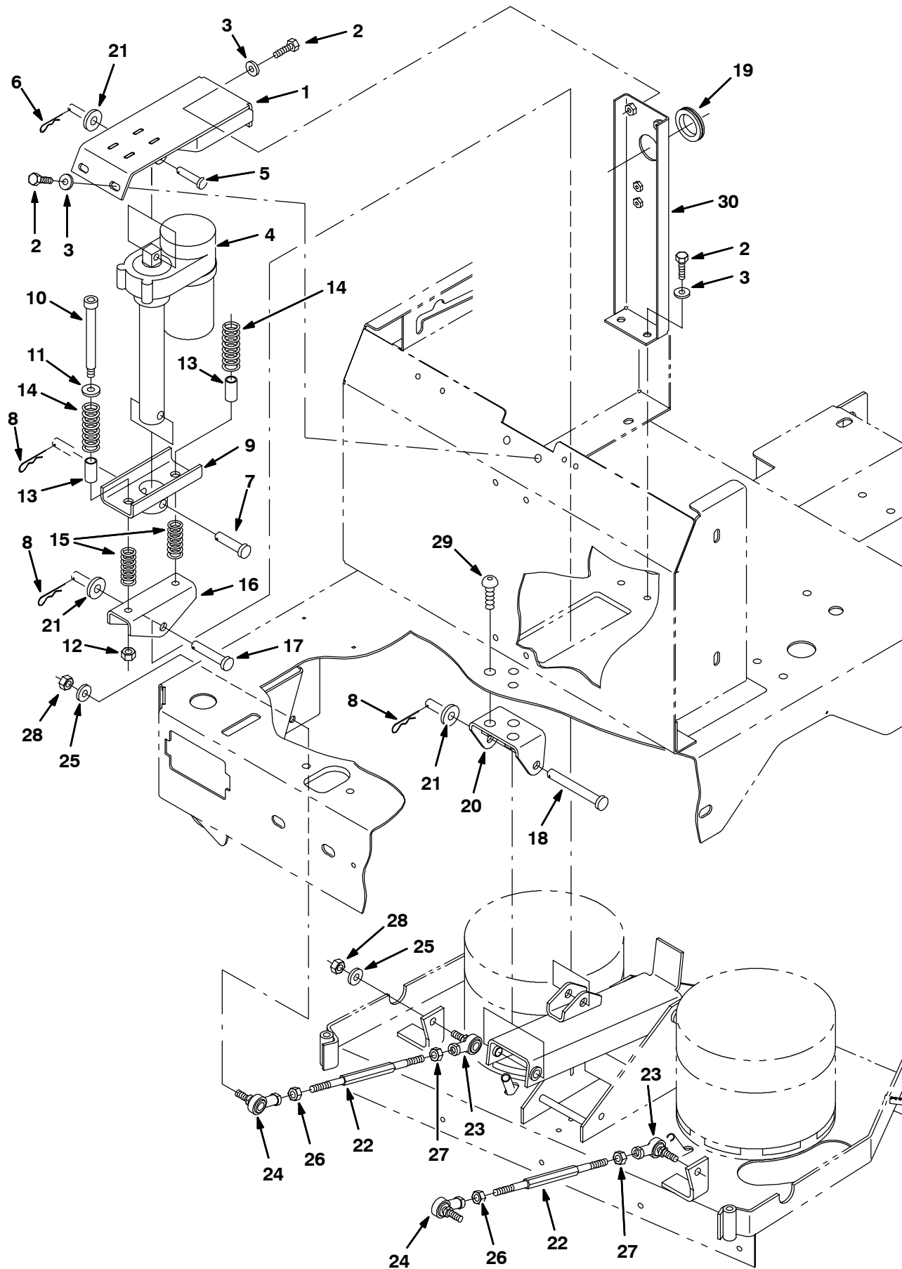
Fig. 17 - Scrub Head Lift Group
