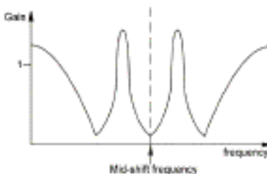
Responses of a phaser with high resonance
