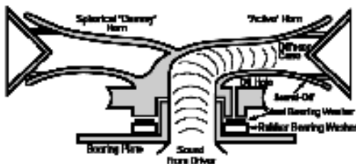
Upper speaker assembly
