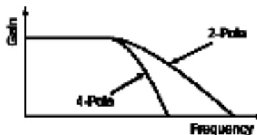
The 2/4 pole switch selects the filter slope
