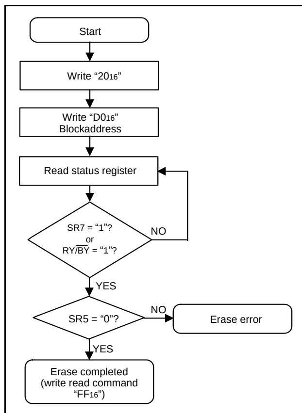
Fig 73. Erase flowchart
