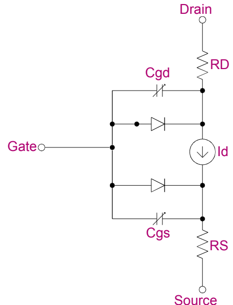
JFET Model
