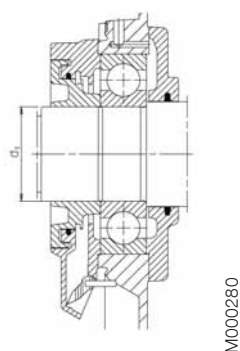
Labyrinth seal
