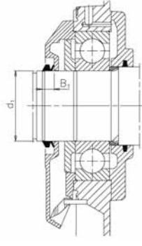
V-ring
