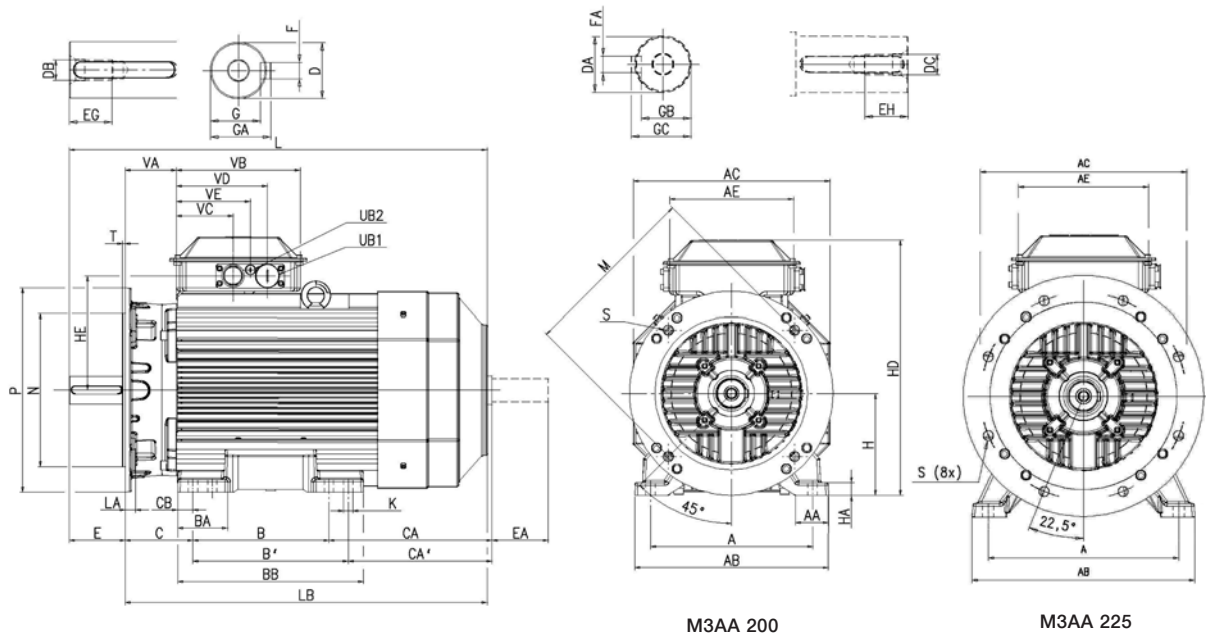
M3AA 200
