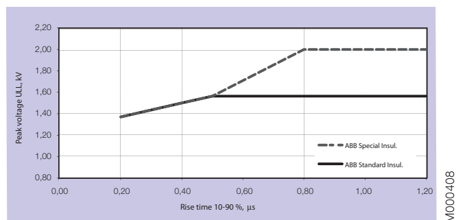
Figure 1 The maximum allowed phase-to-phase voltage peaks at the motors terminals, as a function of the pulse rise time
