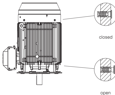
Motor sizes 160-450 As standard with drain holes and closable plugs.
