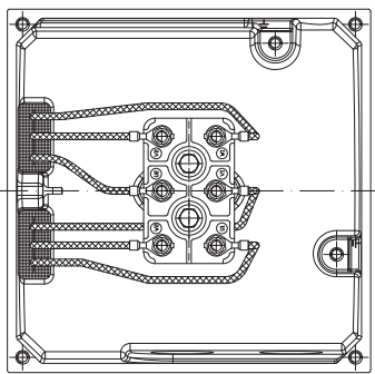
Terminal board for motor sizes 132
