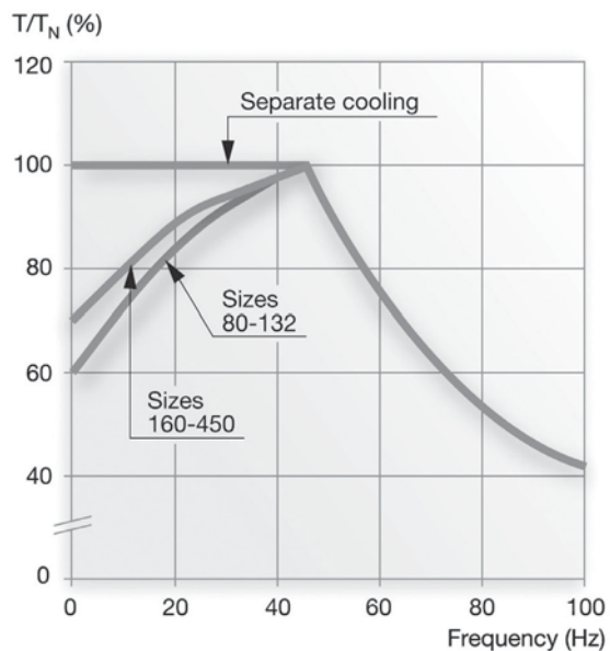
Figure 3. Loadability curves with ACS550 converters with vector control
