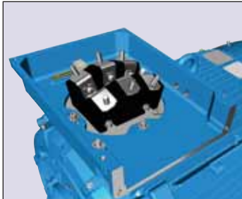
Fig 6. Terminal board for motor sizes 280-315.
