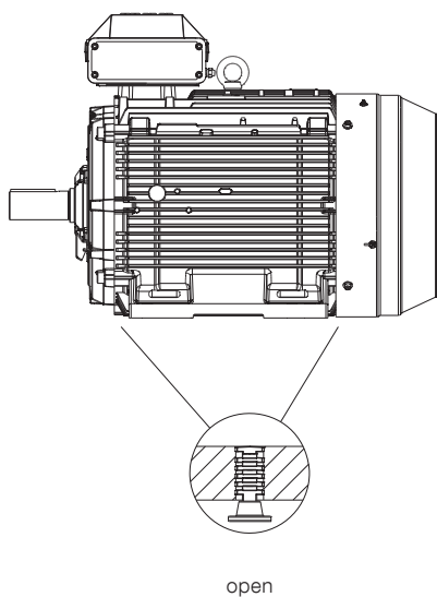
Motor sizes 160-450 As standard with drain holes and closable plugs.
