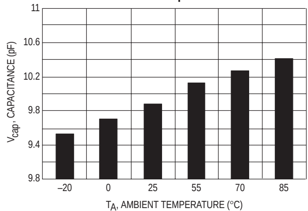
Figure 36. Varicap Value at V_{CV} = 1.0 V Over Temperature
