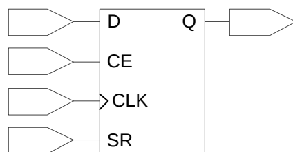
Figure 3-14 Register Structure in I/O Logic
