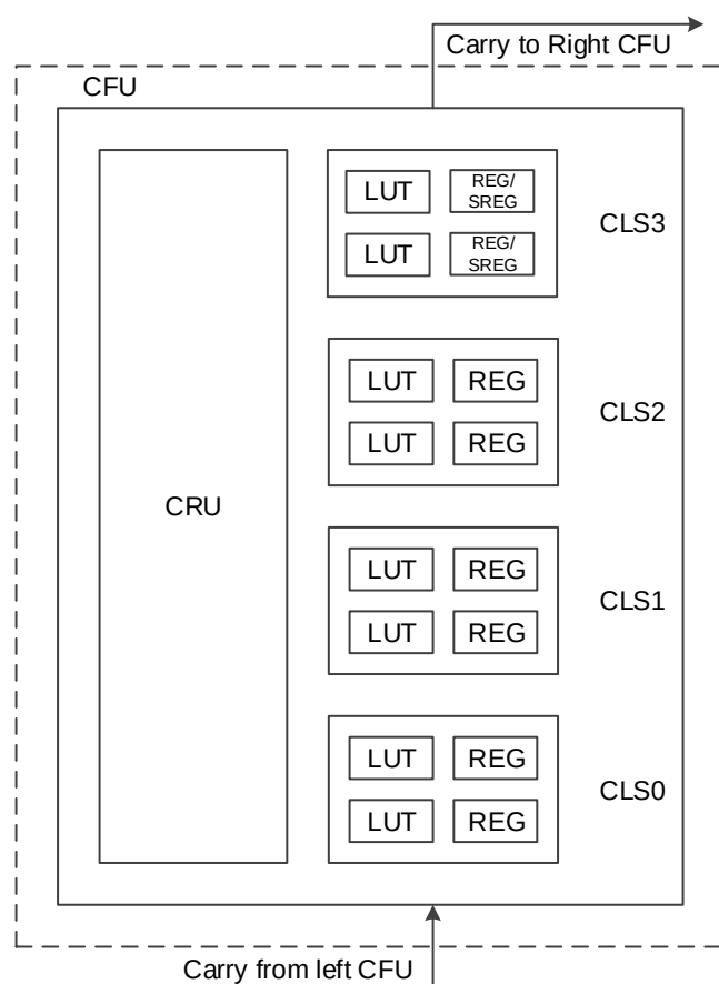
Figure 3-5 CFU View
