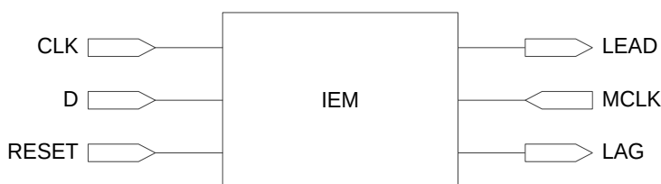
Figure 3-15 IEM Structure
