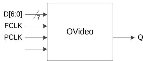
Figure 3-23 I/O Logic in OVideo Mode
