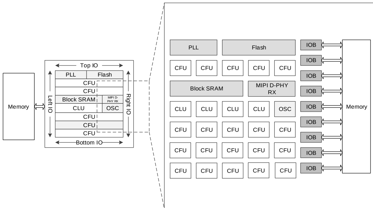
Figure 3-4 GW1NR-2 Architecture Overview
