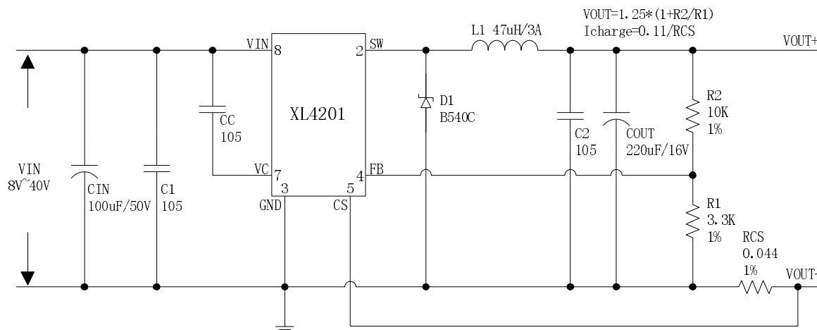
Figure5. XL4201 System Parameters Test Circuit (VIN=8V~36V, VOUT=5V/0.1A~2.5A)
