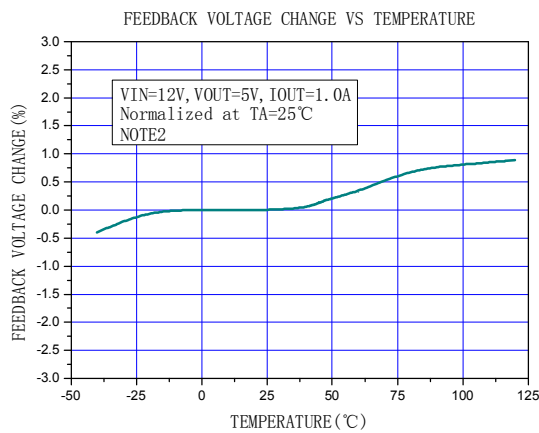
Figure10. Feedback voltage change Curve
