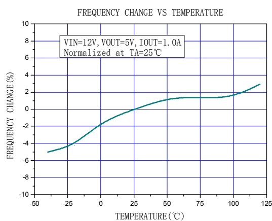
Figure9. Frequency change Curve
